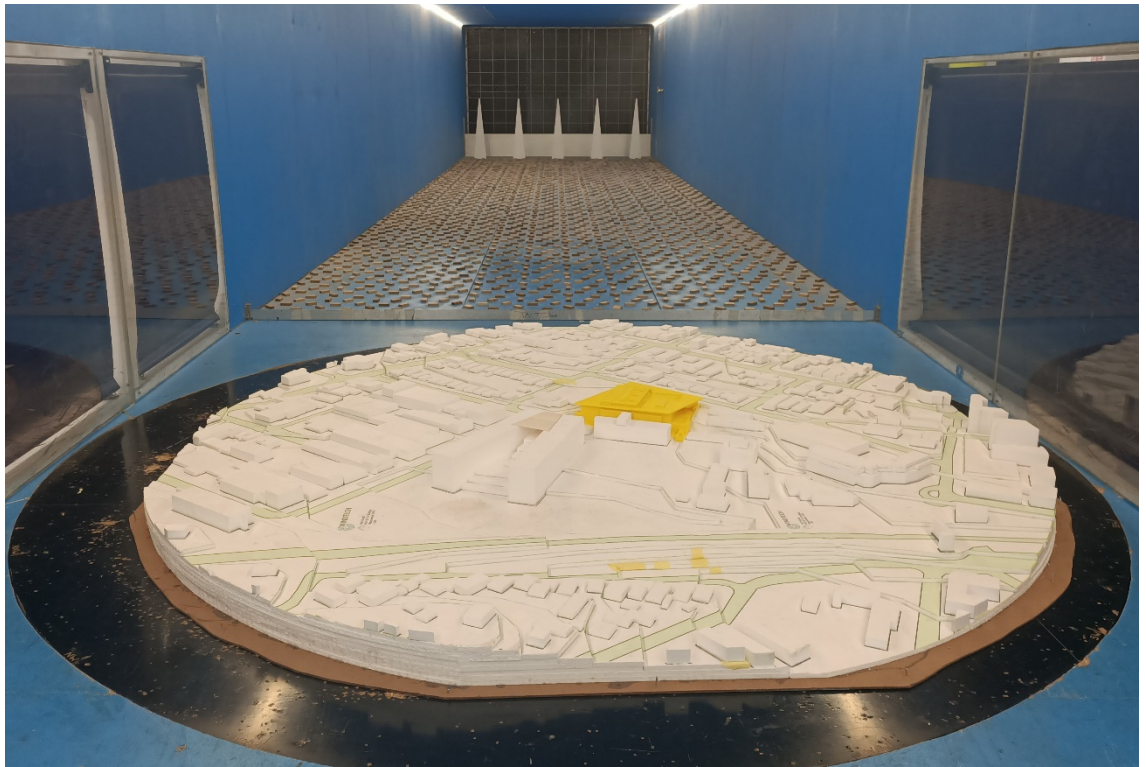
Figure 1b: Photograph of the Wind Tunnel Model – Proposed Scenario (view from the west)
