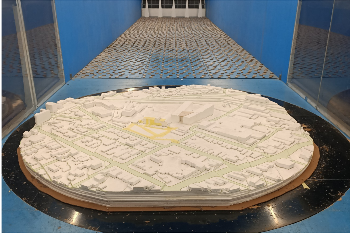
Figure 1f: Photograph of the Wind Tunnel Model – Existing Scenario (view from the east)
