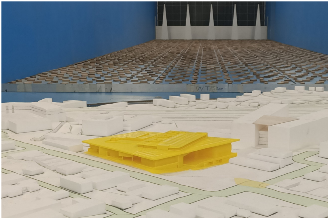
Figure 1e: Photograph of the Wind Tunnel Model – Proposed Scenario (view from the east)
