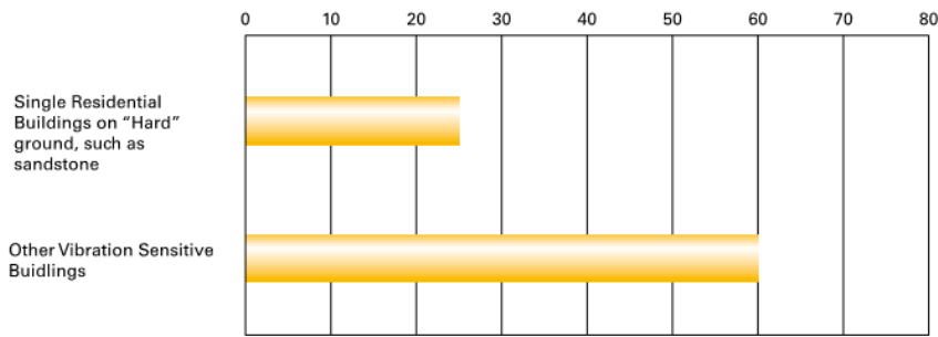
Figure 6: Vibration Assessment Zones based on distance (m) of vibration sensitive development from rail corridor
