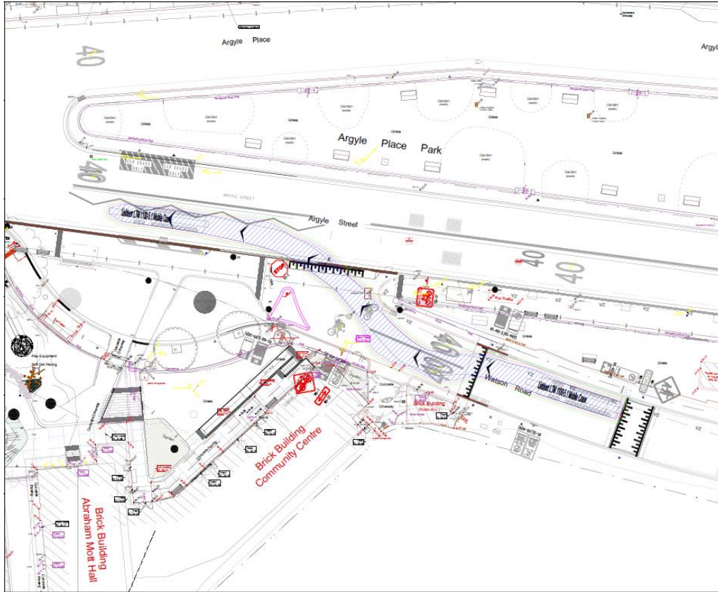
Figure 13: Mobile crane exit from Watson Road to Argyle Street
