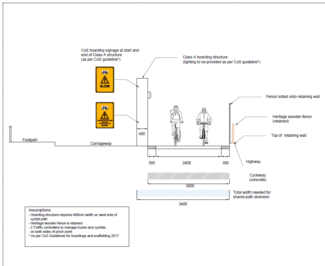
Figure 7: SHB shared path diversion hoarding structure
