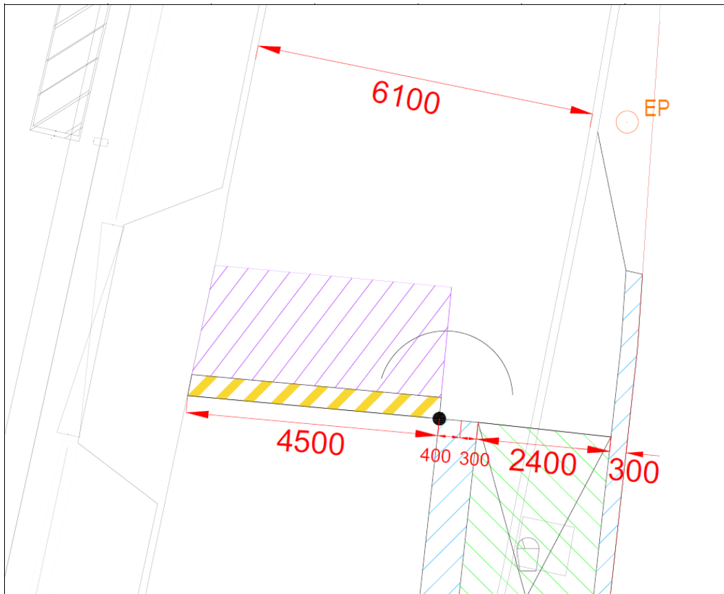
Figure 15: Dimensioned plan view of construction gate line and SHB shared path diversion
