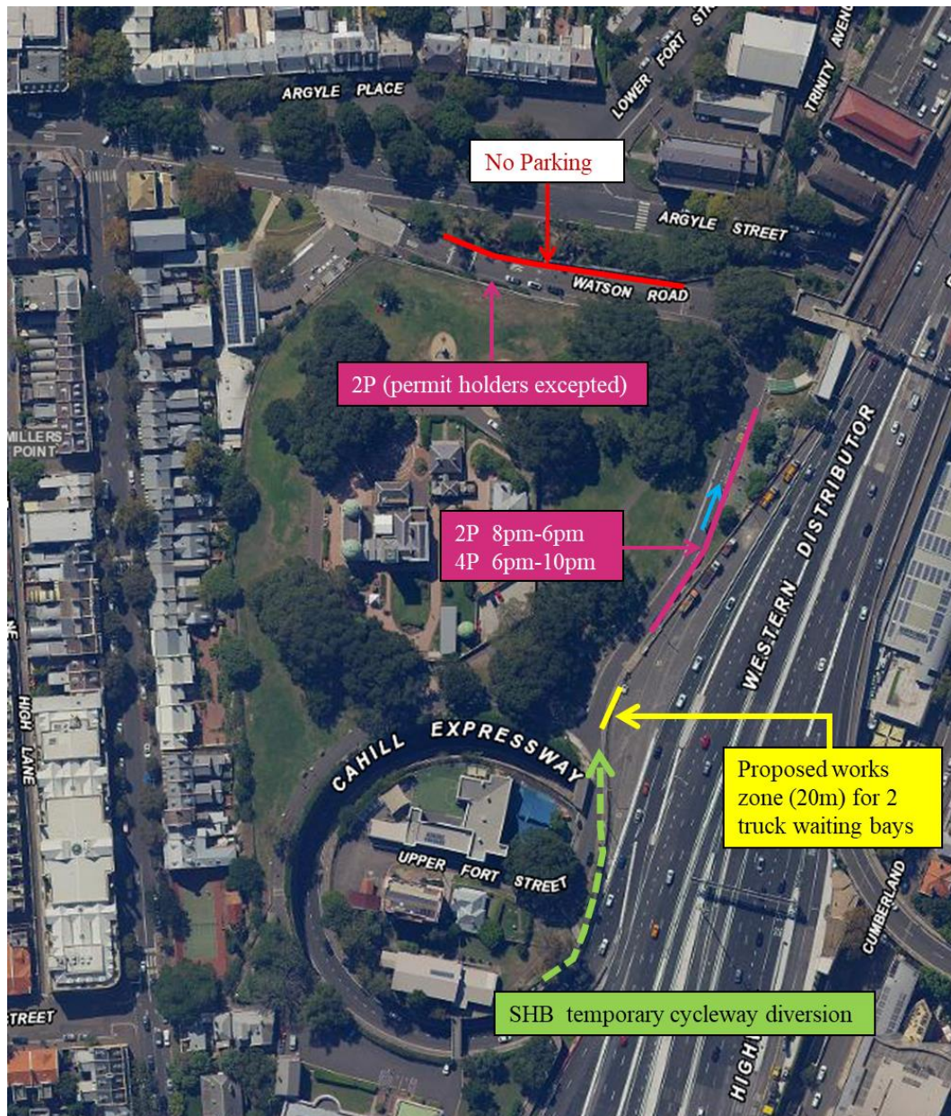
Figure 9: Proposed works zone
