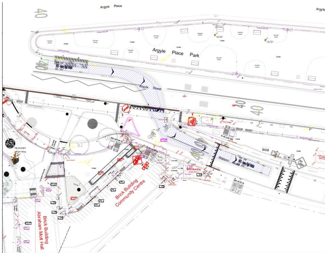
Figure 10: HRV entry path from Argyle Street into Watson Road
