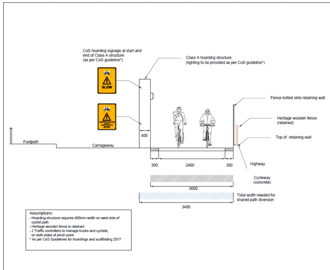
Figure 16: SHB shared path diversion cross section
