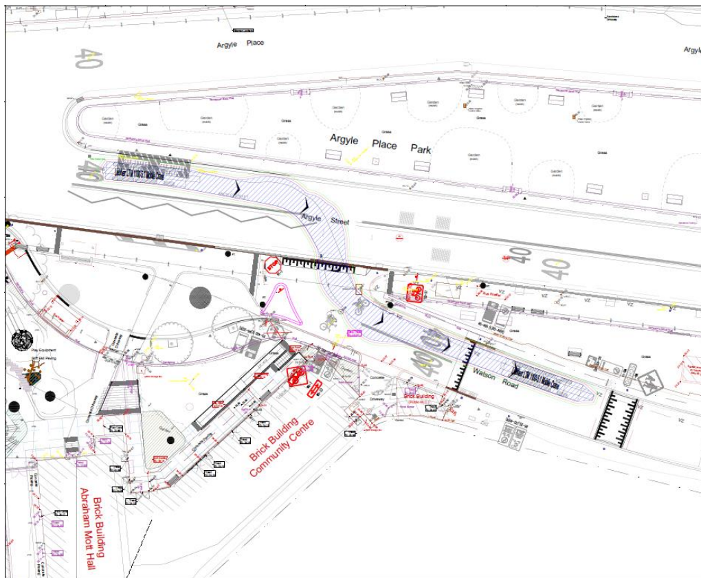
Figure 12: Mobile crane entry from Argyle Street into Watson Road
