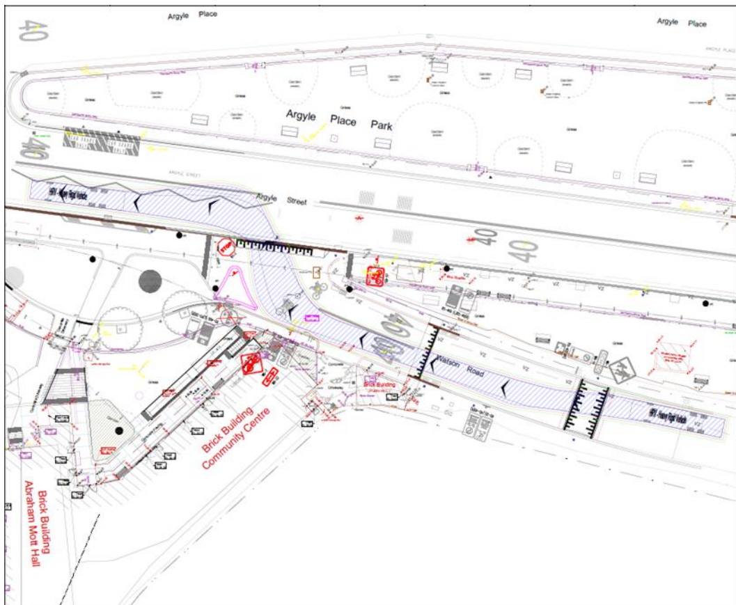
Figure 11: HRV exit from Watson Road to Argyle Street
