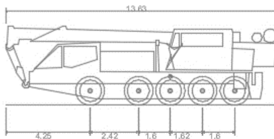
Figure 2: HRV vehicle dimensions
