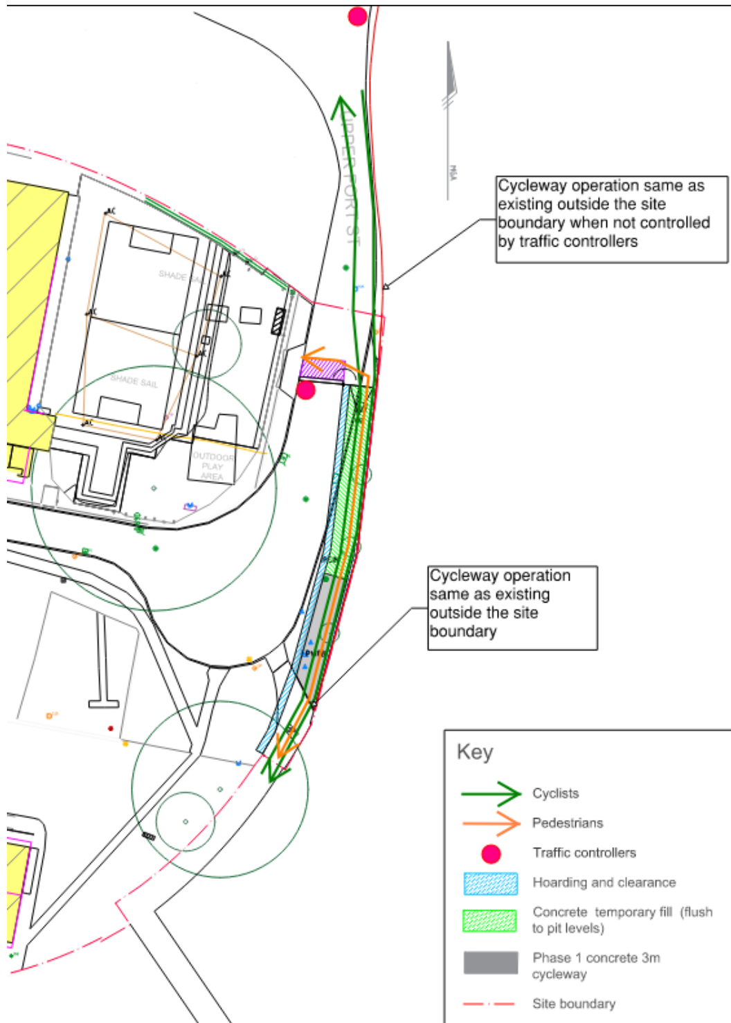
Figure 17: Operation of SHB shared path diversion
