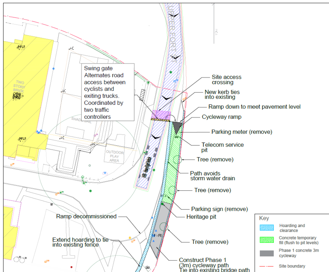
Figure 14: SHB Phase 1 and SHB shared path diversion
