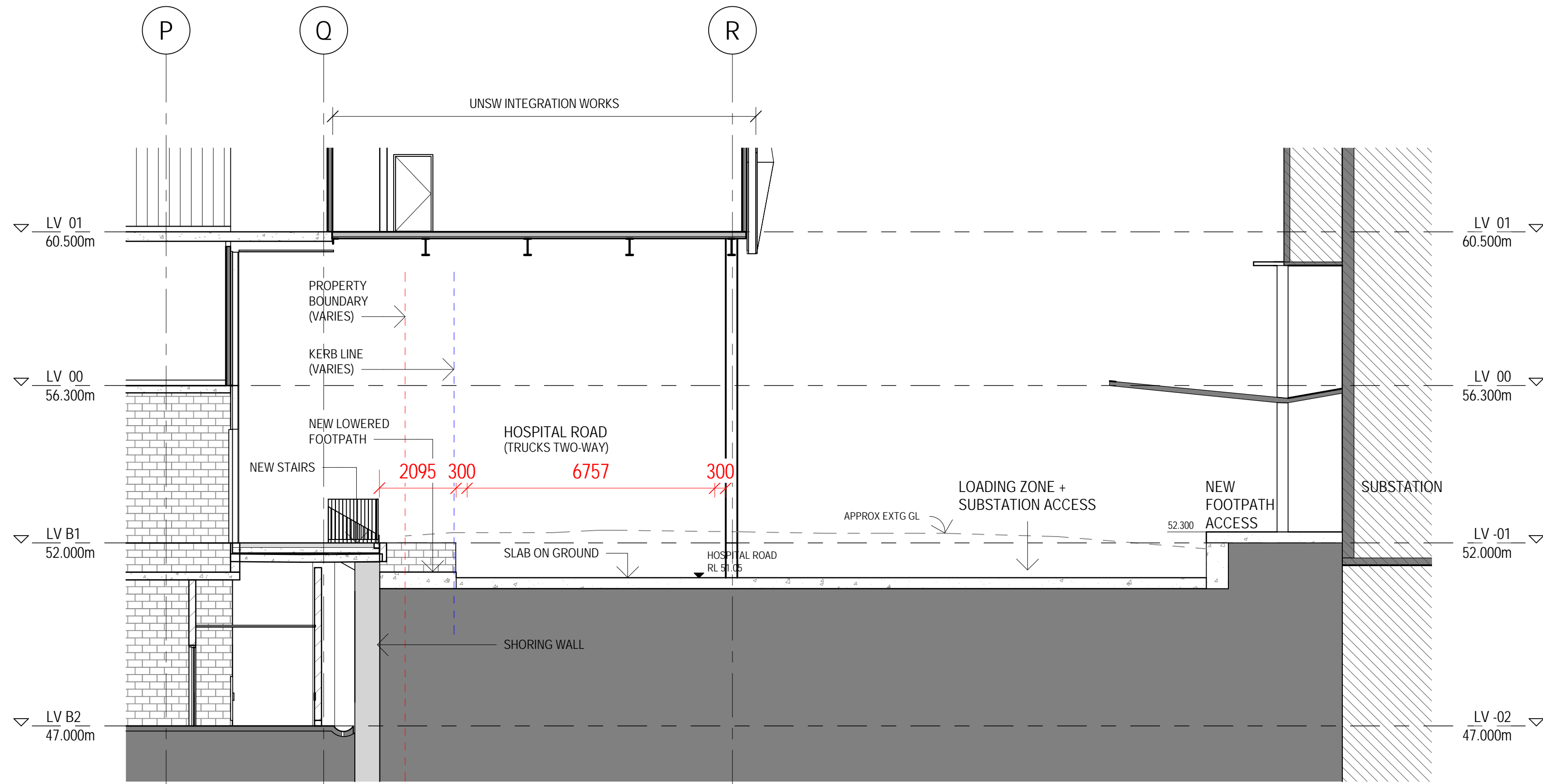
1 HOSPITAL ROAD - SECTION WOMEN'S HOSPITAL LOADING DOCK 1 : 100
