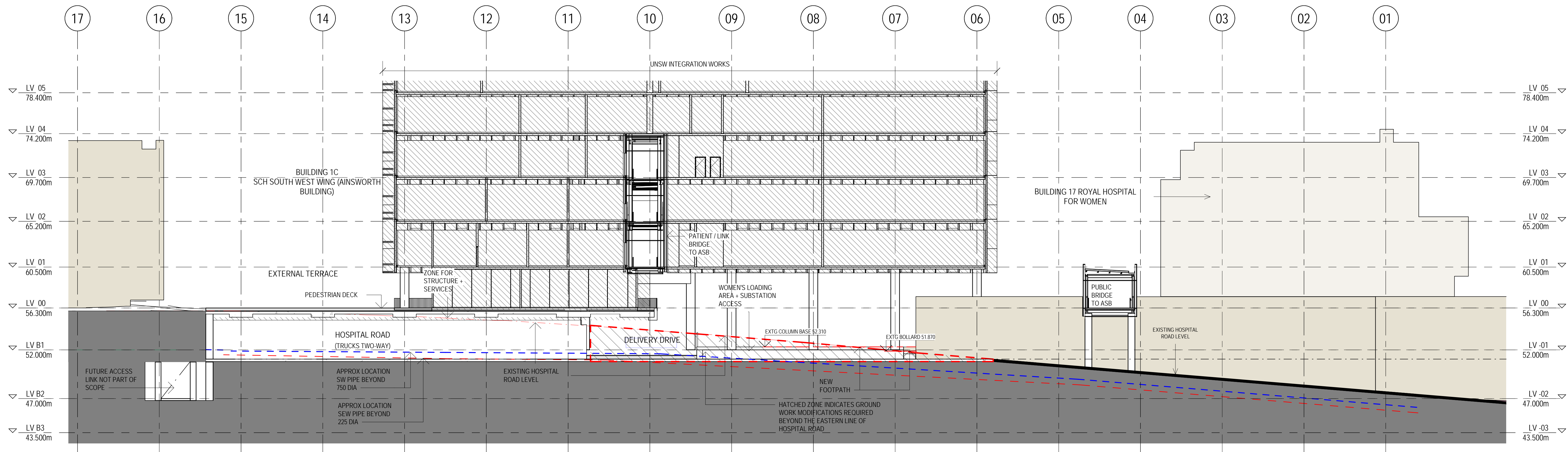
1 HOSPITAL ROAD - LONG SECTION_LOOKING EAST 108-B100001 1 : 200
