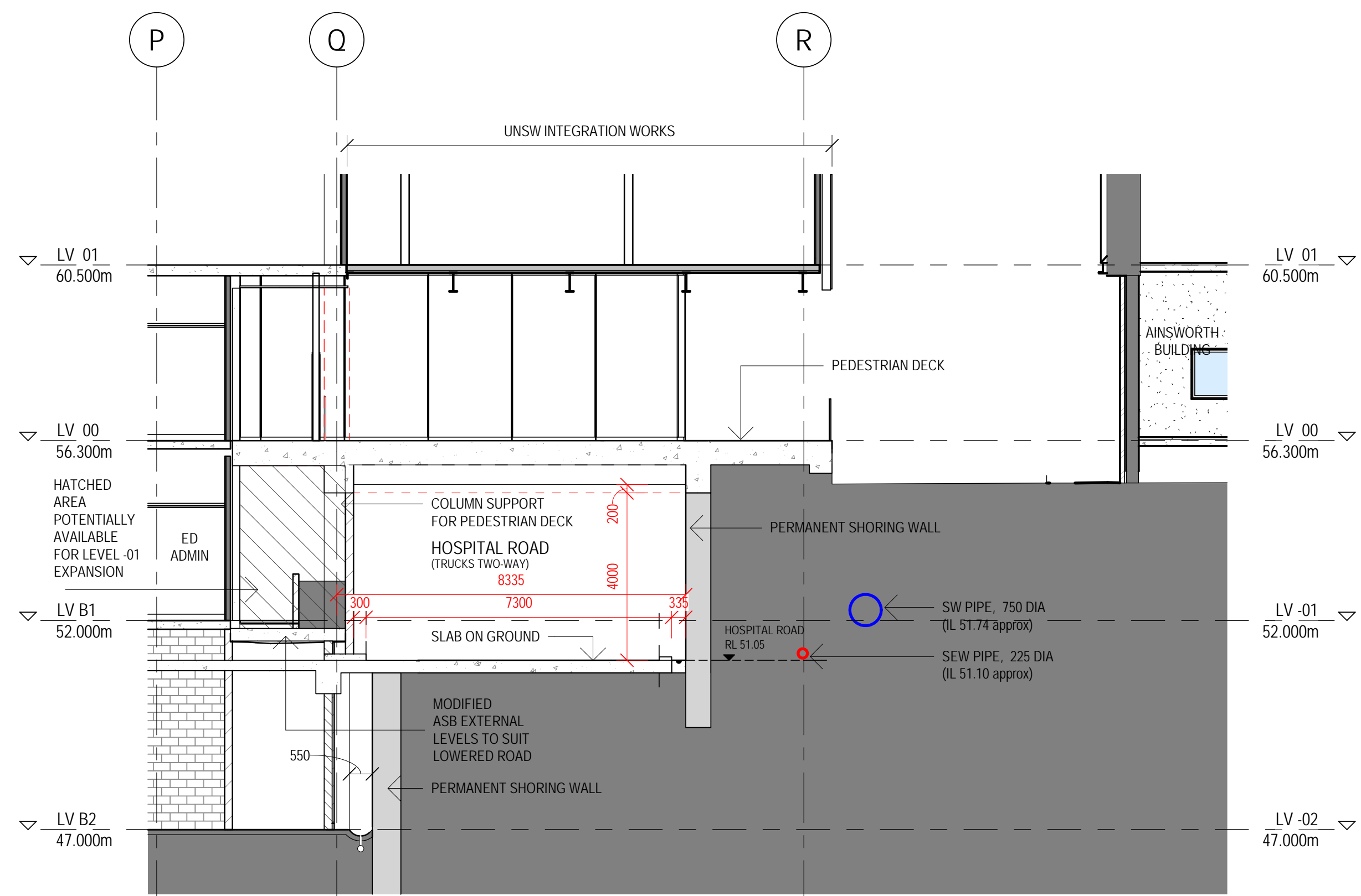
2 HOSPITAL ROAD - SECTION AINSWORTH 1 : 100
