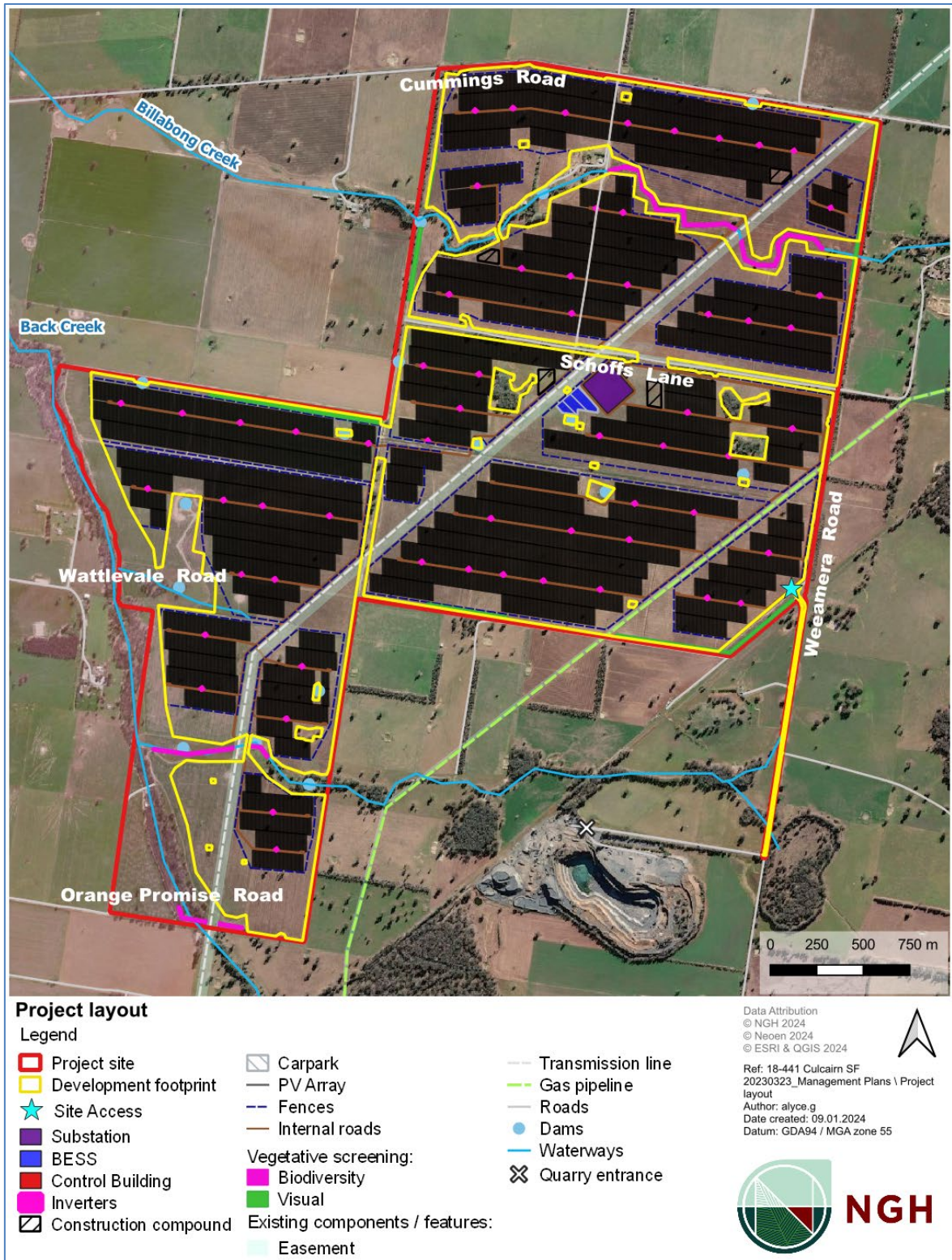
Figure 1: Approved Project Layout, as amended by Modification 1 of the Development Consent dated 22 December 2023
