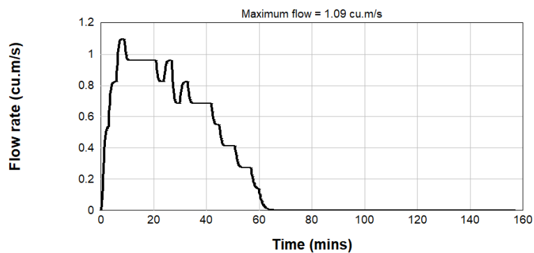
Figure B2.108: Post Development PMF Inflow Hydrograph - Catchment ROAD
