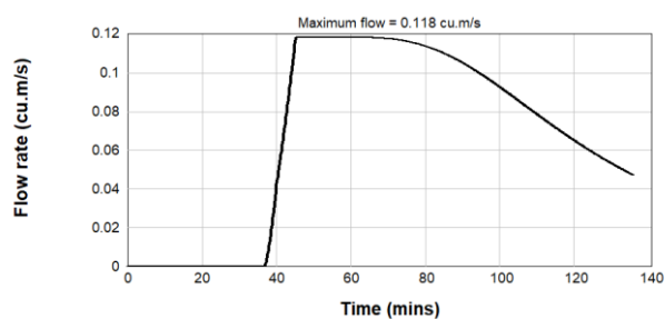
Figure B2.6: Pre & Post Development 4EY Inflow Hydrograph - Catchment U/S4
