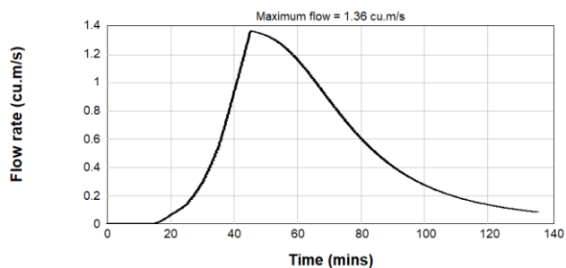
Figure B2.20: Pre-Development 5% AEP Inflow Hydrograph - Catchment 1
