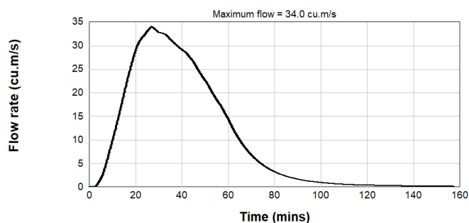
Figure B2.61: Pre & Post Development PMF Inflow Hydrograph - Catchment U/S4
