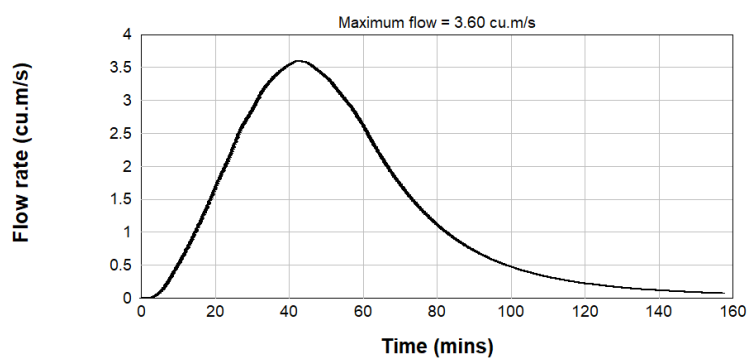
Figure B2.110: Post Development PMF Inflow Hydrograph - Catchment E2
