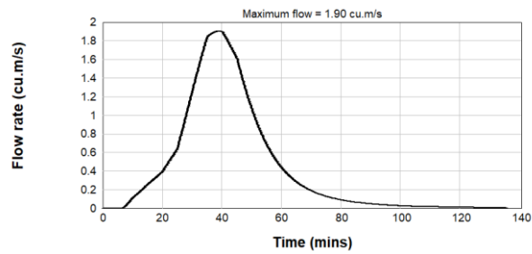
Figure B2.44: Pre-Development 0.5% AEP Inflow Hydrograph - Catchment 3
