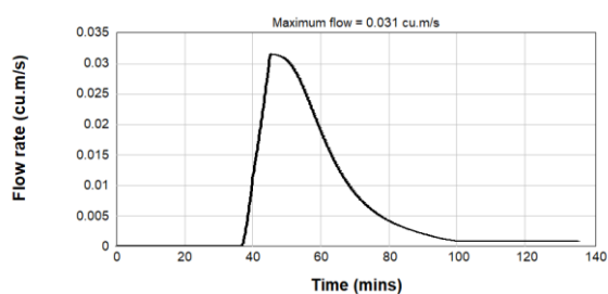
Figure B2.4: Pre & Post Development 4EY Inflow Hydrograph - Catchment U/S2
