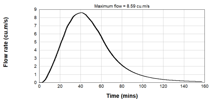
Figure B2.105: Post Development PMF Inflow Hydrograph - Catchment 2-1
