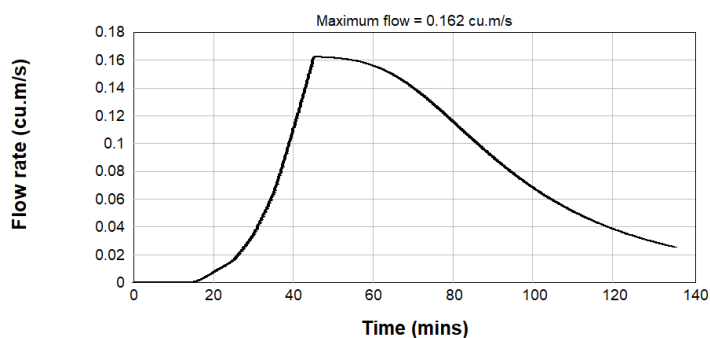
Figure B2.81: Post Development 5% AEP Inflow Hydrograph - Catchment E2-2
