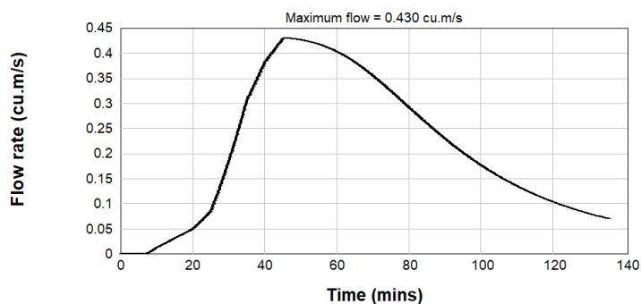
Figure B2.89: Post Development 1% AEP Inflow Hydrograph - Catchment E2
