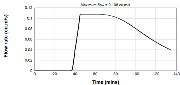
Figure B2.13: Pre-Development 4EY Inflow Hydrograph - Catchment 6
