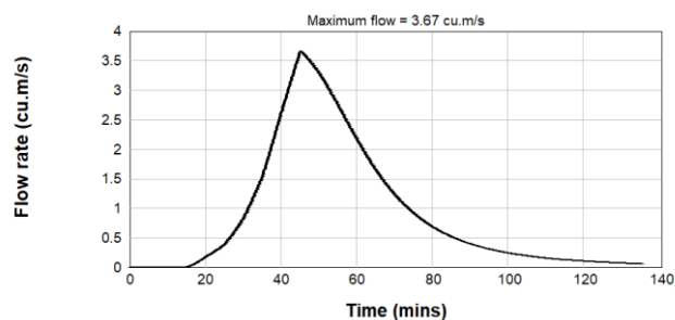
Figure B2.16: Pre & Post Development 5% AEP Inflow Hydrograph - Catchment U/S3
