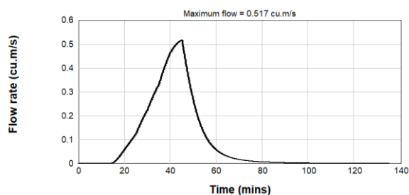
Figure B2.15: Pre & Post Development 5% AEP Inflow Hydrograph - Catchment U/S2
