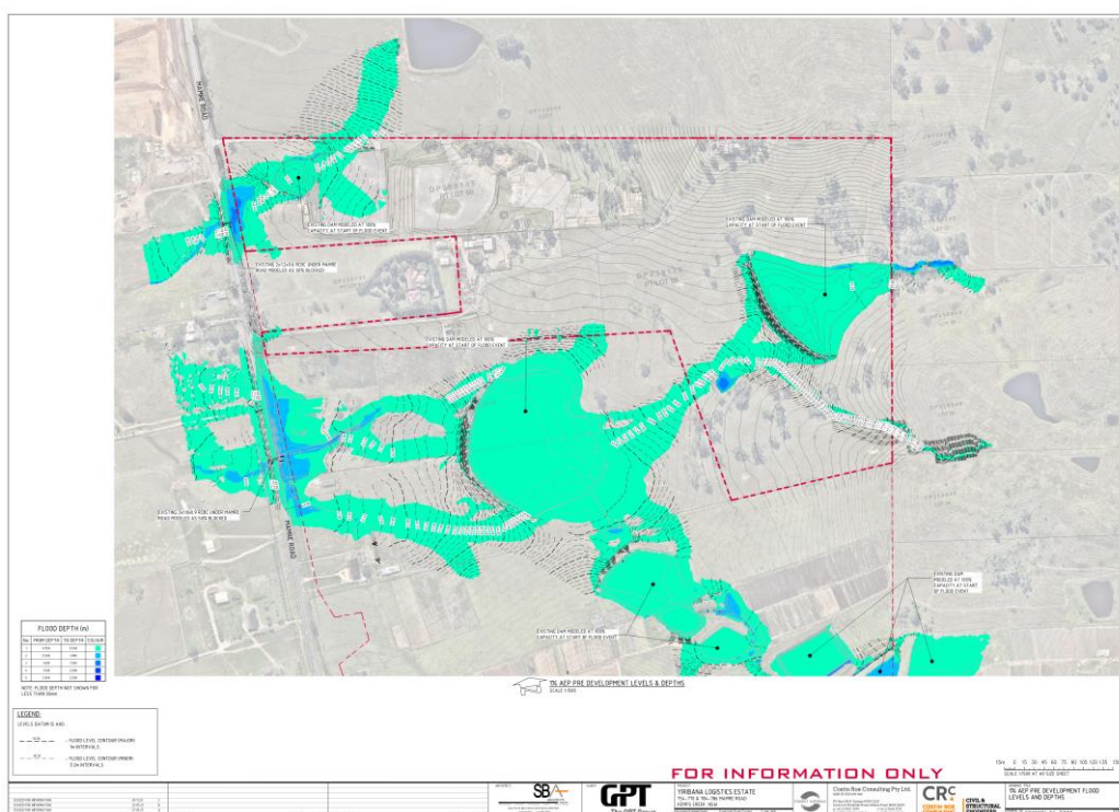
Figure B4.1: 1% AEP Flood Depths – Pre-Development
