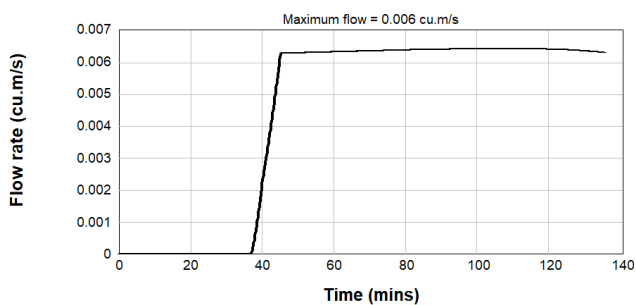
Figure B2.69: Post Development 4EY Inflow Hydrograph – Catchment 1
