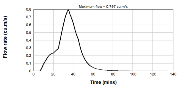
Figure B2.37: Pre & Post Development 0.5% AEP Inflow Hydrograph - Catchment U/S2
