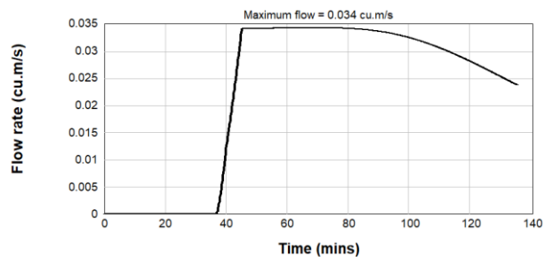
Figure B2.9: Pre-Development 4EY Inflow Hydrograph - Catchment 1
