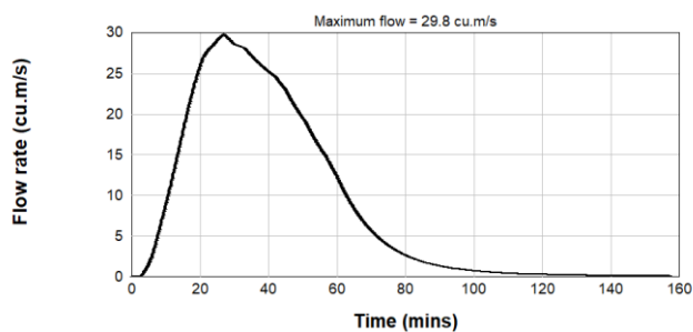
Figure B2.68: Pre-Development PMF Inflow Hydrograph - Catchment 6
