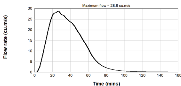
Figure B2.58: Pre & Post Development PMF Inflow Hydrograph - Catchment U/S1
