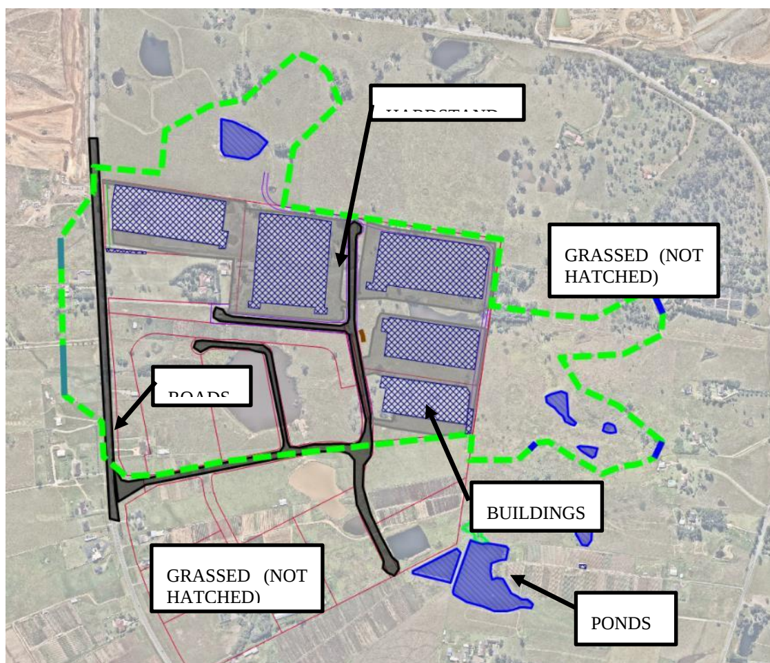
Figure B3.3: Manning's Roughness Surface Areas (Post-Development)
