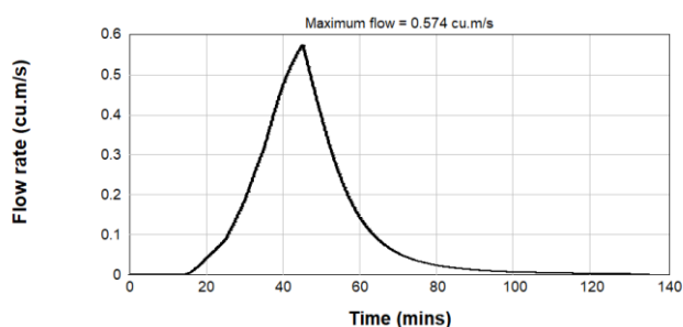
Figure B2.19: Pre & Post Development 5% AEP Inflow Hydrograph - Catchment U/S6
