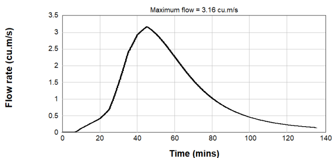
Figure B2.90: Post Development 0.5% AEP Inflow Hydrograph – Catchment 1
