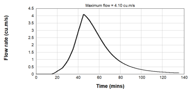
Figure B2.24: Pre-Development 5% AEP Inflow Hydrograph - Catchment 6
