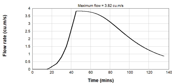
Figure B2.79: Post Development 5% AEP Inflow Hydrograph - Catchment MIRVAC
