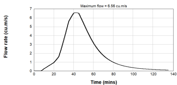
Figure B2.28: Pre & Post Development 1% AEP Inflow Hydrograph - Catchment U/S4
