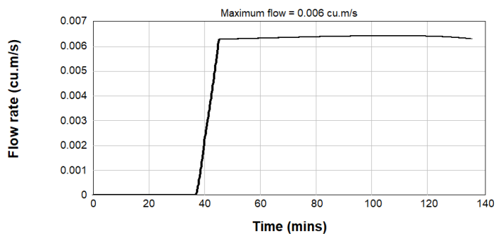
Figure B2.75: Post Development 4EY Inflow Hydrograph - Catchment E2
