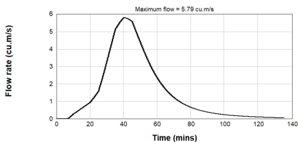
Figure B2.38: Pre & Post Development 0.5% AEP Inflow Hydrograph - Catchment U/S3
