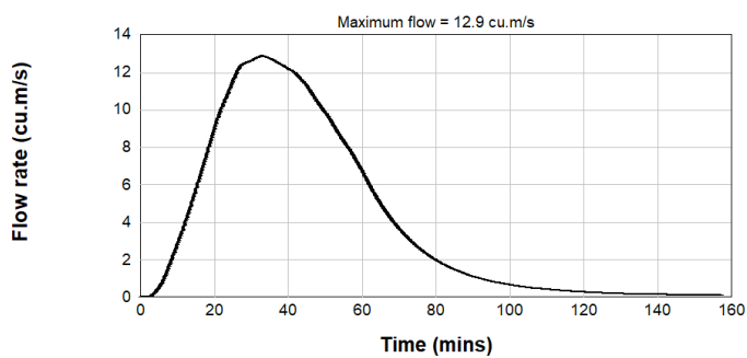
Figure B2.64: Pre-Development PMF Inflow Hydrograph - Catchment 1
