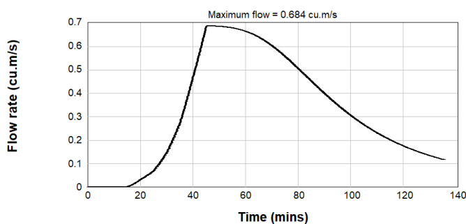
Figure B2.77: Post Development 5% AEP Inflow Hydrograph - Catchment 2-1
