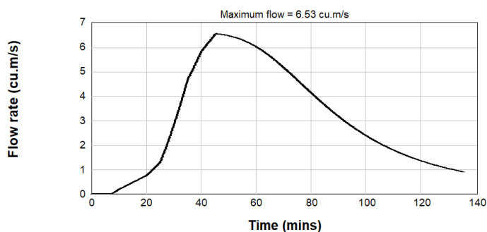
Figure B2.86: Post Development 1% AEP Inflow Hydrograph - Catchment MIRVAC
