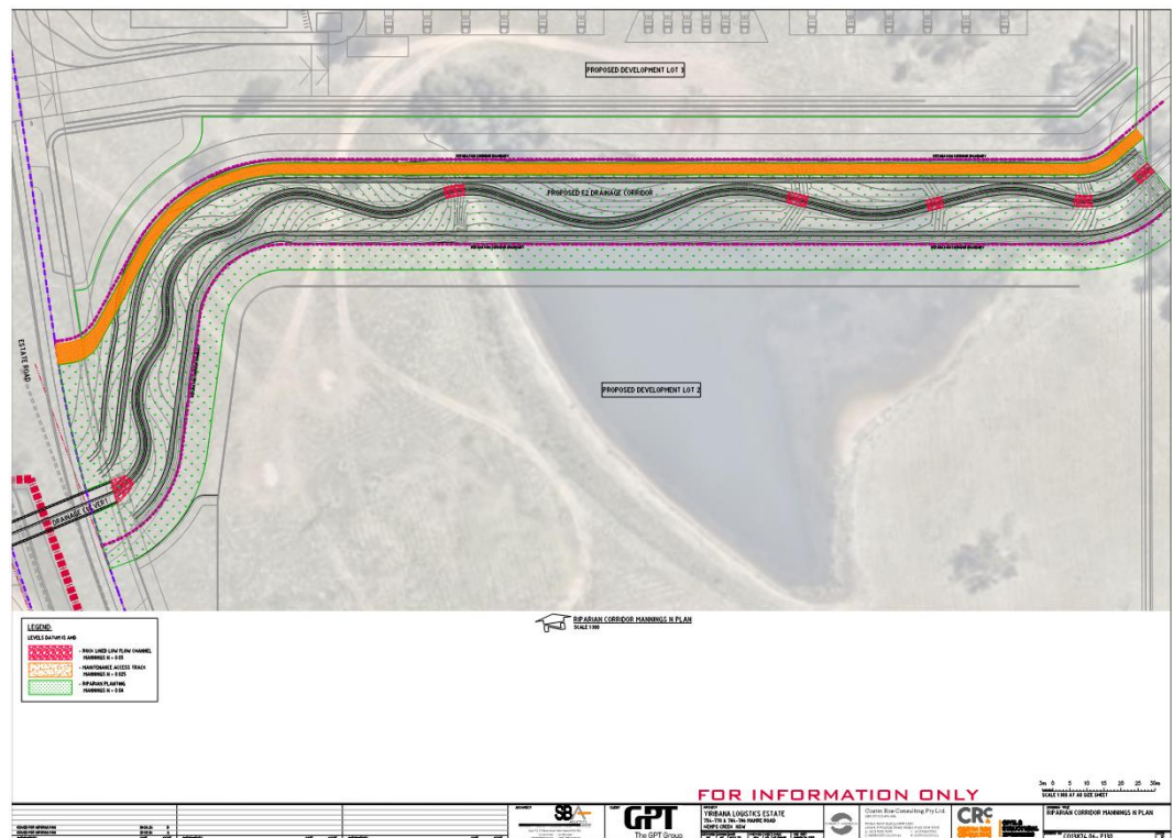
Figure B3.4: Manning's Roughness Surface Areas (Post-Development Riparian Channel)
