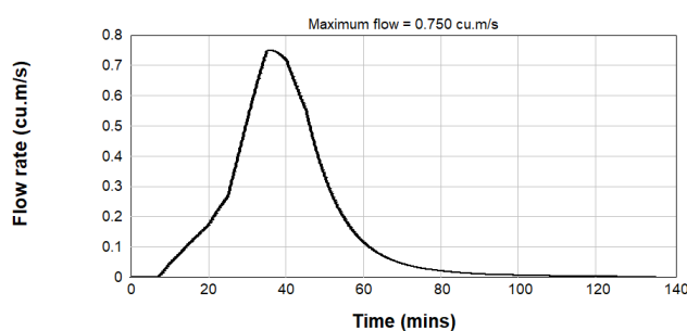
Figure B2.30: Pre & Post Development 1% AEP Inflow Hydrograph - Catchment U/S6
