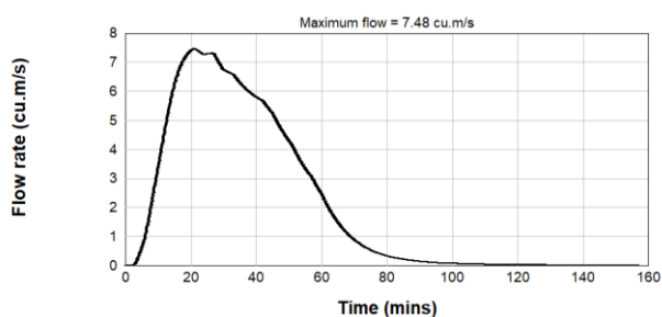
Figure B2.66: Pre-Development PMF Inflow Hydrograph - Catchment 3
