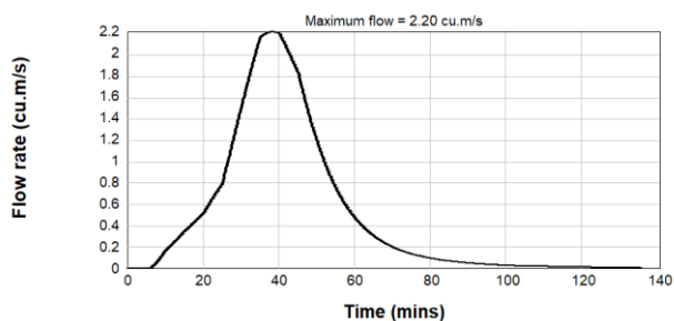
Figure B2.55: Pre-Development 0.2% AEP Inflow Hydrograph - Catchment 3
