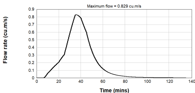
Figure B2.41: Pre & Post Development 0.5% AEP Inflow Hydrograph - Catchment U/S6
