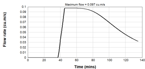
Figure B2.5: Pre & Post Development 4EY Inflow Hydrograph - Catchment U/S3
