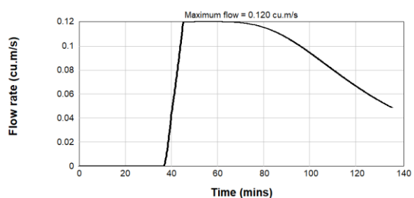
Figure B2.12: Pre-Development 4EY Inflow Hydrograph - Catchment 5
