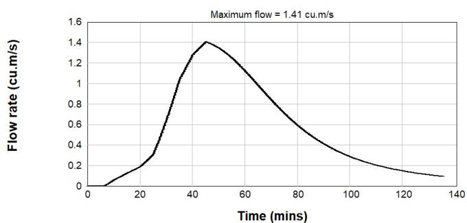
Figure B2.99: Post Development 0.2% AEP Inflow Hydrograph - Catchment 2-3
