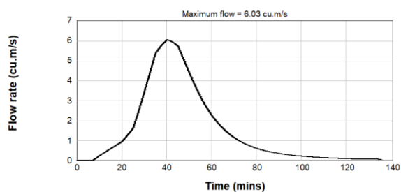
Figure B2.25: Pre & Post Development 1% AEP Inflow Hydrograph - Catchment U/S1
