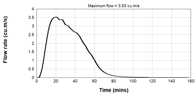
Figure B2.62: Pre & Post Development PMF Inflow Hydrograph - Catchment U/S5
