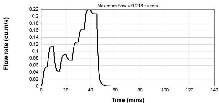
Figure B2.80: Post Development 5% AEP Inflow Hydrograph - Catchment ROAD
