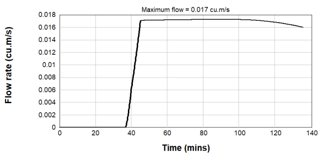
Figure B2.70: Post Development 4EY Inflow Hydrograph - Catchment 2-1
