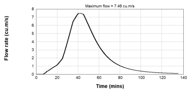
Figure B2.45: Pre-Development 0.5% AEP Inflow Hydrograph - Catchment 5
