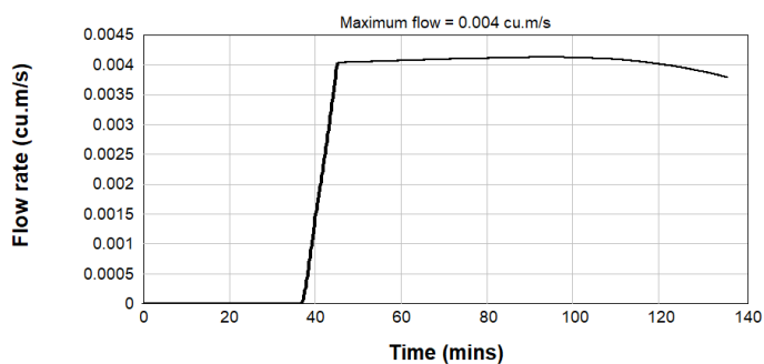
Figure B2.74: Post Development 4EY Inflow Hydrograph - Catchment E2-2
