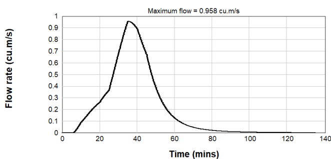
Figure B2.52: Pre & Post Development 0.2% AEP Inflow Hydrograph - Catchment U/S6
