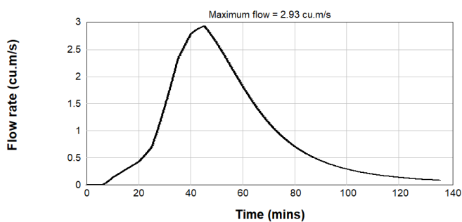
Figure B2.53: Pre-Development 0.2% AEP Inflow Hydrograph - Catchment 1
