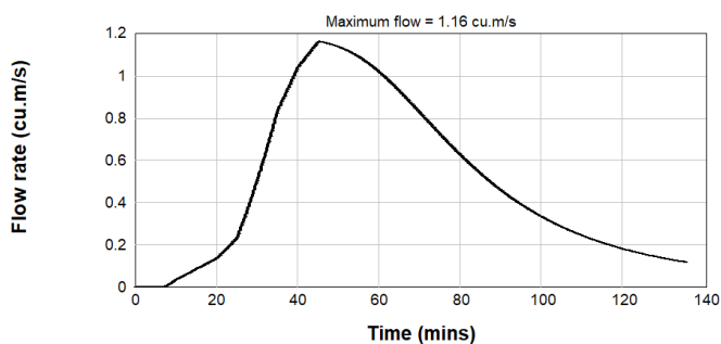
Figure B2.84: Post Development 1% AEP Inflow Hydrograph - Catchment 2-1
