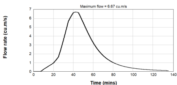
Figure B2.34: Pre-Development 1% AEP Inflow Hydrograph - Catchment 5
