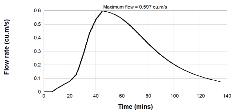
Figure B2.103: Post Development 0.2% AEP Inflow Hydrograph - Catchment E2
