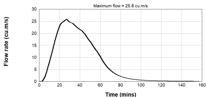
Figure B2.60: Pre & Post Development PMF Inflow Hydrograph - Catchment U/S3
