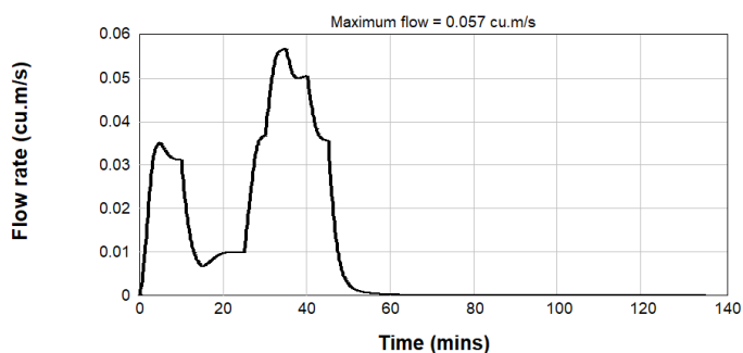
Figure B2.73: Post Development 4EY Inflow Hydrograph - Catchment ROAD
