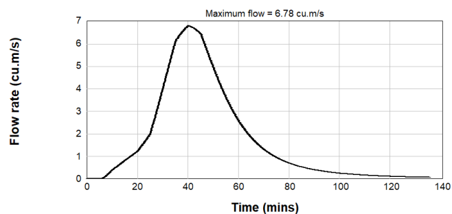
Figure B2.50: Pre & Post Development 0.2% AEP Inflow Hydrograph - Catchment U/S4
