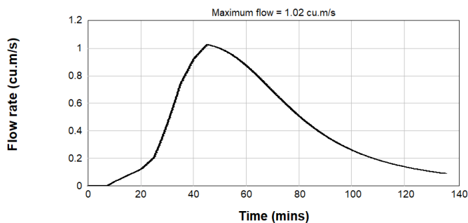
Figure B2.85: Post Development 1% AEP Inflow Hydrograph - Catchment 2-3
