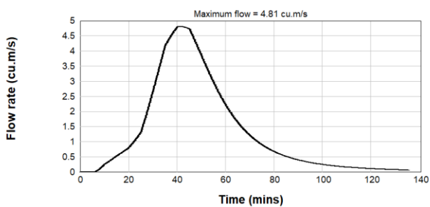
Figure B2.54: Pre-Development 0.2% AEP Inflow Hydrograph - Catchment 2
