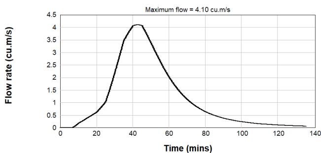
Figure B2.43: Pre-Development 0.5% AEP Inflow Hydrograph - Catchment 2
