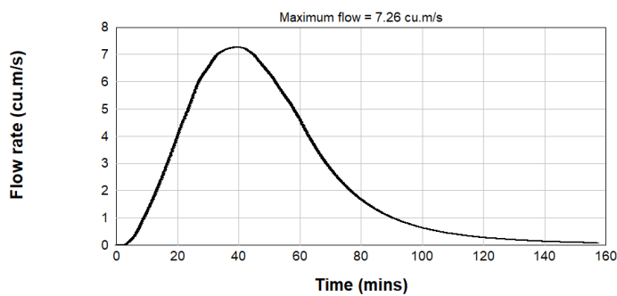
Figure B2.106: Post Development PMF Inflow Hydrograph - Catchment 2-3
