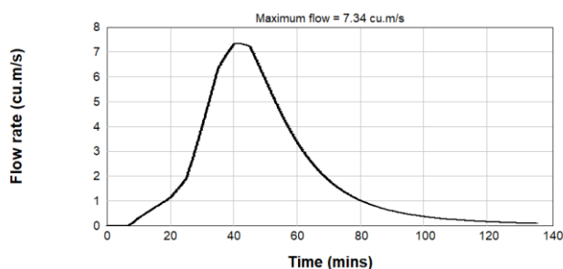
Figure B2.39: Pre & Post Development 0.5% AEP Inflow Hydrograph - Catchment U/S4
