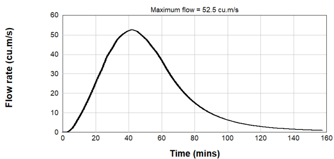
Figure B2.107: Post Development PMF Inflow Hydrograph - Catchment MIRVAC
