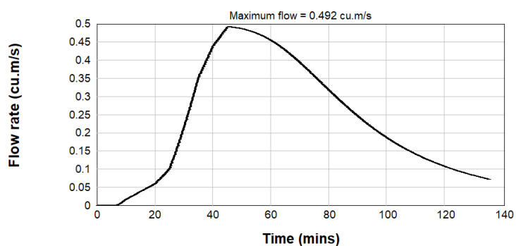
Figure B2.96: Post Development 0.5% AEP Inflow Hydrograph - Catchment E2
