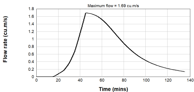
Figure B2.76: Post Development 5% AEP Inflow Hydrograph – Catchment 1
