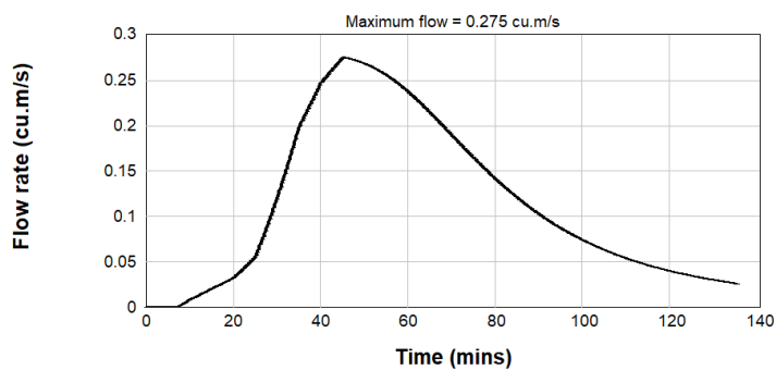
Figure B2.88: Post Development 1% AEP Inflow Hydrograph - Catchment E2-2
