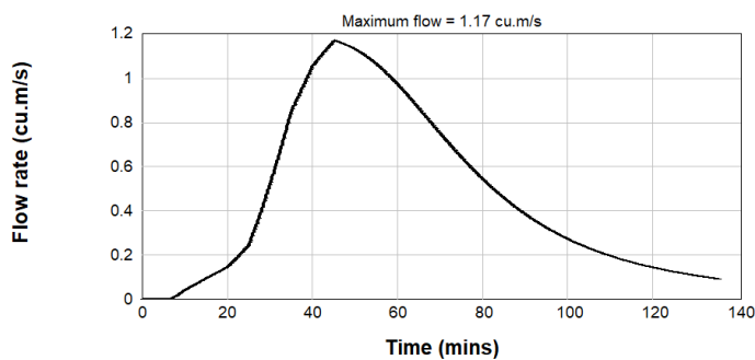
Figure B2.92: Post Development 0.5% AEP Inflow Hydrograph - Catchment 2-3
