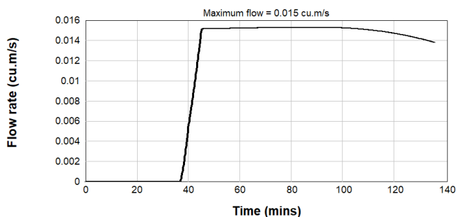
Figure B2.71: Post Development 4EY Inflow Hydrograph - Catchment 2-3
