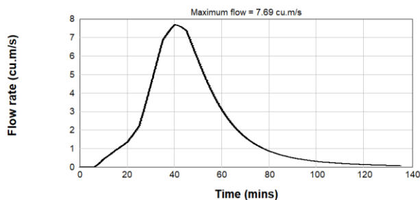
Figure B2.57: Pre-Development 0.2% AEP Inflow Hydrograph - Catchment 6
