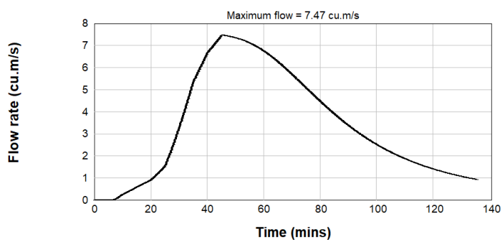
Figure B2.93: Post Development 0.5% AEP Inflow Hydrograph - Catchment MIRVAC
