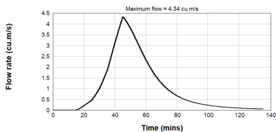
Figure B2.14: Pre & Post Development 5% AEP Inflow Hydrograph - Catchment U/S1
