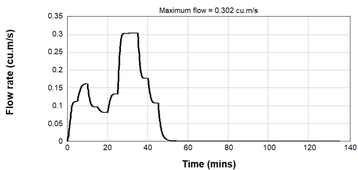
Figure B2.87: Post Development 1% AEP Inflow Hydrograph - Catchment ROAD
