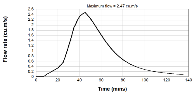
Figure B2.42: Pre-Development 0.5% AEP Inflow Hydrograph - Catchment 1
