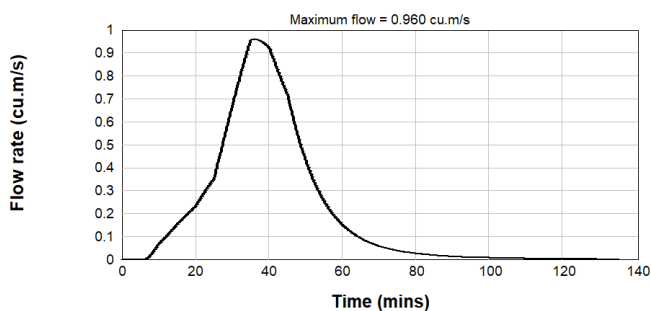
Figure B2.40: Pre & Post Development 0.5% AEP Inflow Hydrograph - Catchment U/S5
