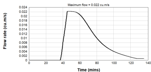
Figure B2.8: Pre & Post Development 4EY Inflow Hydrograph - Catchment U/S6
