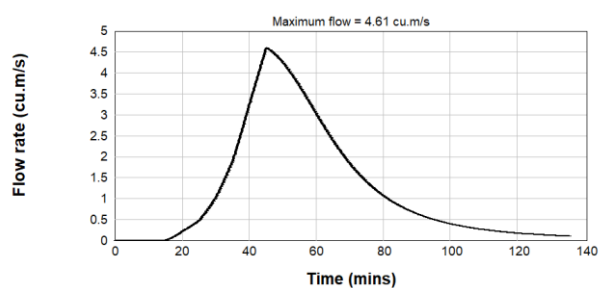
Figure B2.23: Pre-Development 5% AEP Inflow Hydrograph - Catchment 5
