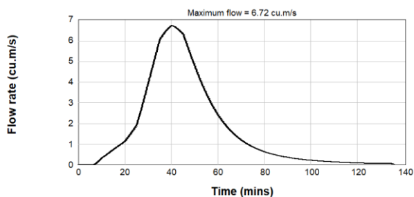
Figure B2.36: Pre & Post Development 0.5% AEP Inflow Hydrograph - Catchment U/S1
