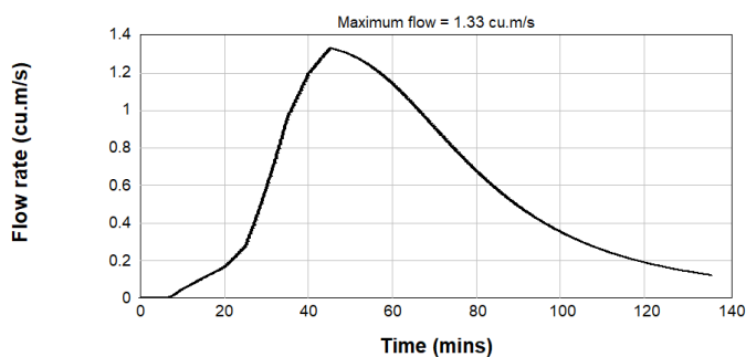
Figure B2.91: Post Development 0.5% AEP Inflow Hydrograph - Catchment 2-1
