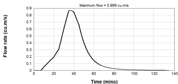
Figure B2.29: Pre & Post Development 1% AEP Inflow Hydrograph - Catchment U/S5
