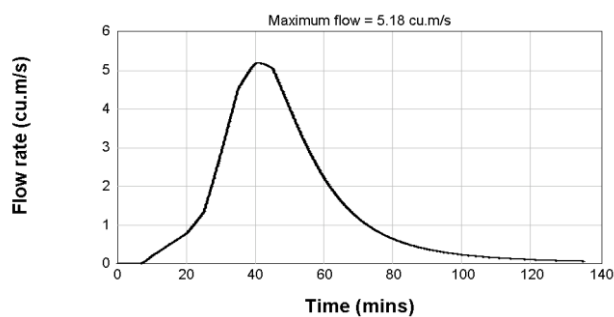
Figure B2.27: Pre & Post Development 1% AEP Inflow Hydrograph - Catchment U/S3
