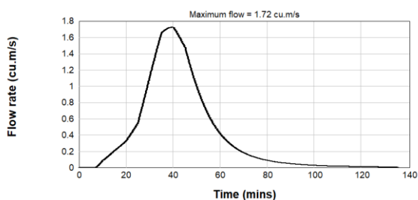
Figure B2.33: Pre-Development 1% AEP Inflow Hydrograph - Catchment 3
