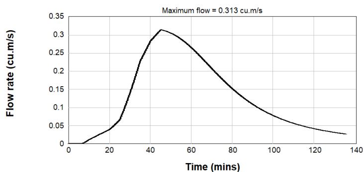
Figure B2.95: Post Development 0.5% AEP Inflow Hydrograph - Catchment E2-2
