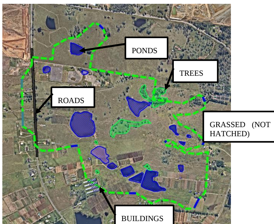
Figure B3.2: Manning's Roughness Surface Areas (Pre-Development)
