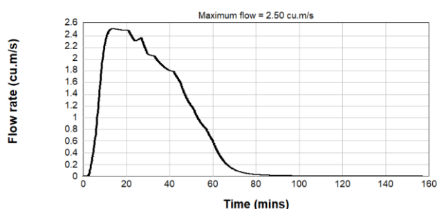
Figure B2.59: Pre & Post Development PMF Inflow Hydrograph - Catchment U/S2
