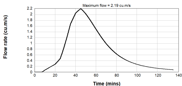
Figure B2.31: Pre-Development 1% AEP Inflow Hydrograph - Catchment 1
