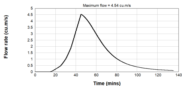
Figure B2.17: Pre & Post Development 5% AEP Inflow Hydrograph - Catchment U/S4
