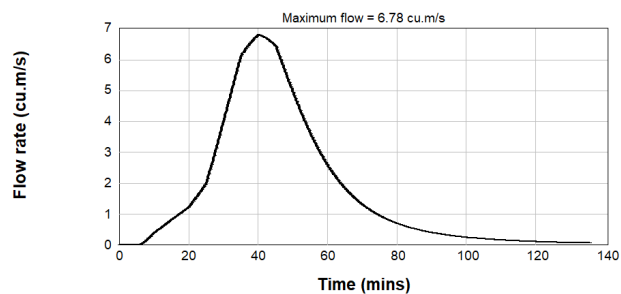
Figure B2.49: Pre & Post Development 0.2% AEP Inflow Hydrograph - Catchment U/S3
