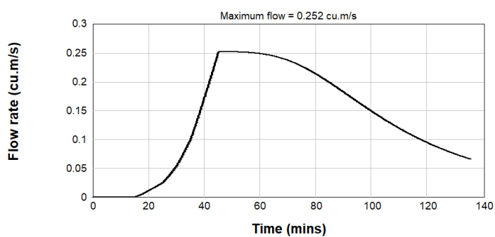
Figure B2.82: Post Development 5% AEP Inflow Hydrograph - Catchment E2
