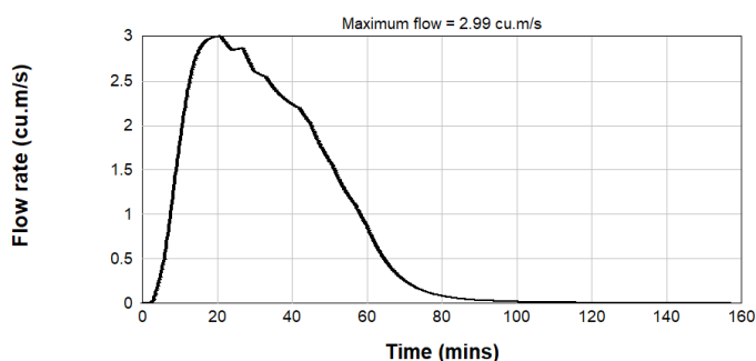
Figure B2.63: Pre & Post Development PMF Inflow Hydrograph - Catchment U/S6
