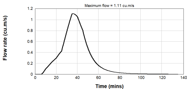
Figure B2.51: Pre & Post Development 0.2% AEP Inflow Hydrograph - Catchment U/S5
