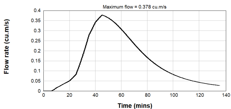
Figure B2.102: Post Development 0.2% AEP Inflow Hydrograph - Catchment E2-2
