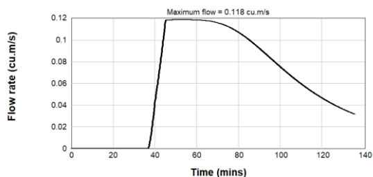
Figure B2.3: Pre & Post Development 4EY Inflow Hydrograph - Catchment U/S1
