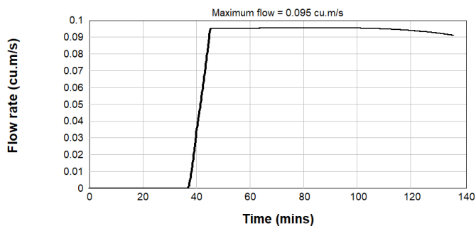
Figure B2.72: Post Development 4EY Inflow Hydrograph - Catchment MIRVAC
