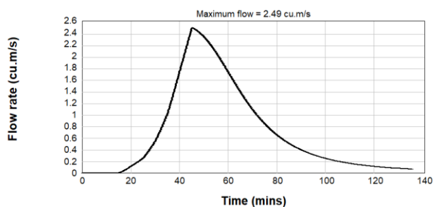
Figure B2.21: Pre-Development 5% AEP Inflow Hydrograph - Catchment 2
