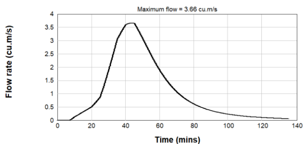
Figure B2.32: Pre-Development 1% AEP Inflow Hydrograph - Catchment 2
