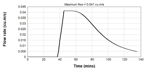
Figure B2.11: Pre-Development 4EY Inflow Hydrograph - Catchment 3
