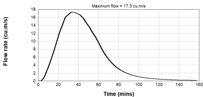
Figure B2.104: Post Development PMF Inflow Hydrograph – Catchment 1
