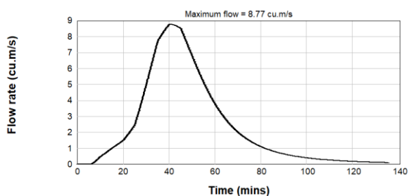
Figure B2.56: Pre-Development 0.2% AEP Inflow Hydrograph - Catchment 5
