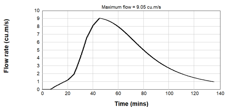
Figure B2.100: Post Development 0.2% AEP Inflow Hydrograph - Catchment MIRVAC
