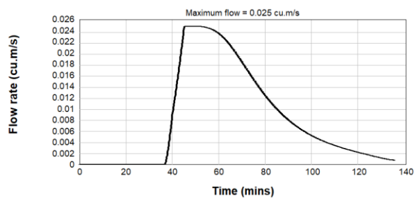
Figure B2.7: Pre & Post Development 4EY Inflow Hydrograph - Catchment U/S5
