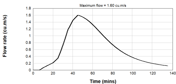
Figure B2.98: Post Development 0.2% AEP Inflow Hydrograph - Catchment 2-1
