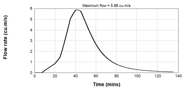
Figure B2.35: Pre-Development 1% AEP Inflow Hydrograph - Catchment 6
