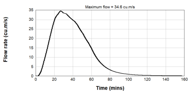
Figure B2.67: Pre-Development PMF Inflow Hydrograph - Catchment 5
