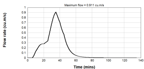
Figure B2.48: Pre & Post Development 0.2% AEP Inflow Hydrograph - Catchment U/S2
