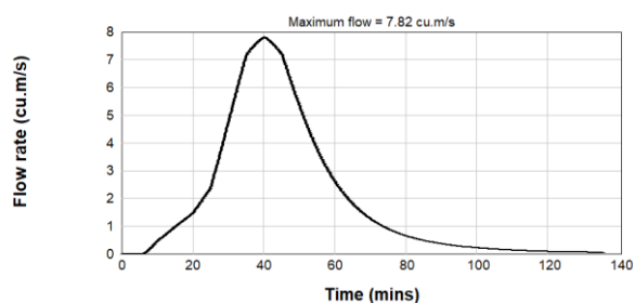
Figure B2.47: Pre & Post Development 0.2% AEP Inflow Hydrograph - Catchment U/S1
