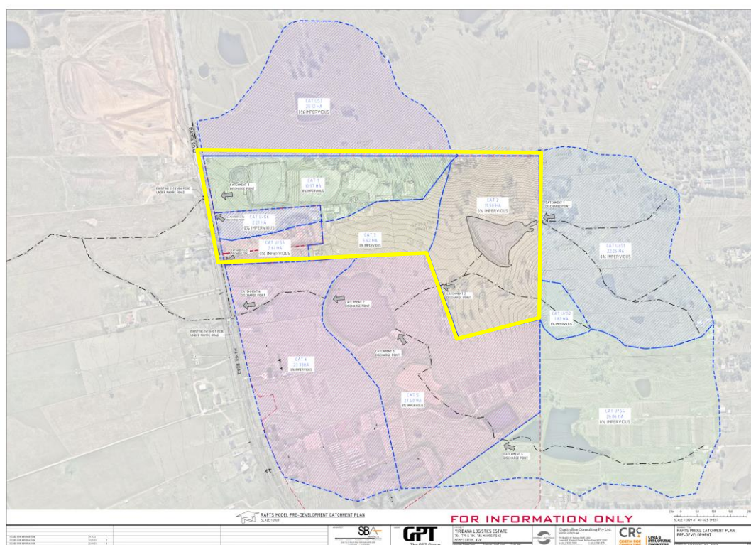
Figure B2.1. Pre-Development Contributing Catchment.
