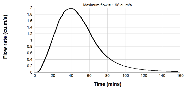
Figure B2.109: Post Development PMF Inflow Hydrograph - Catchment E2-2
