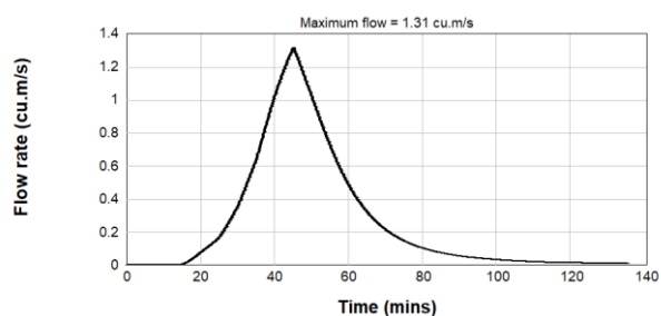
Figure B2.22: Pre-Development 5% AEP Inflow Hydrograph - Catchment 3
