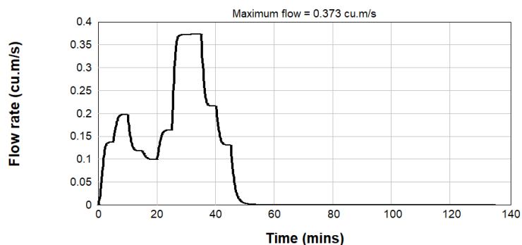
Figure B2.101: Post Development 0.2% AEP Inflow Hydrograph - Catchment ROAD
