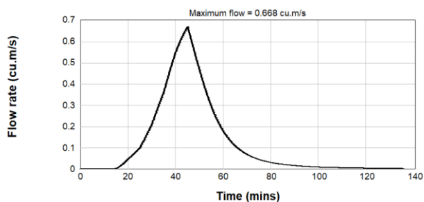
Figure B2.18: Pre & Post Development 5% AEP Inflow Hydrograph - Catchment U/S5
