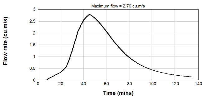
Figure B2.83: Post Development 1% AEP Inflow Hydrograph – Catchment 1
