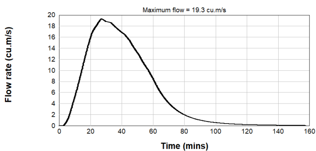
Figure B2.65: Pre-Development PMF Inflow Hydrograph - Catchment 2
