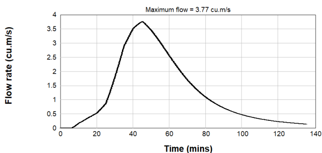
Figure B2.97: Post Development 0.2% AEP Inflow Hydrograph – Catchment 1
