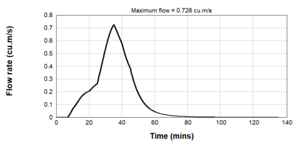
Figure B2.26: Pre & Post Development 1% AEP Inflow Hydrograph - Catchment U/S2
