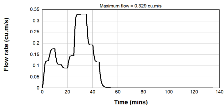
Figure B2.94: Post Development 0.5% AEP Inflow Hydrograph - Catchment ROAD
