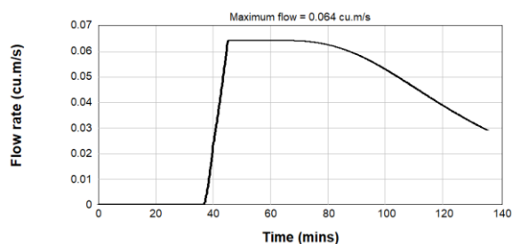
Figure B2.10: Pre-Development 4EY Inflow Hydrograph - Catchment 2
