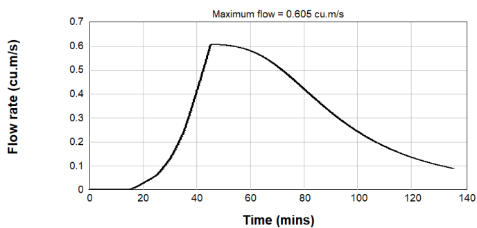
Figure B2.78: Post Development 5% AEP Inflow Hydrograph - Catchment 2-3
