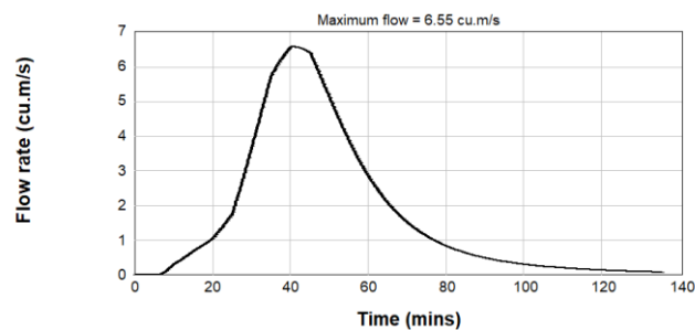
Figure B2.46: Pre-Development 0.5% AEP Inflow Hydrograph - Catchment 6
