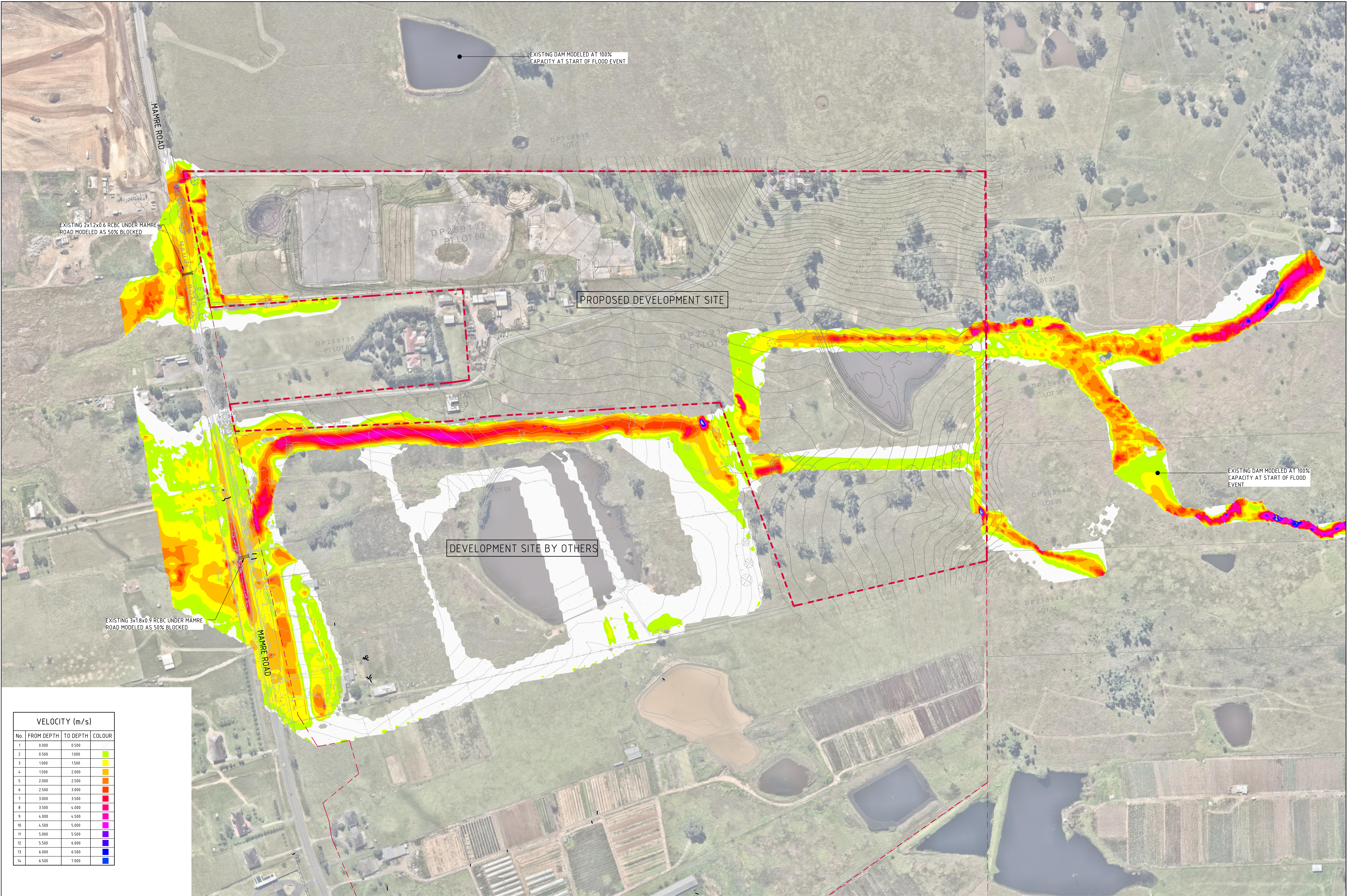
PMF POST DEVELOPMENT VELOCITY SCALE 1:1500
