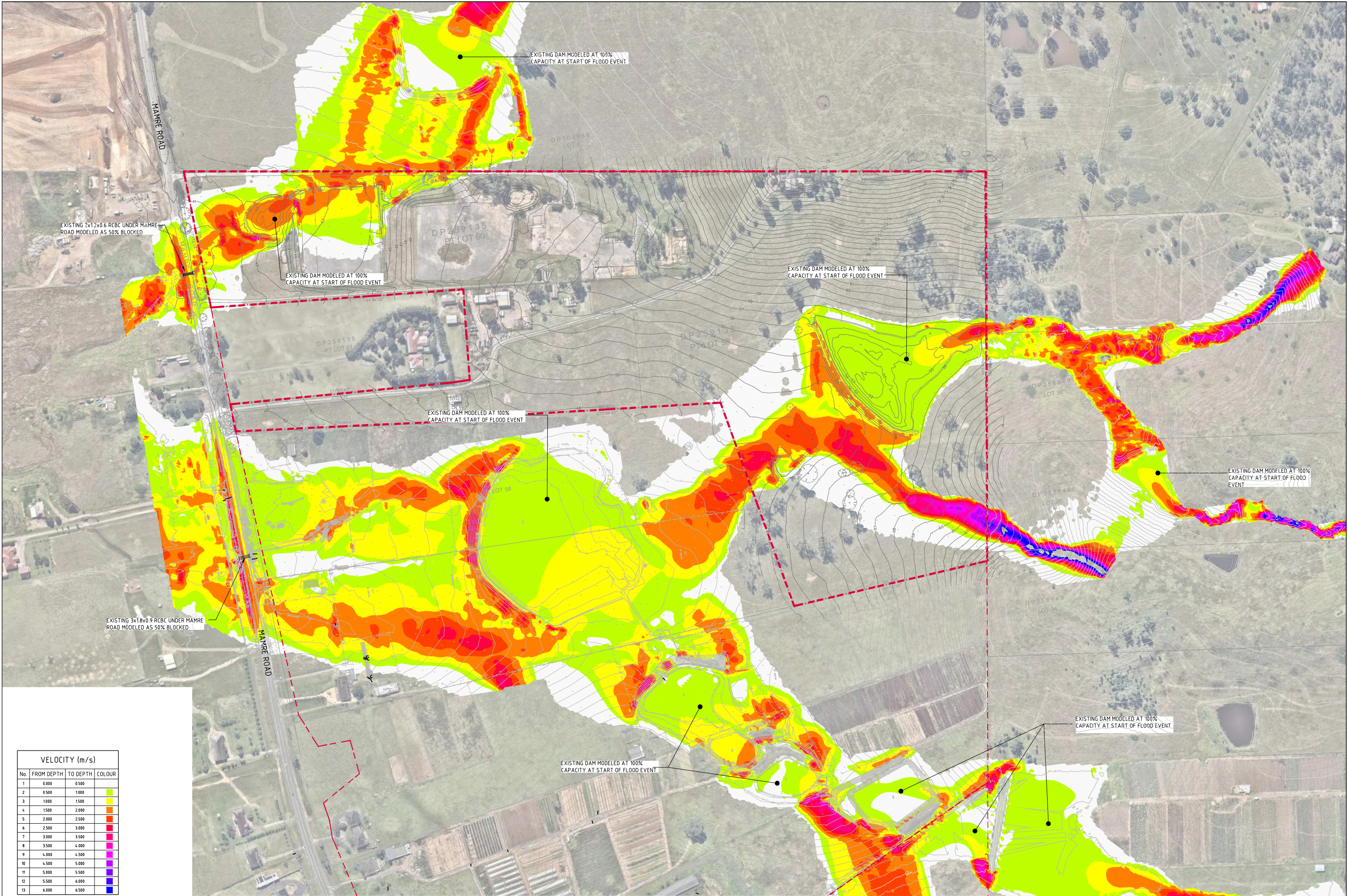
PMF PRE DEVELOPMENT VELOCITY SCALE 1:1500
