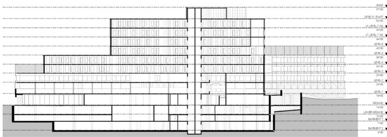
Figure 3: Building Section of the Proposed Development
