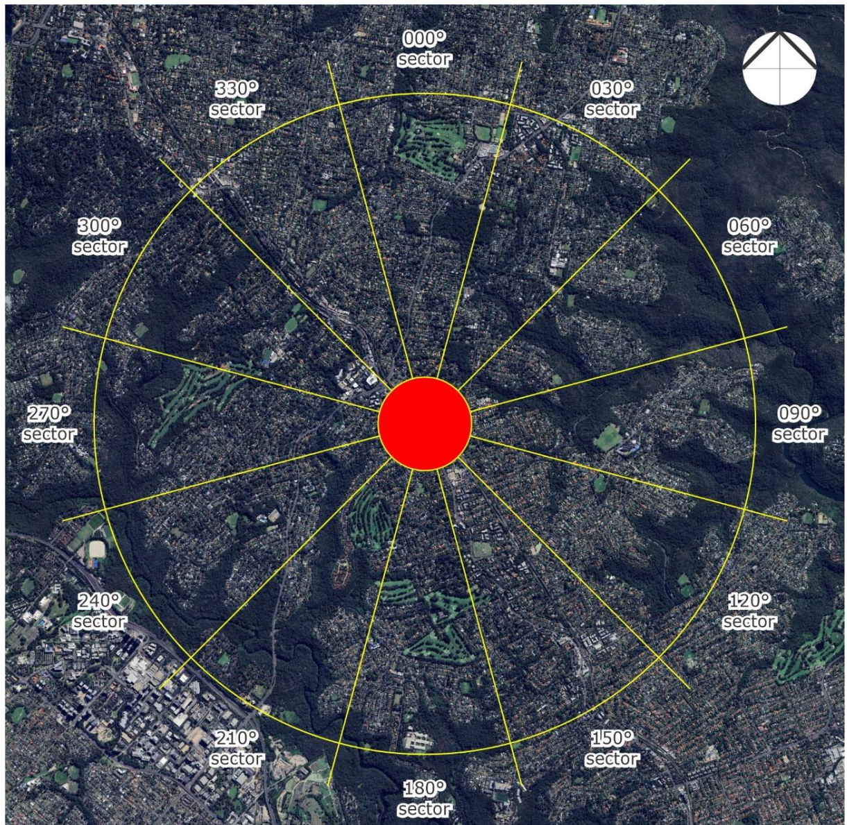
Figure 3: Aerial Image of the Surrounding Terrain (radius of 3.0km from the edge of the proximity model)
