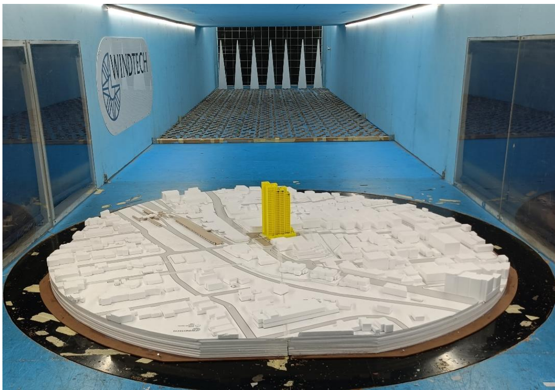
Figure 1b: Photograph of the Wind Tunnel Model (view from the north)
