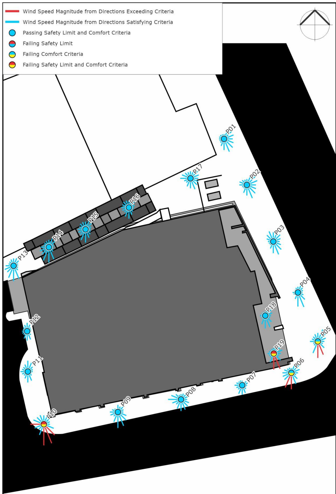
Figure 6a: Wind Tunnel Results – Ground Level Plan (results shown without treatments applied)
