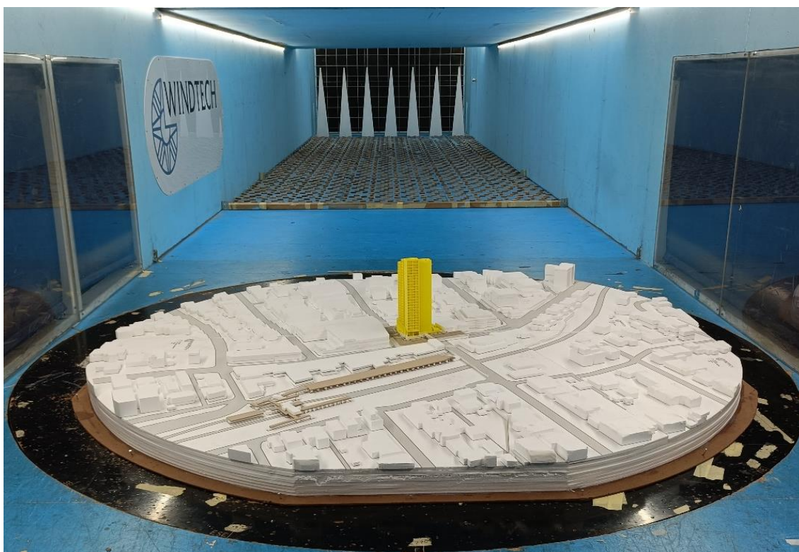
Figure 1c: Photograph of the Wind Tunnel Model (view from the east)
