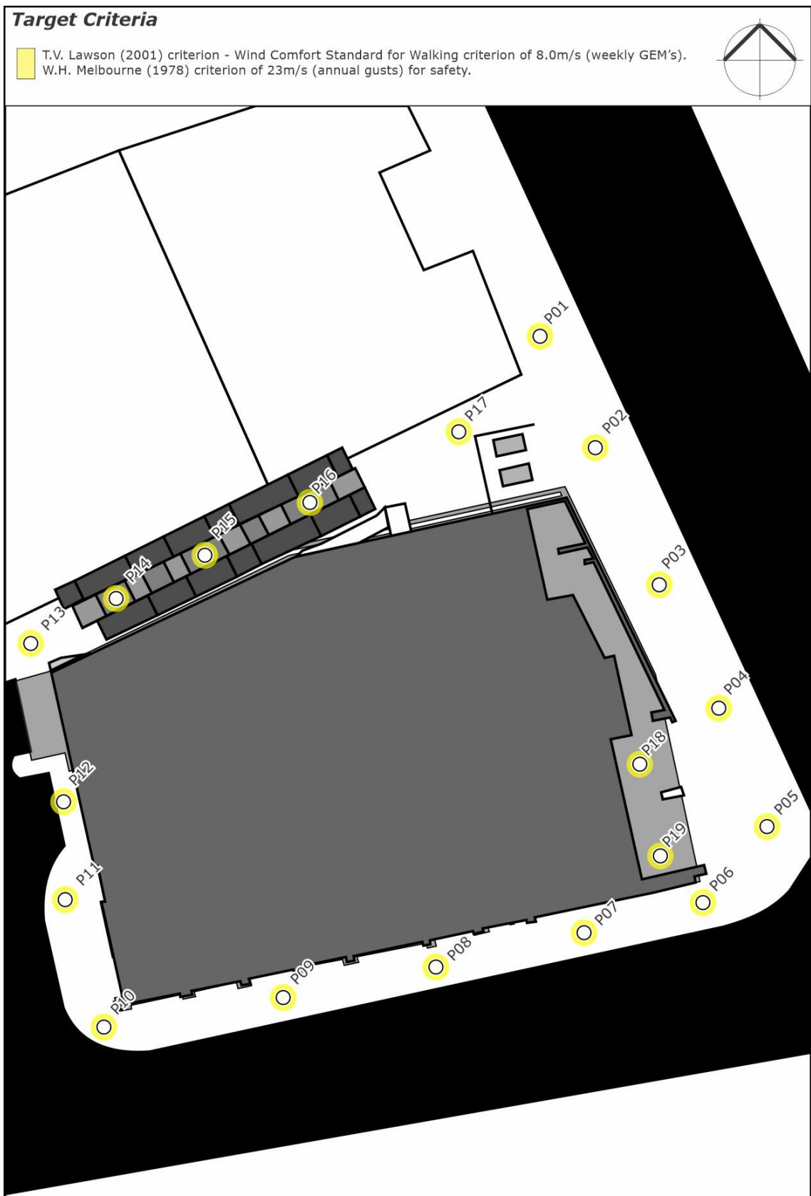
Figure 5a: Study Point Locations and Target Wind Speed Criteria – Ground Level Plan
