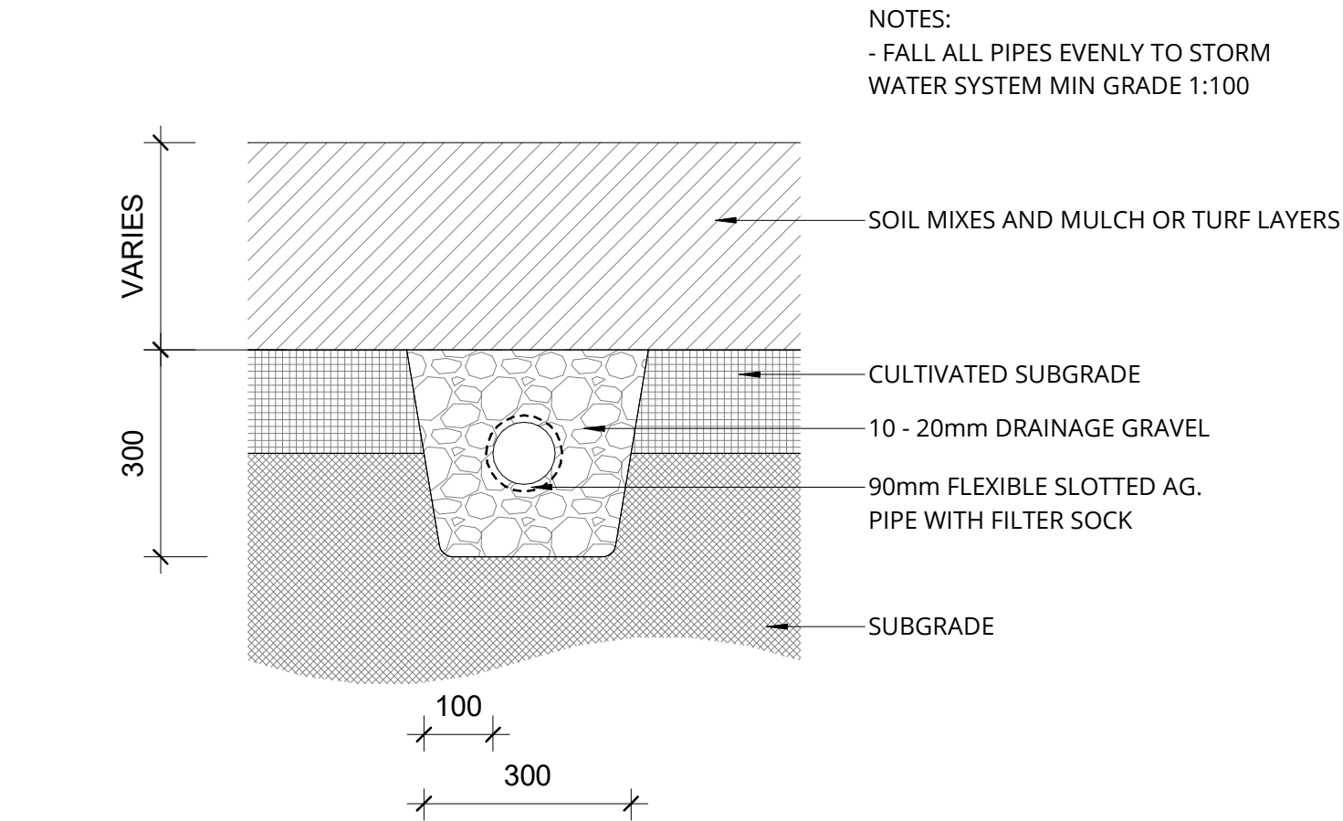
3 SUB SOIL DRAINAGE 1 : 10
