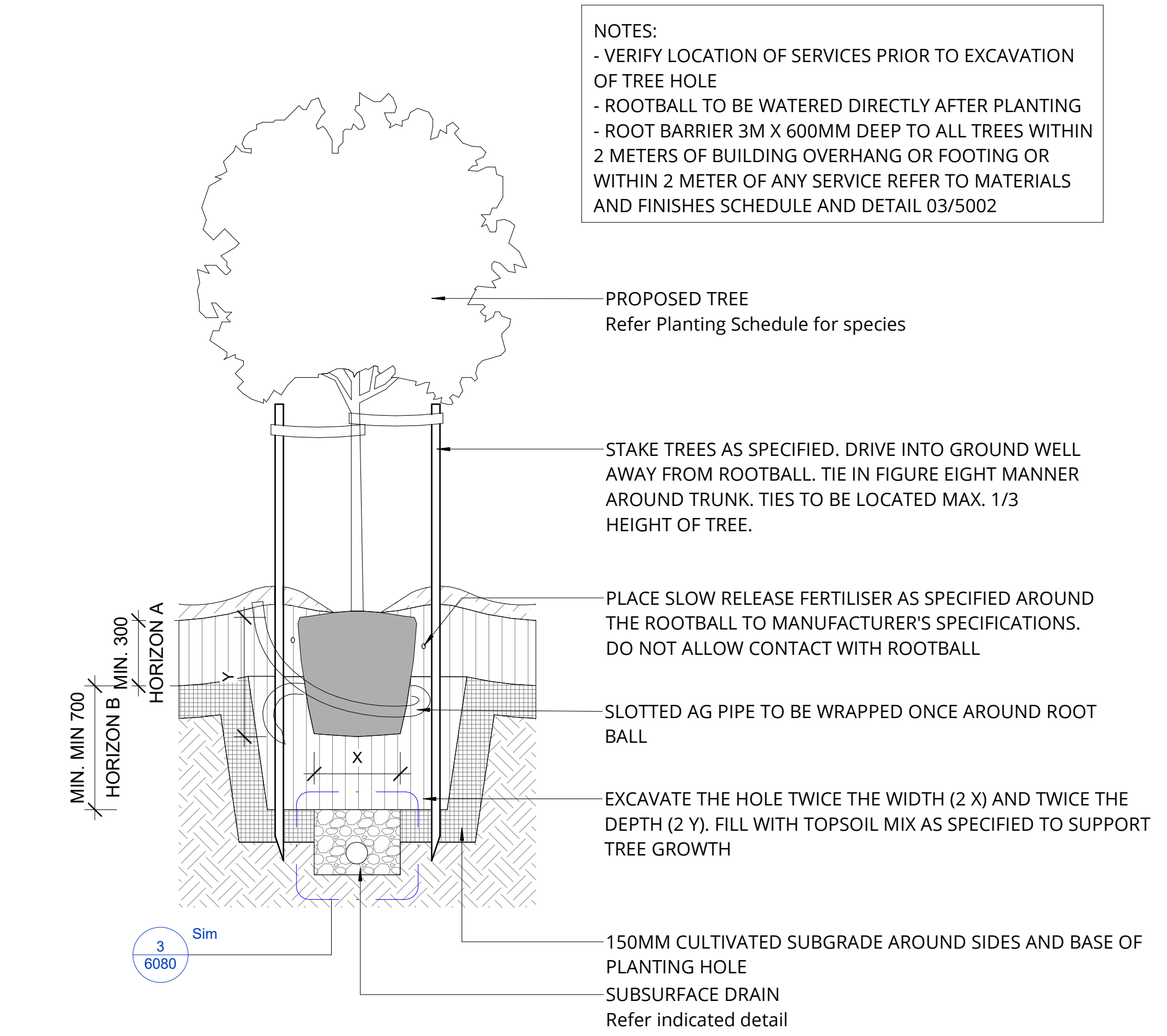
2 TREE PLANTING 1 : 20
