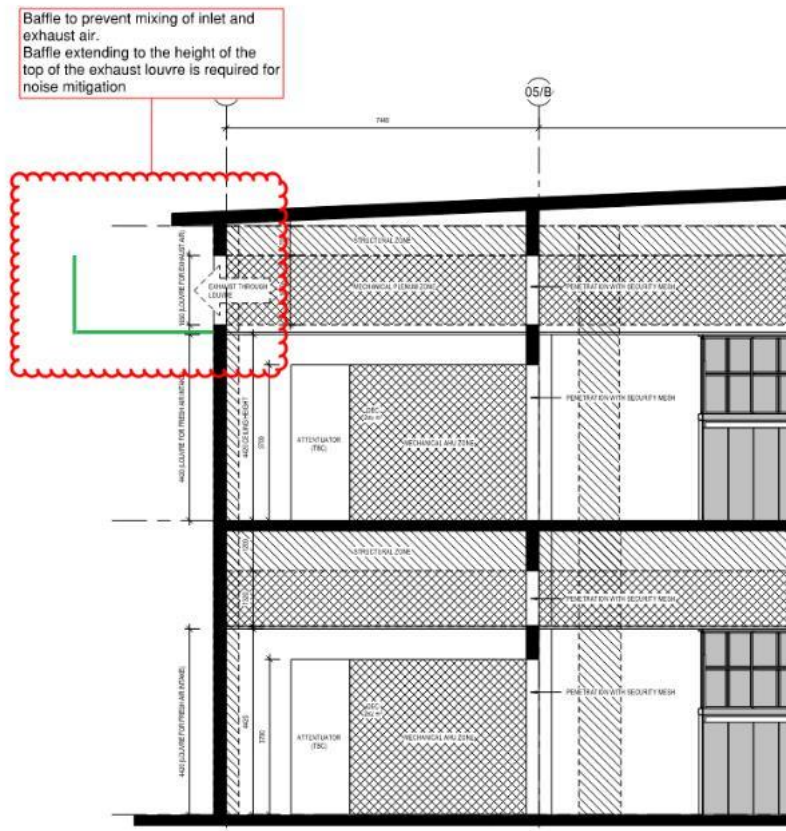
Figure 7: Acoustic requirements for baffle to separate discharge and inlet air
