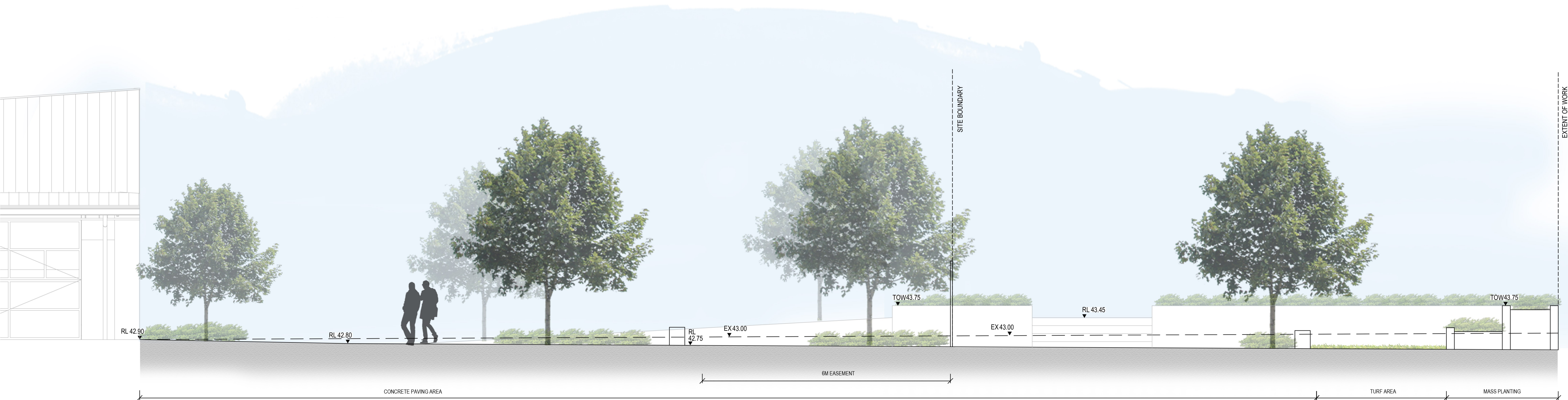
01 SECTION 1 : ENTRY PLAZA (SCENARIO 1) 9001 1:50 SECTION
