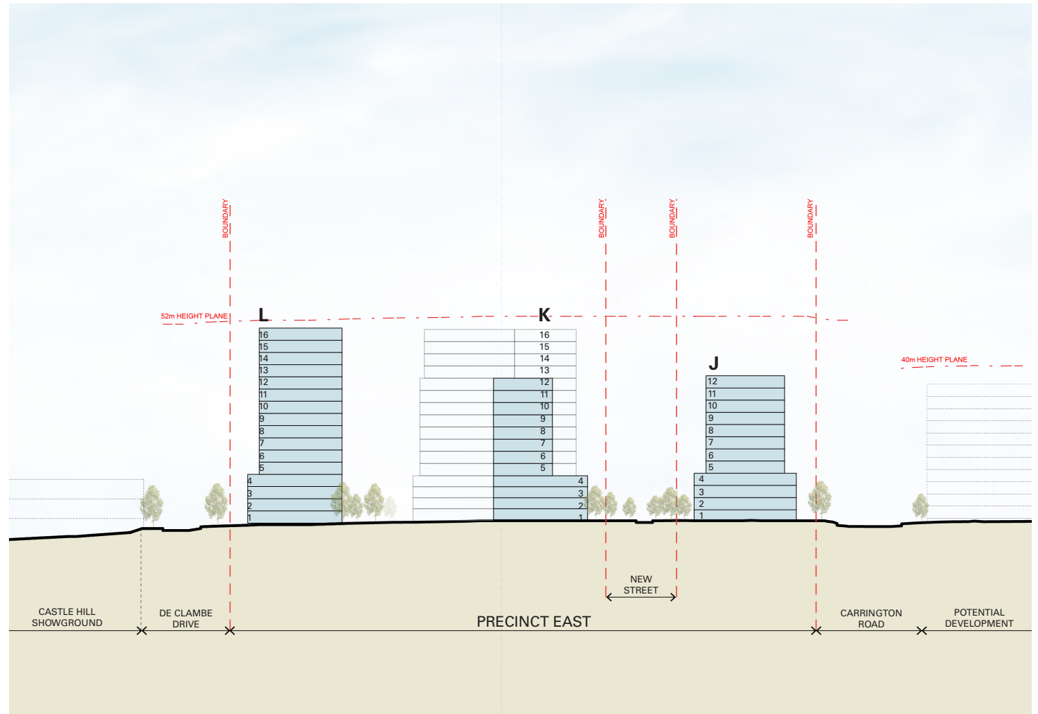
Figure 89: Site Section 02
