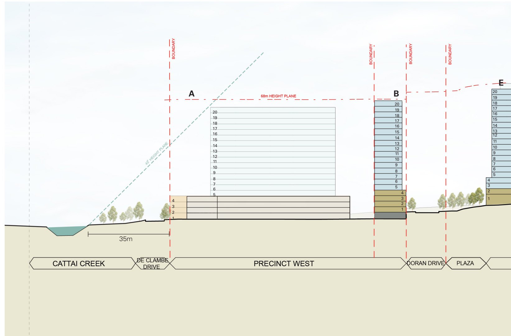
Figure 88: Site Section 01
