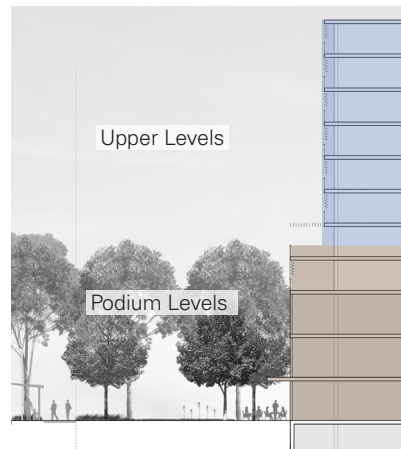
Figure 185: Building configuration
