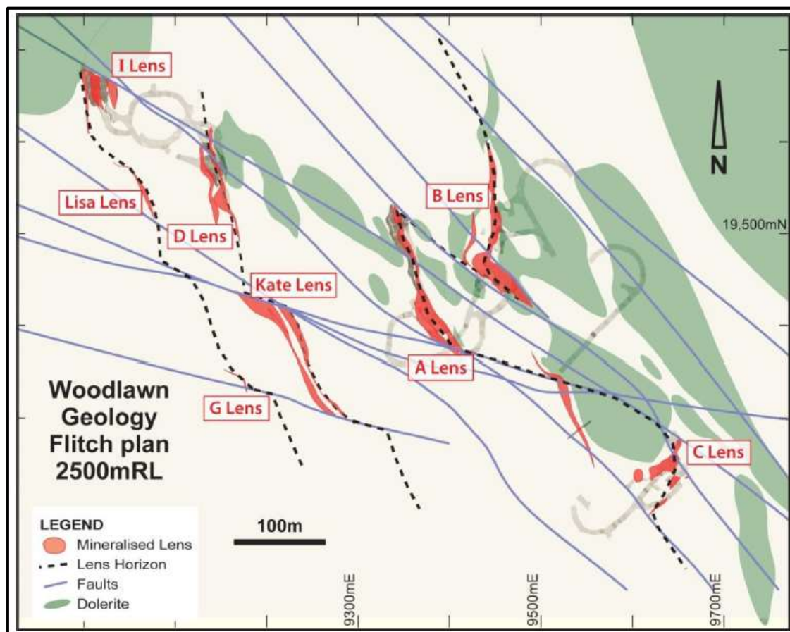
Figure 2.7 - Simplified Geology
