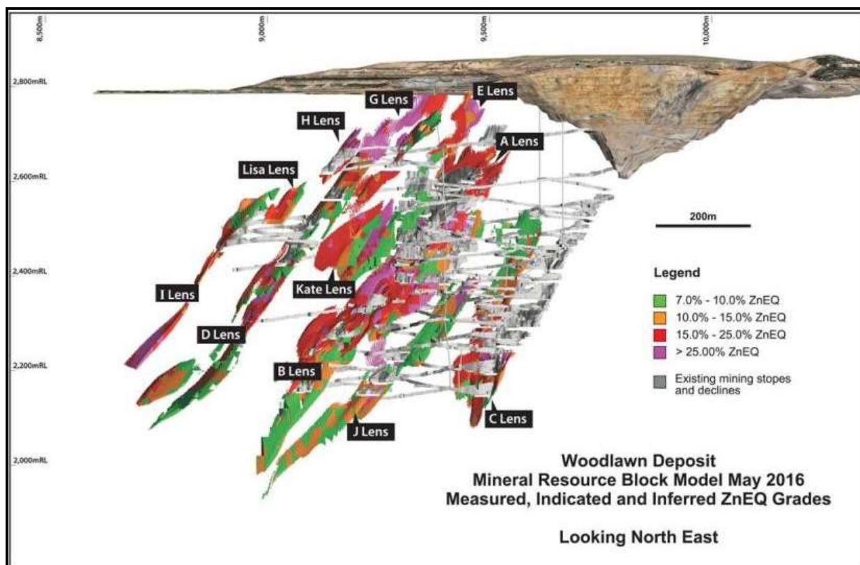
Figure 2.1 – Woodlawn ore lenses (looking north east)
