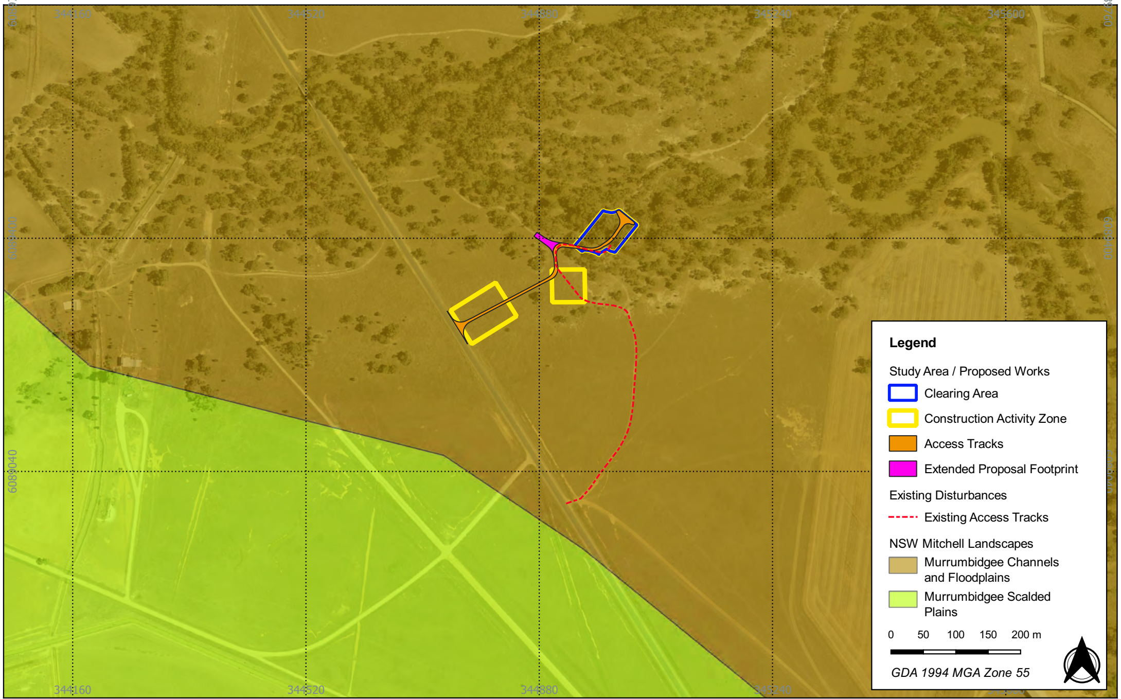
Figure 3.6 - Mitchell soil landscapes identified within the Forest Creek Block Bank
