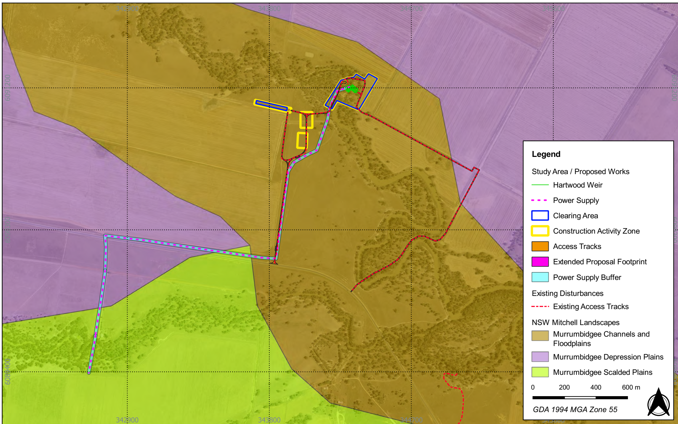
Figure 3.5 - Mitchell soil landscapes identified within the Hartwood Weir study area
