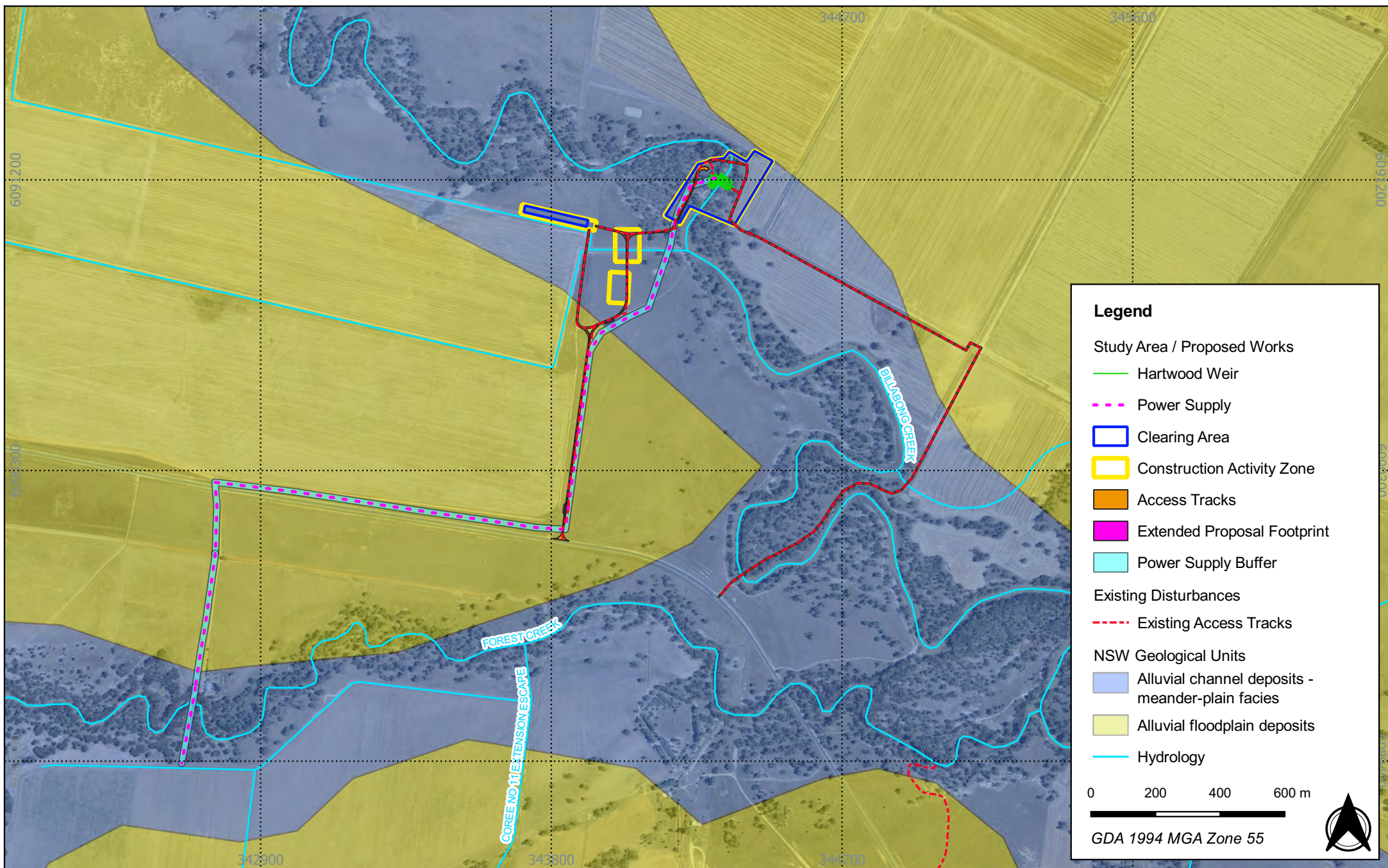
Figure 3.1 - Geology and hydrology of the Hartwood Weir study area
