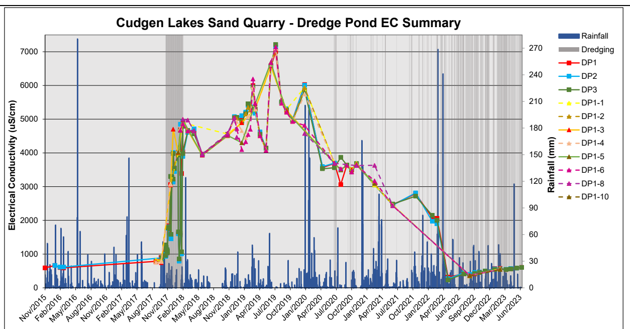
Figure 7.2 DREDGE POND EC SUMMARY
