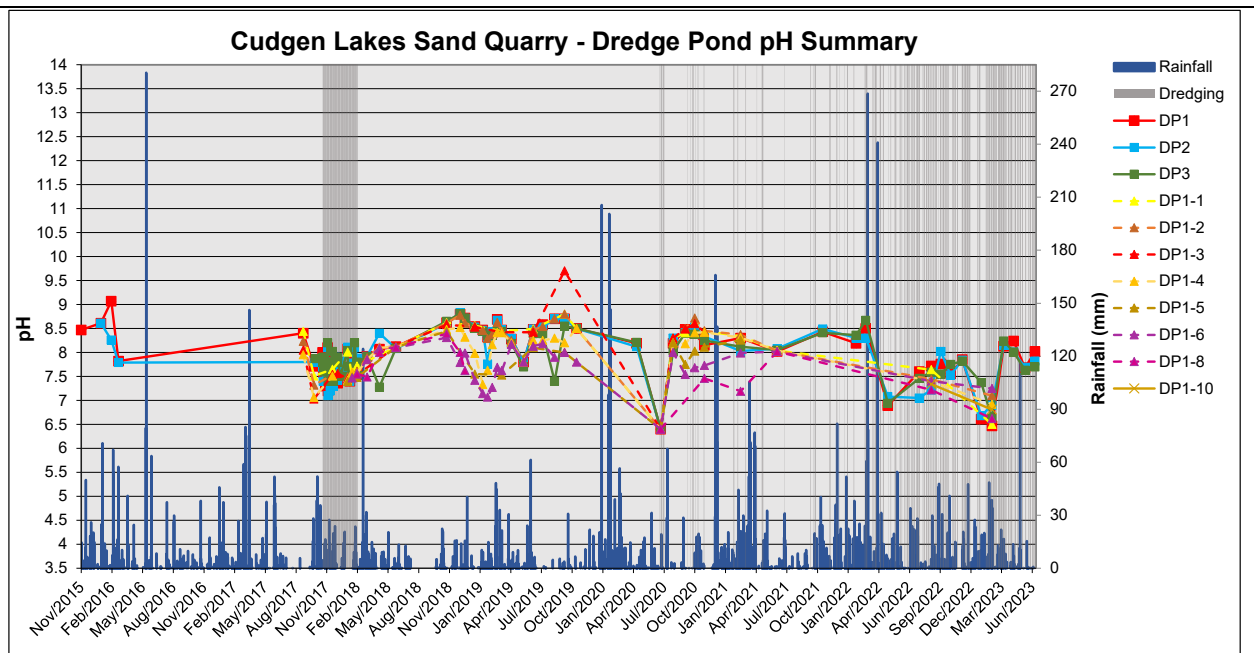
Figure 7.1 DREDGE POND pH SUMMARY
