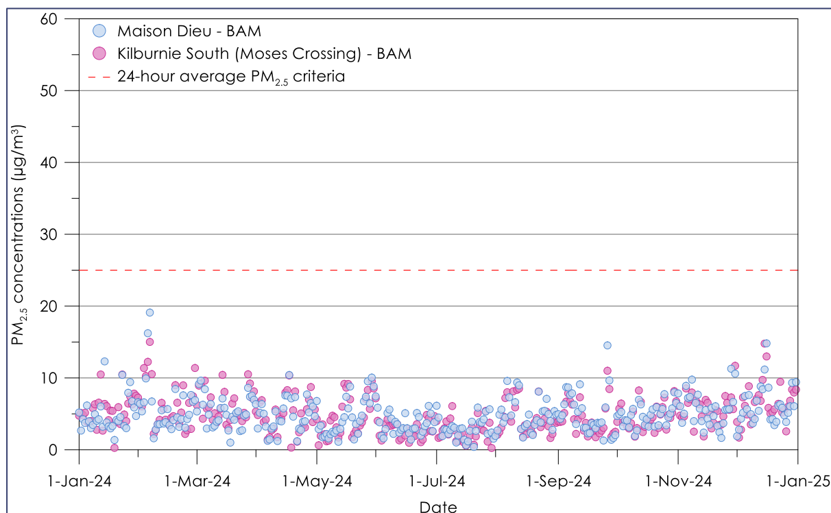
Figure 2-8: 24-hour average PM 2.5 BAM data
