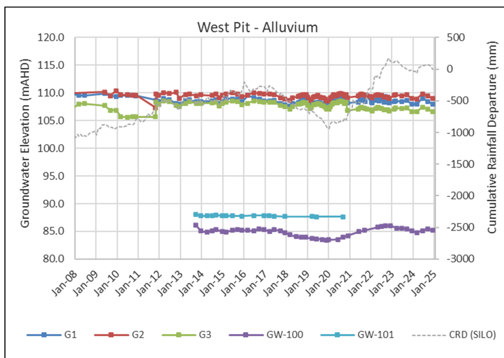
Figure 5.1 Groundwater Levels – West Pit Alluvium
