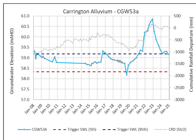
Figure 5.8 Groundwater Levels – CGW53a
