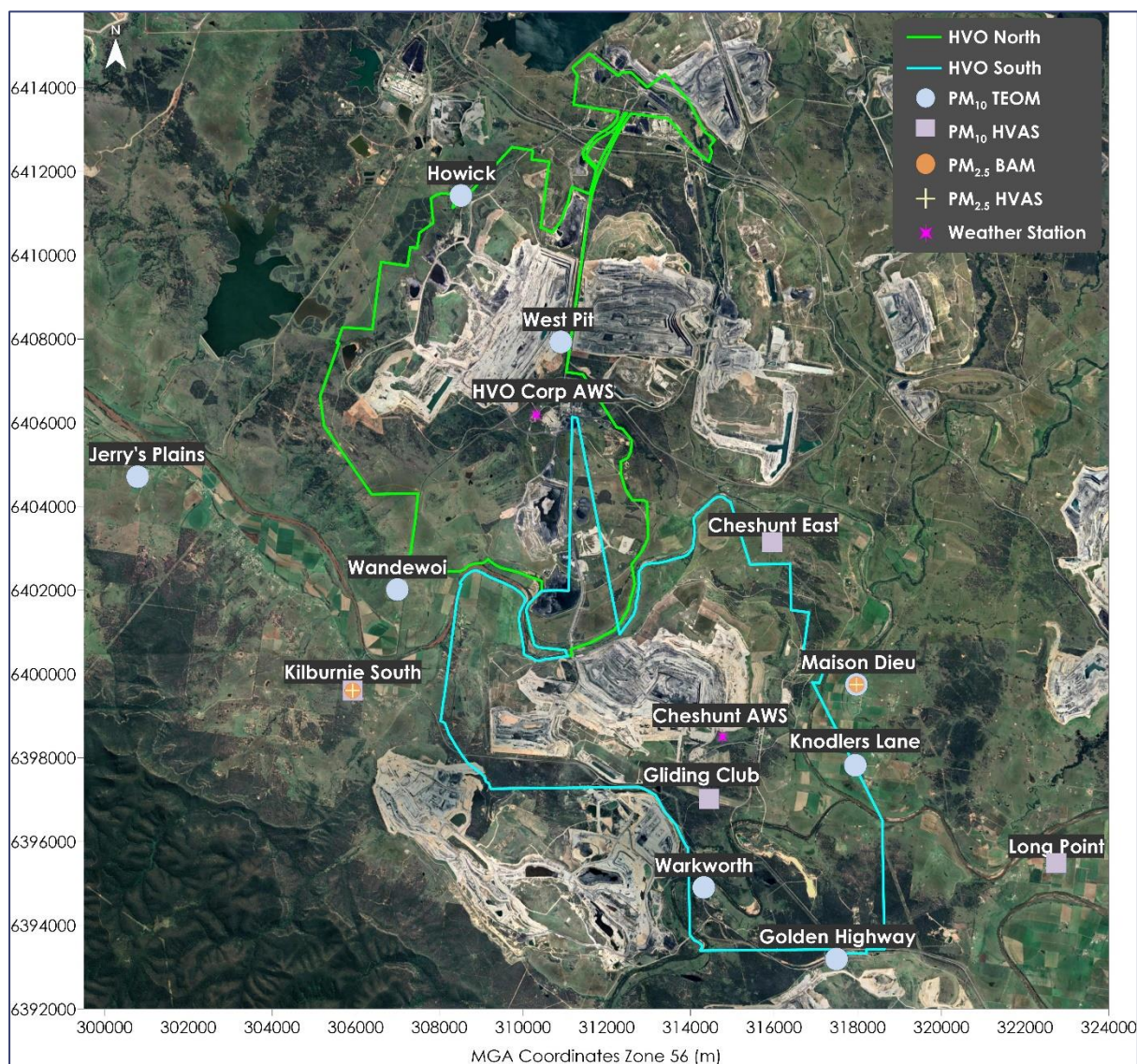
Figure 2-7: HVO PM 2.5 and PM 10 monitoring network
