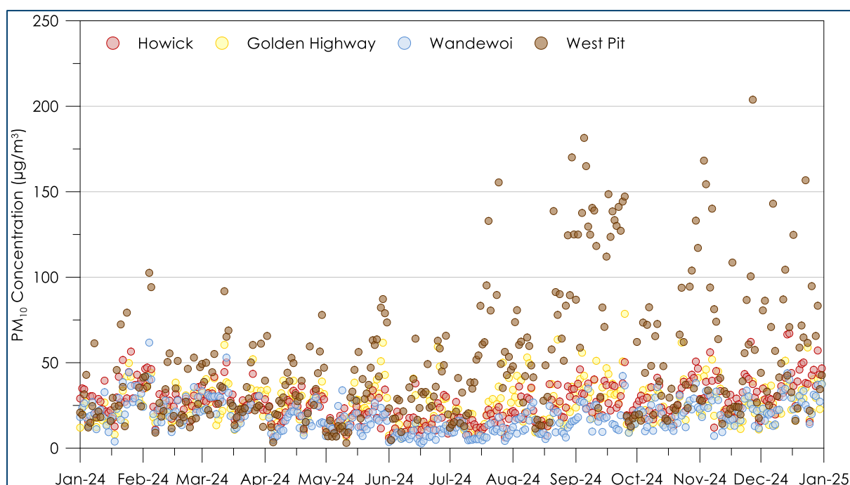
Figure 2-11: 24-hour average PM 10 TEOM results for 2024 – non-compliance monitors
