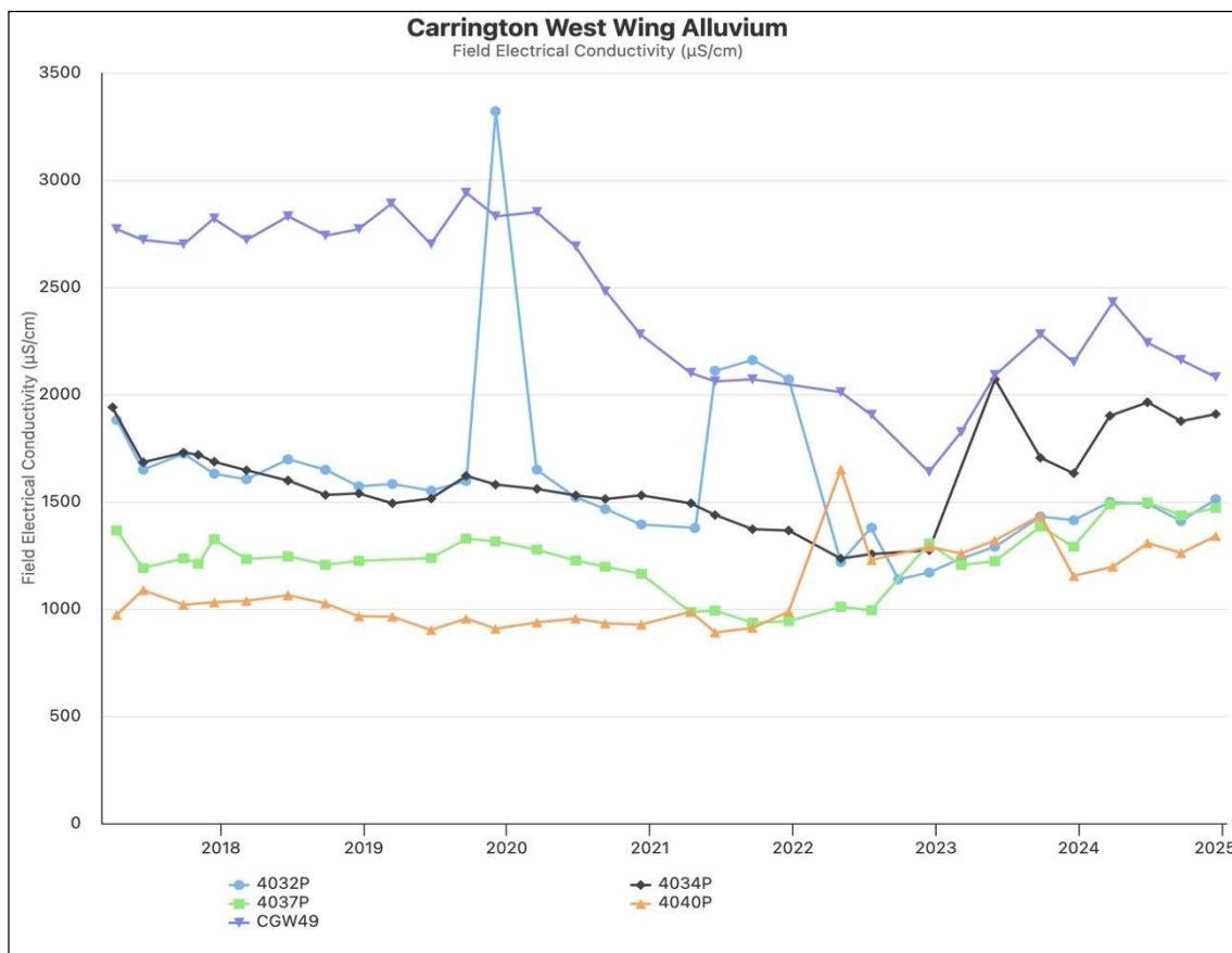
Figure 7-29: Carrington West Wing Alluvium Groundwater EC Trends 2017 – 2024
