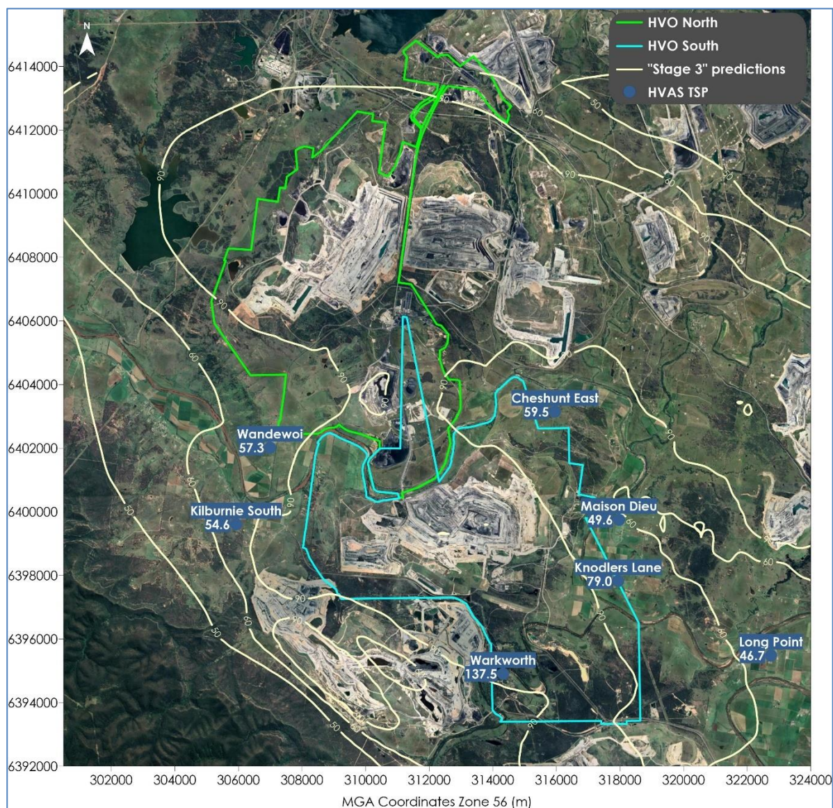
Figure 3-4: Annual average TSP monitoring data for 2024 superimposed over the predicted cumulative TSP annual average modelling contour (HVO plus other sources) (Source: Todoroski Air Sciences, 2017)
