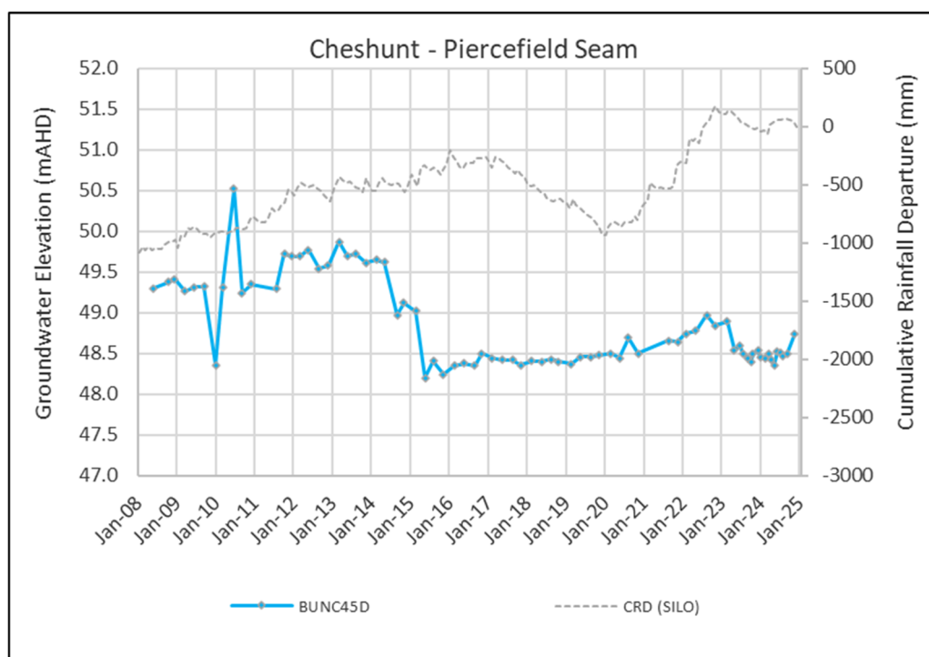
Figure 5.18 Groundwater Levels – Cheshunt Piercefield Seam
