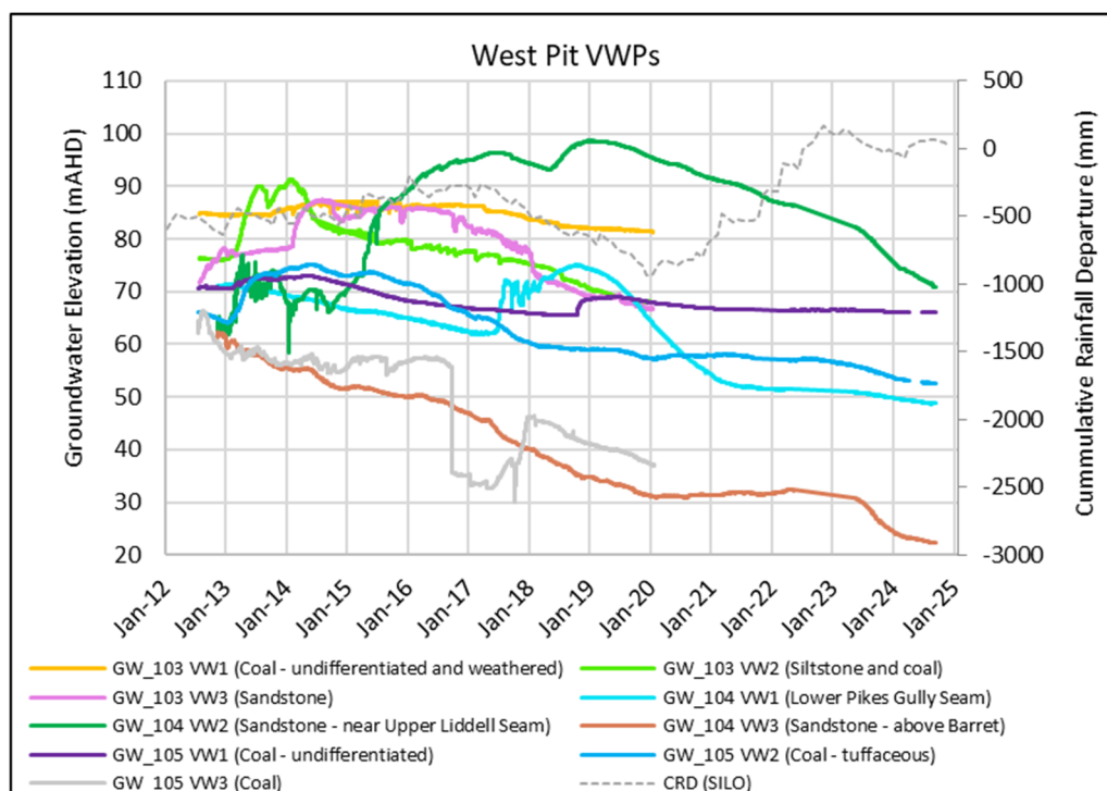
Figure 5.14 Groundwater Levels (VWPs) – West Pit Permian Coal Measures
