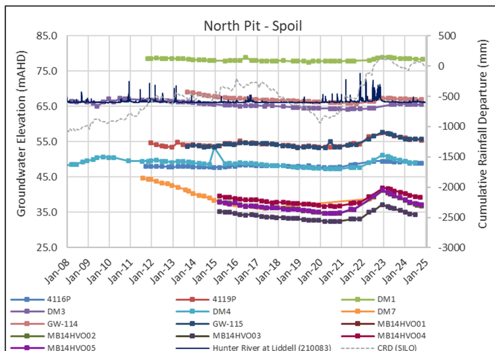
Figure 5.24 Groundwater Levels – North Pit Spoil
