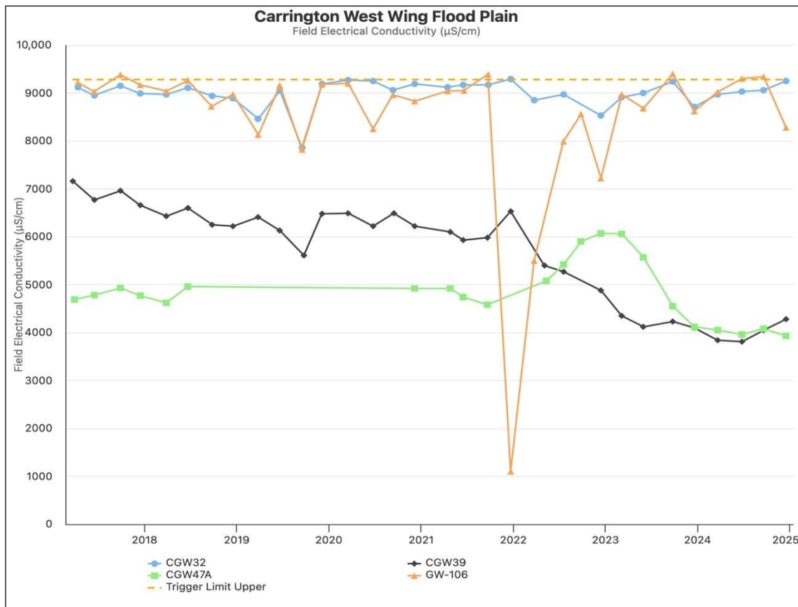
Figure 7-32: Carrington West Wing Flood Plain Groundwater EC Trends 2017 – 2024
