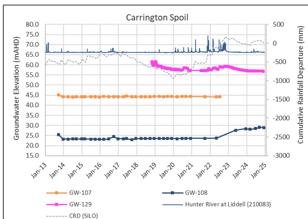
Figure 5.25 Groundwater Levels – Carrington Spoil
