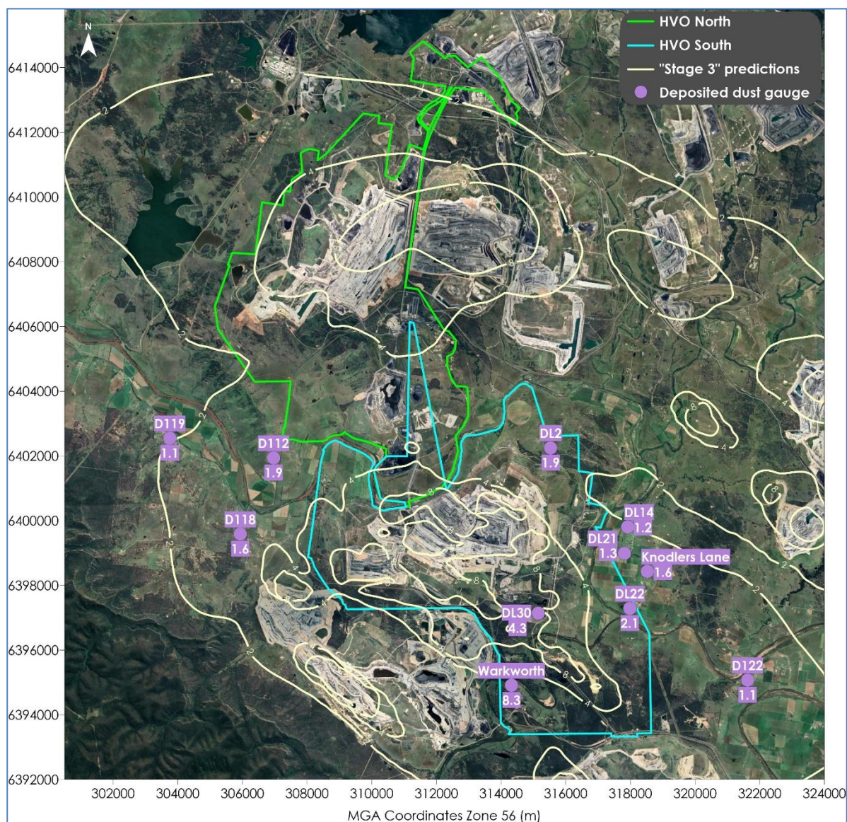
Figure 3-1: Annual average deposited dust monitoring data for 2024 superimposed over the predicted cumulative deposited dust annual average modelling contour (HVO plus other sources) (Source: Todoroski Air Sciences, 2017).
