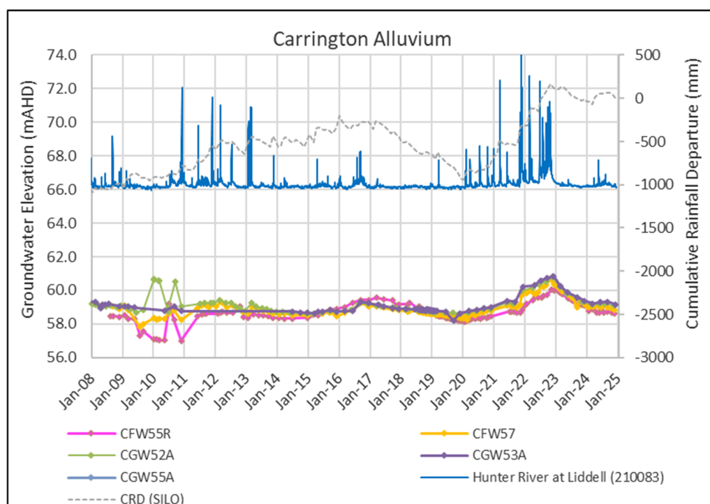
Figure 5.4 Groundwater Levels – Carrington Alluvium
