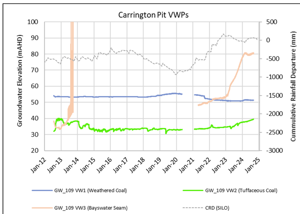
Figure 5.16 Groundwater Levels (VWPs) – Carrington Permian Coal Measures
