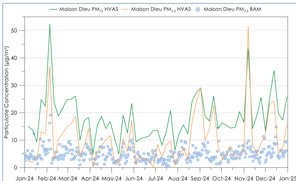
Figure 2-5: Maison Dieu PM 2.5 and PM 10 HVAS and BAM data in 2024
