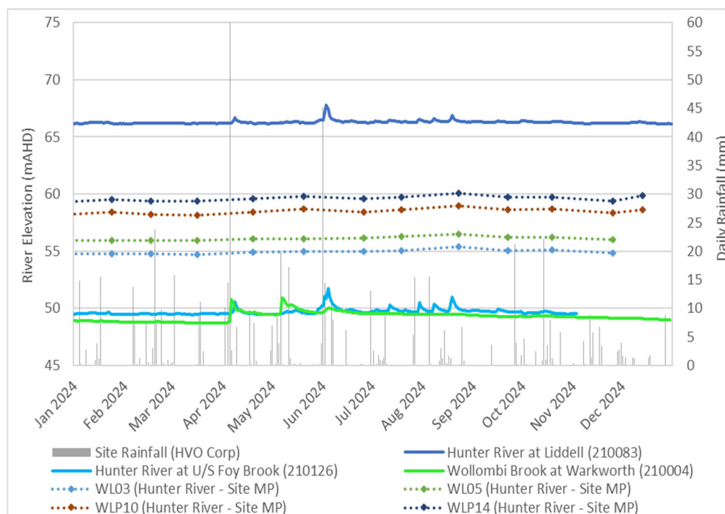
Figure 3.3 Surface Water Levels
