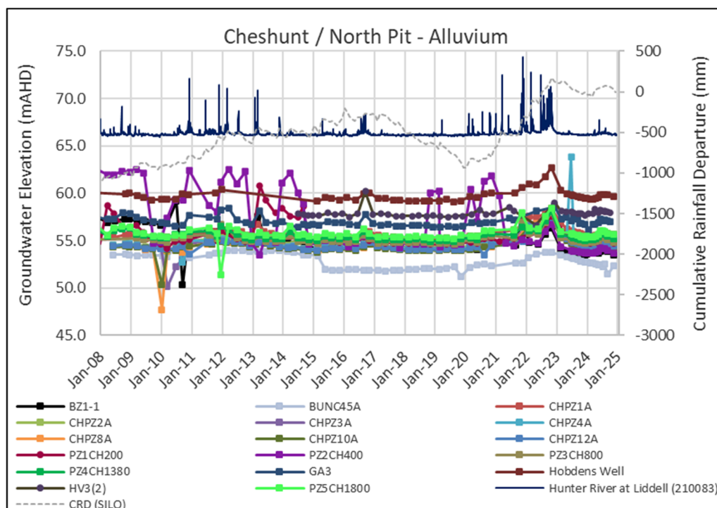
Figure 5.10 Groundwater Levels – Cheshunt/North Pit Alluvium
