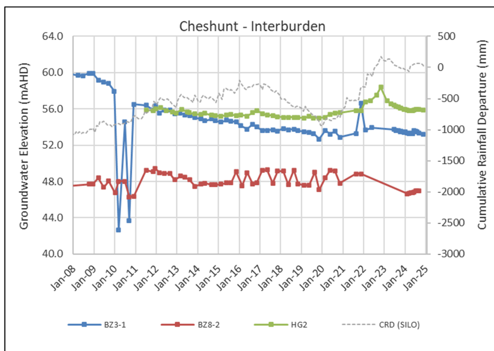
Figure 5.19 Groundwater Levels – Cheshunt Interburden
