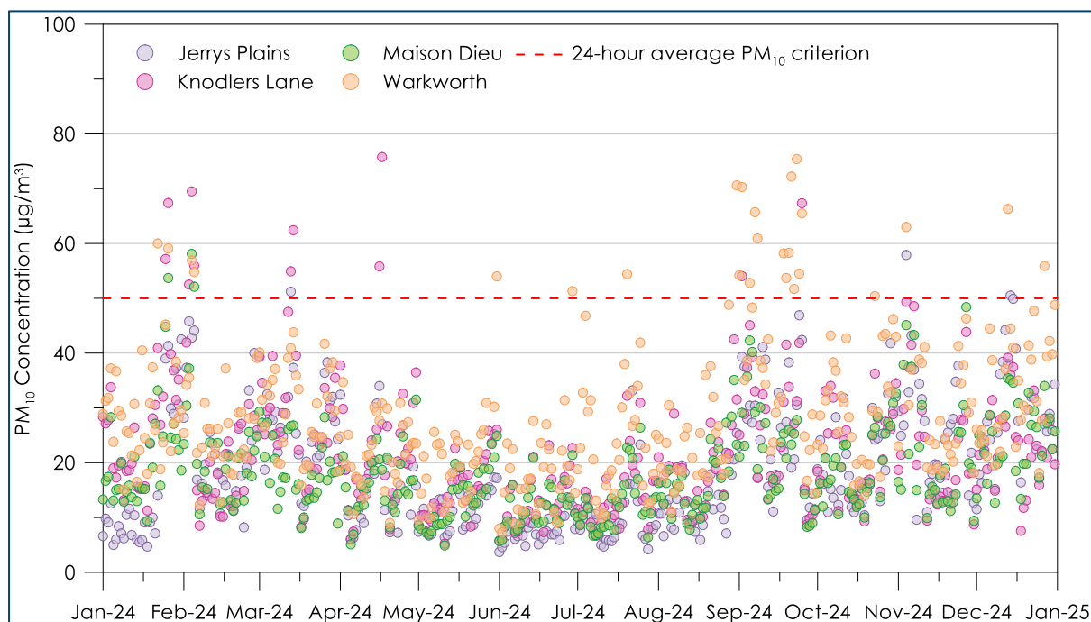
Figure 2-10: 24-hour average PM 10 TEOM results for 2024 – compliance monitors
