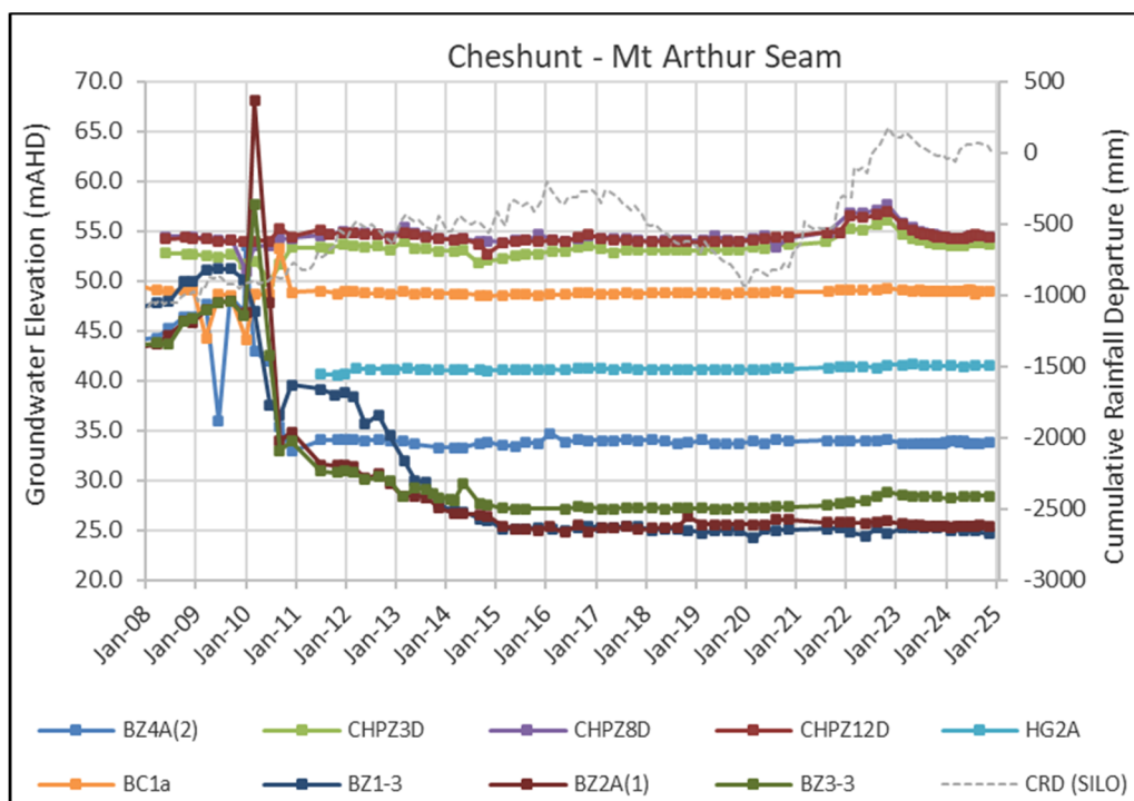
Figure 5.17 Groundwater Levels – Cheshunt Mt Arthur Seam
