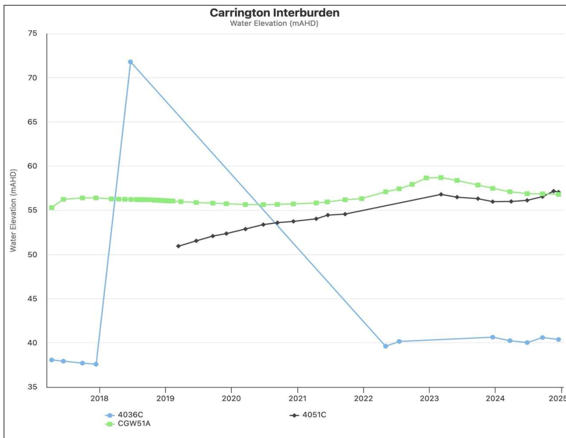
Figure 7-27: Carrington Interburden Groundwater SWL Trends 2017 - 2024
