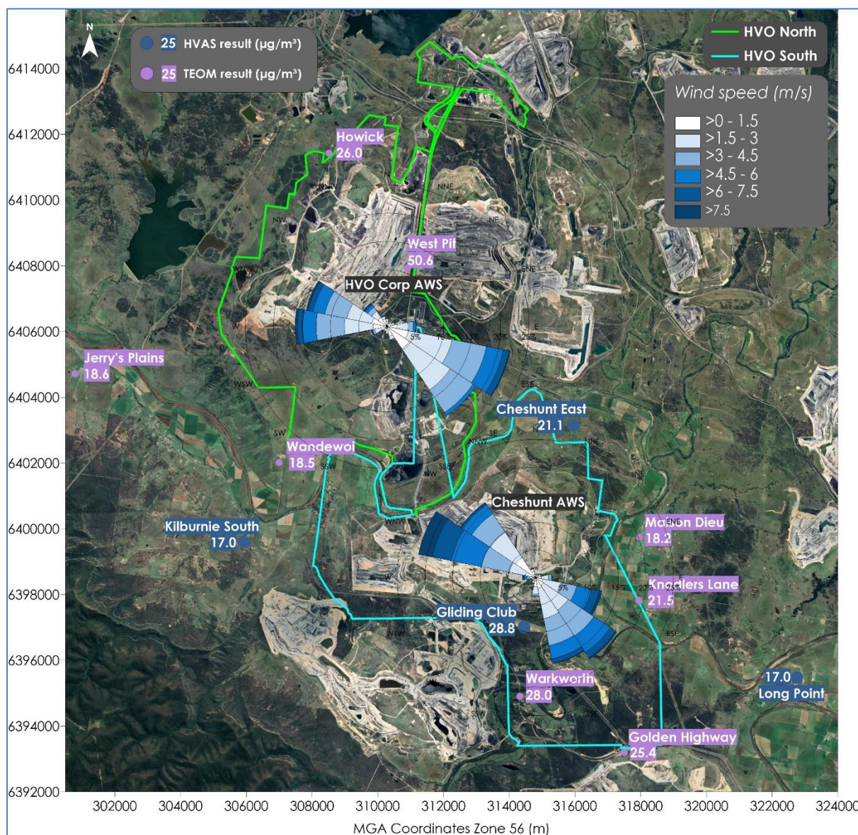
Figure 2-12: Annual average HVAS and TEOM PM 10 results for 2024
