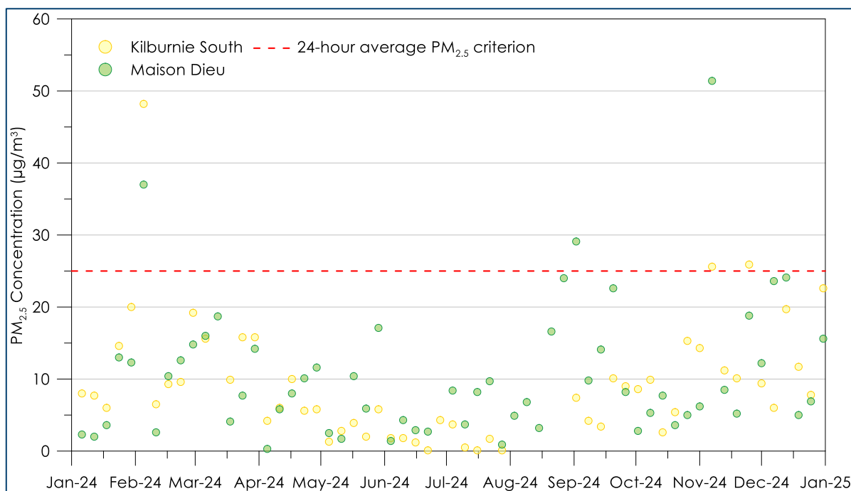
Figure 2-3: Kilburnie South and Maison Dieu 24-hour average PM 2.5 HVAS results for 2024
