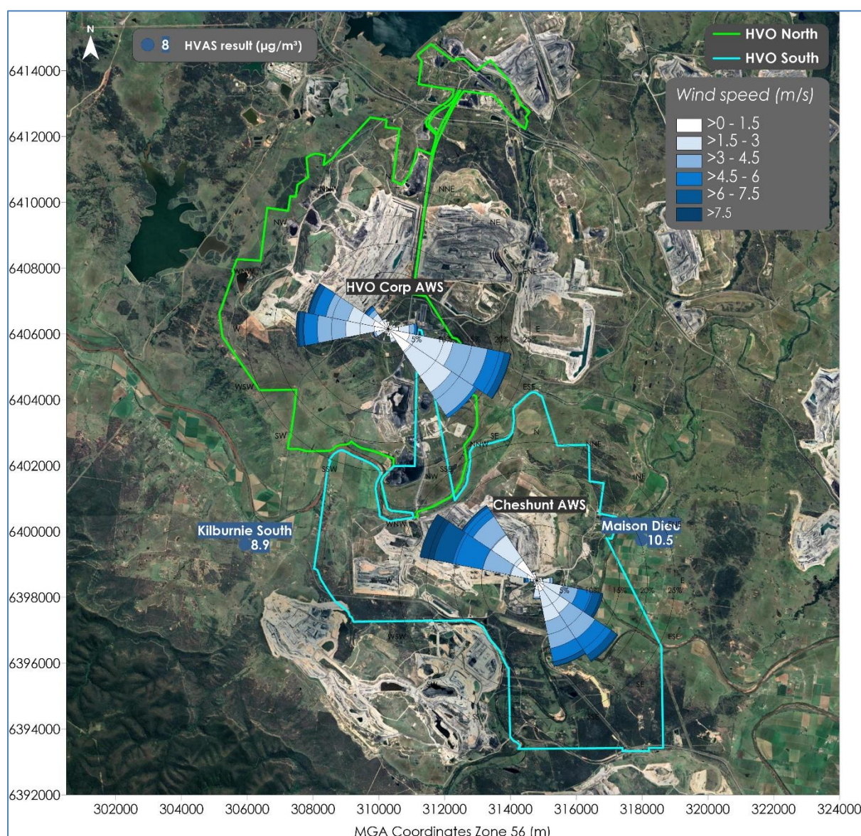
Figure 2-4: HVAS PM 2.5 results for 2024
