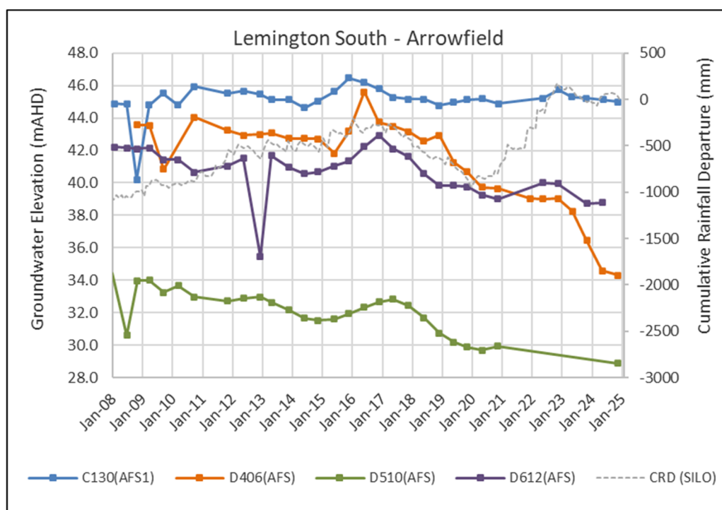
Figure 5.20 Groundwater Levels – Lemington South Arrowfield Seam
