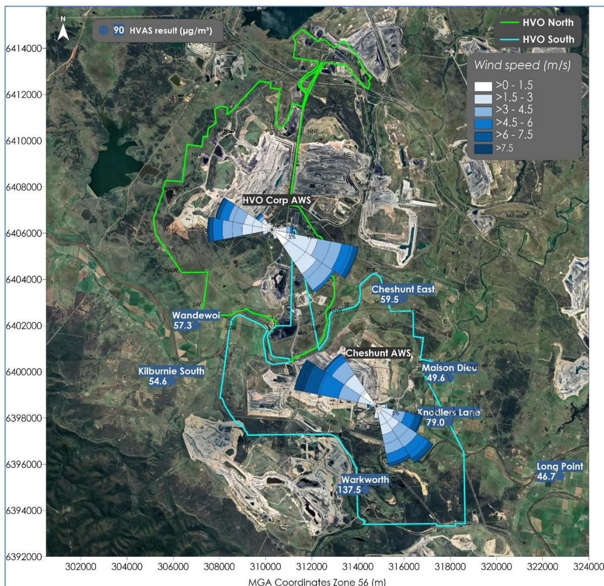
Figure 2-14: TSP HVAS results for 2024
