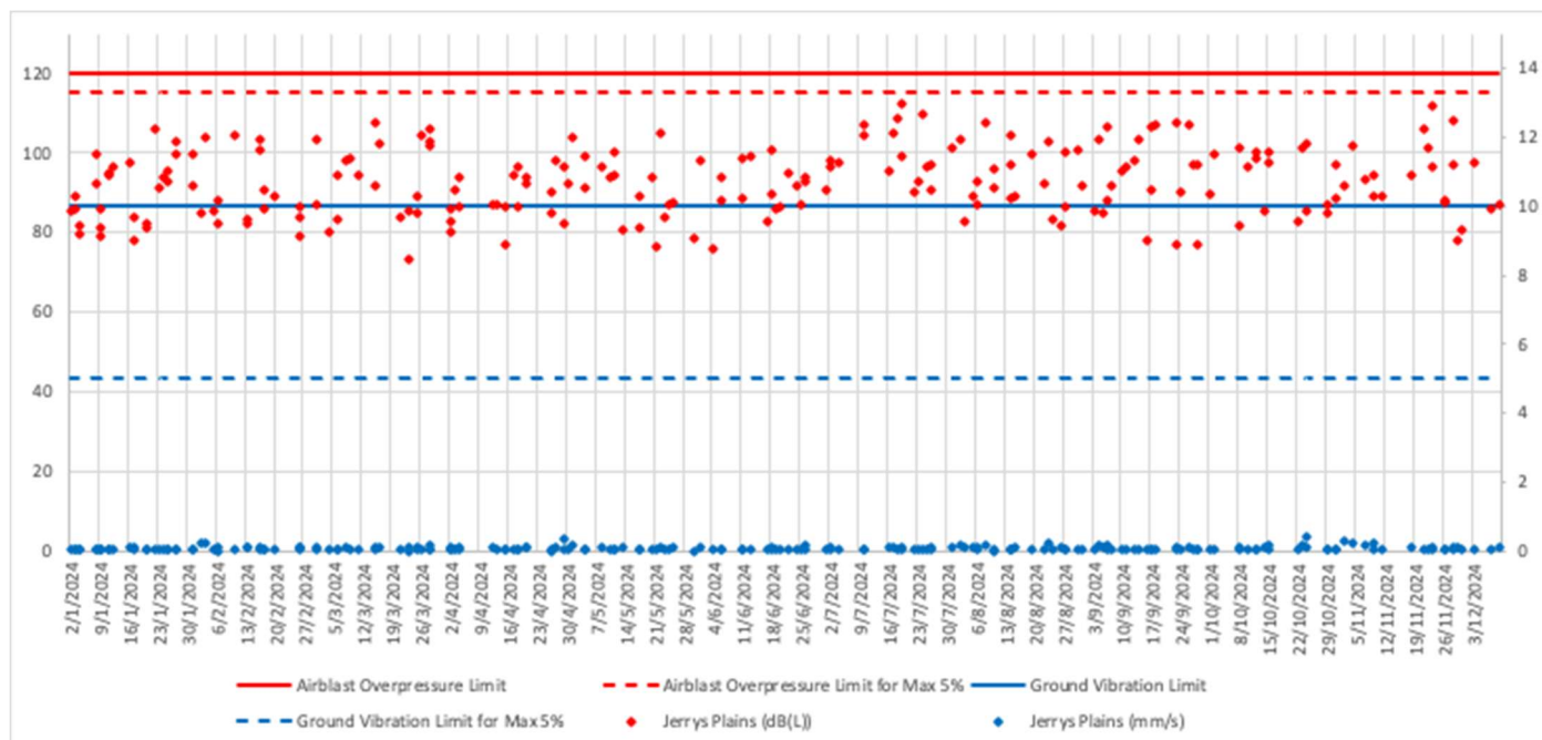
Figure 6-4: Jerrys Plains Blast Monitoring Results 2024
