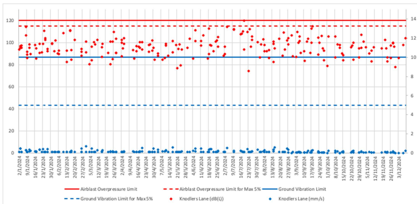
Figure 6-5: Knodlers Lane Blast Monitoring Results 2024
