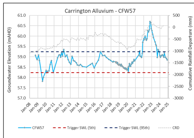
Figure 5.6 Groundwater Levels – CFW57
