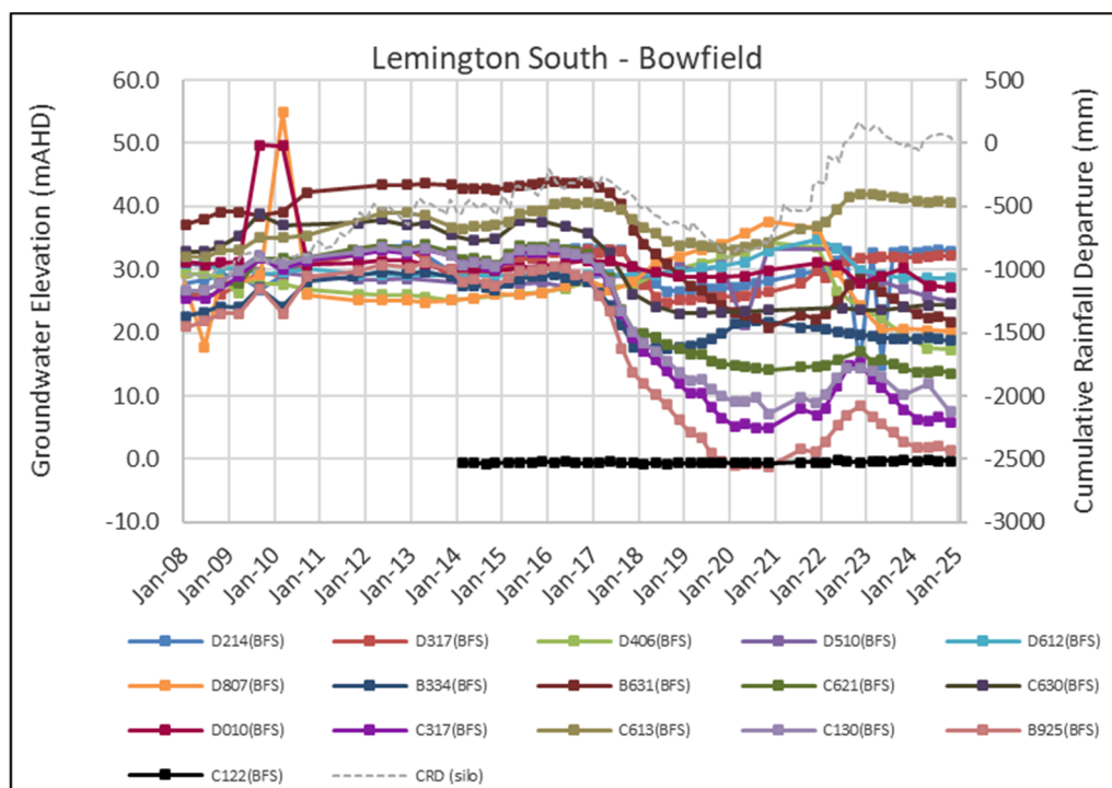
Figure 5.22 Groundwater Levels – Lemington South Bowfield Seam
