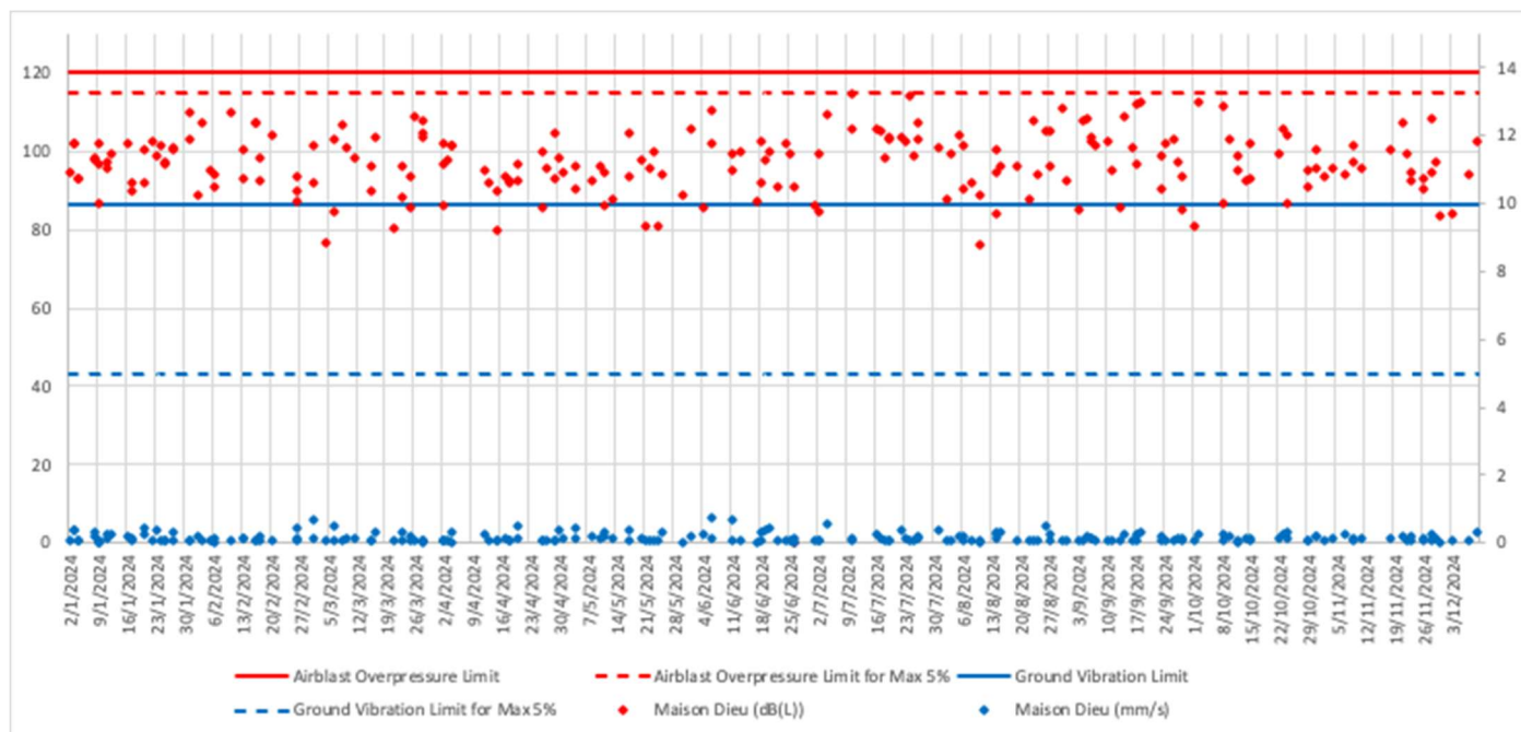
Figure 6-6: Maison Dieu Blast Monitoring Results 2024
