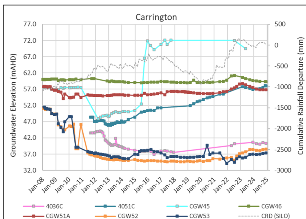
Figure 5.15 Groundwater Levels – Carrington Permian Coal Measures
