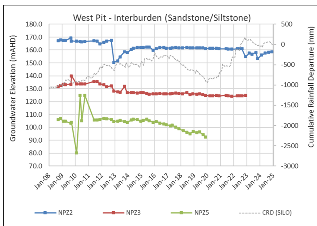
Figure 5.12 Groundwater Levels – West Pit Permian Coal Measures
