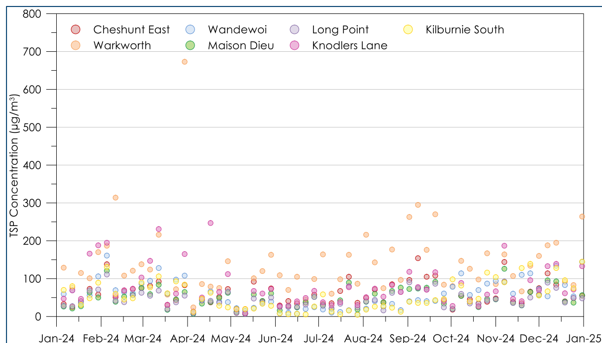
Figure 2-13: 24-hour average TSP HVAS results for 2024
