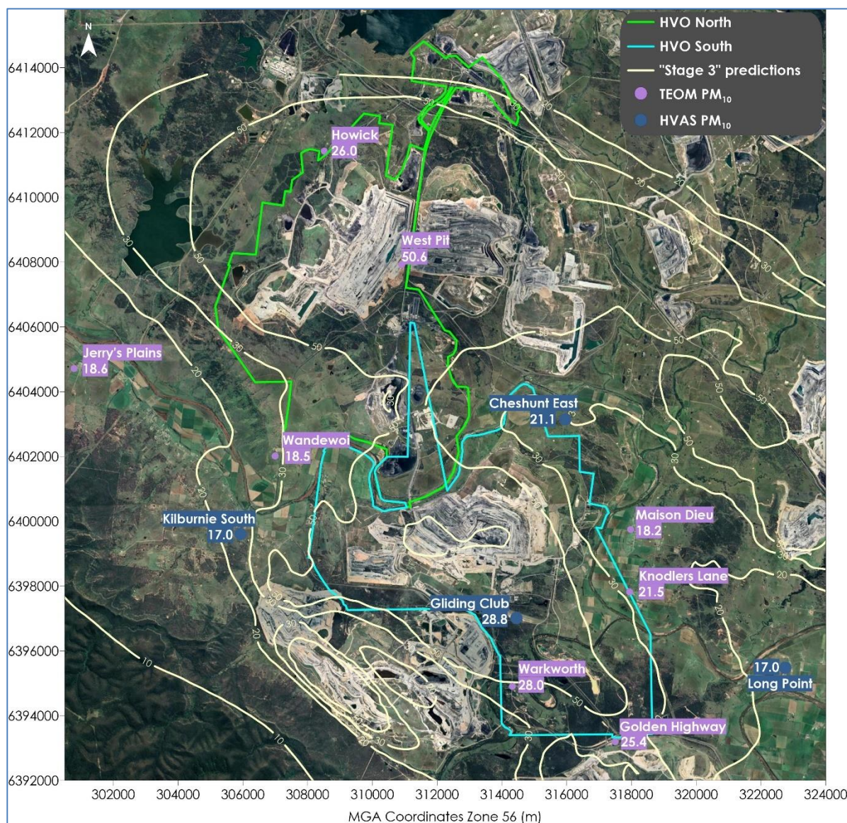
Figure 3-3: Annual average PM 10 monitoring data for 2024 superimposed over the predicted cumulative PM 10 annual average modelling contour (HVO plus other sources) (Source: Todoroski Air Sciences, 2017)
