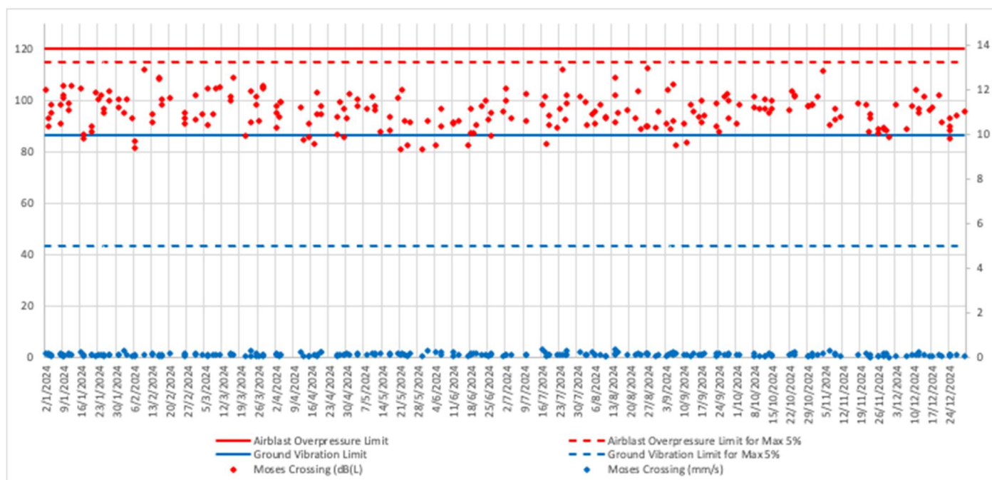
Figure 6-7: Moses Crossing Blast Monitoring Results 2024
