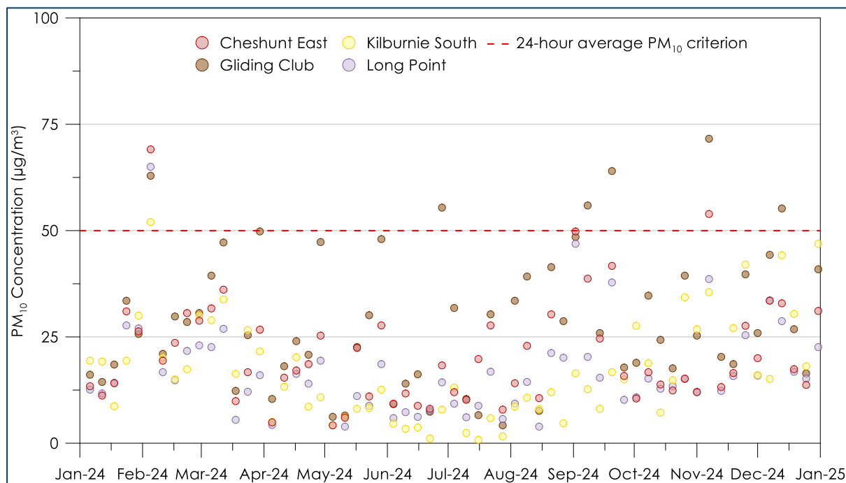
Figure 2-9: 24-hour average PM 10 HVAS results for 2024
