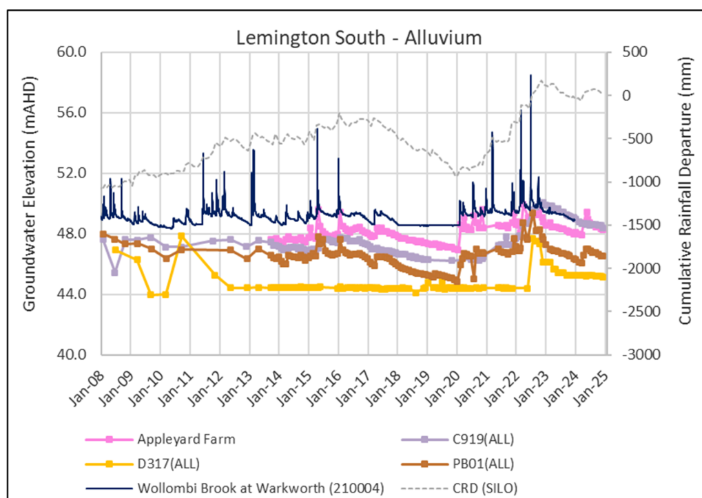
Figure 5.11 Groundwater Levels – Lemington South Alluvium
