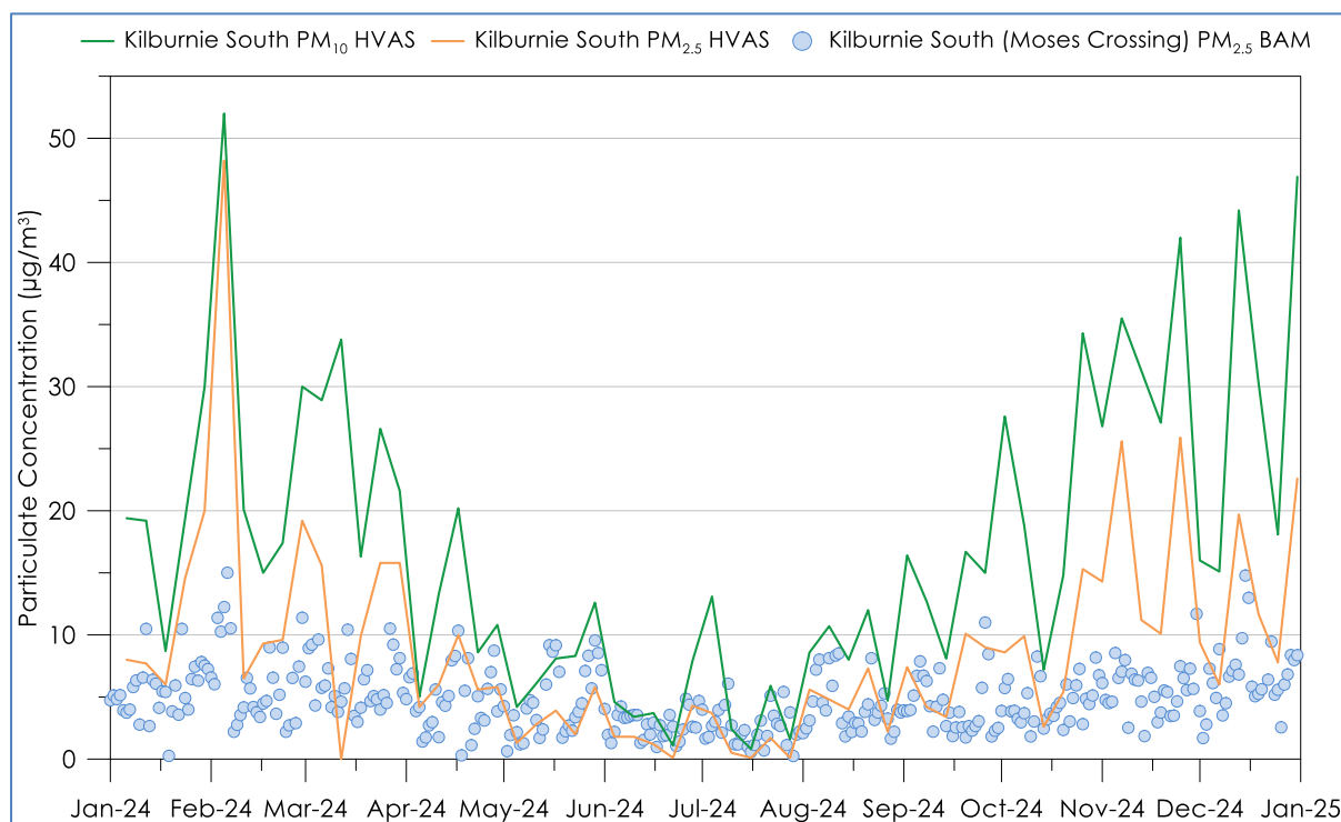
Figure 2-6: Kilburnie South PM 2.5 and PM 10 HVAS and BAM data in 2024
