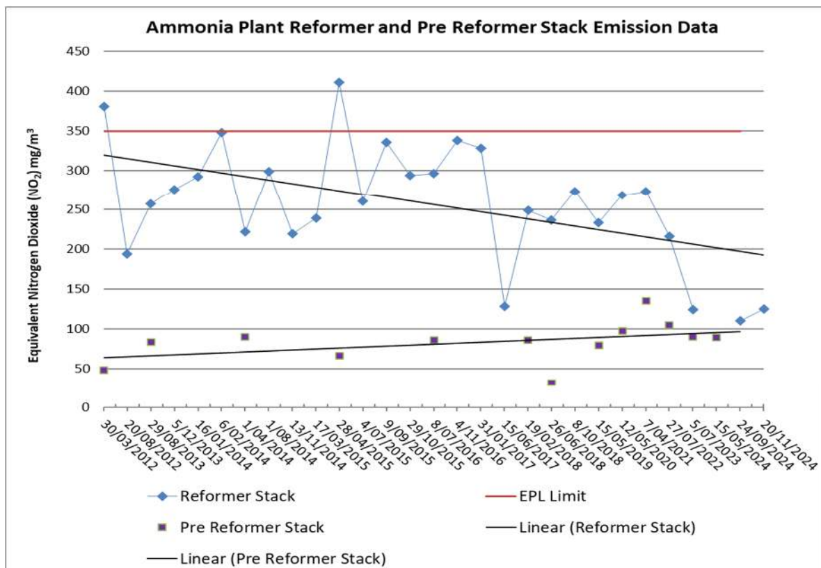
Figure 2 – Stack emission testing for ammonia plant
