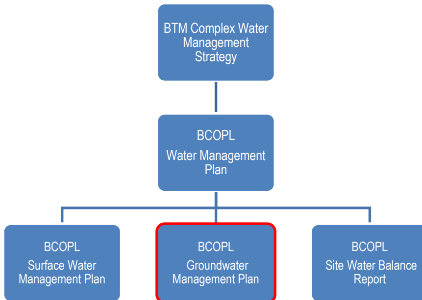
Figure 1-3: Document Hierarchy
