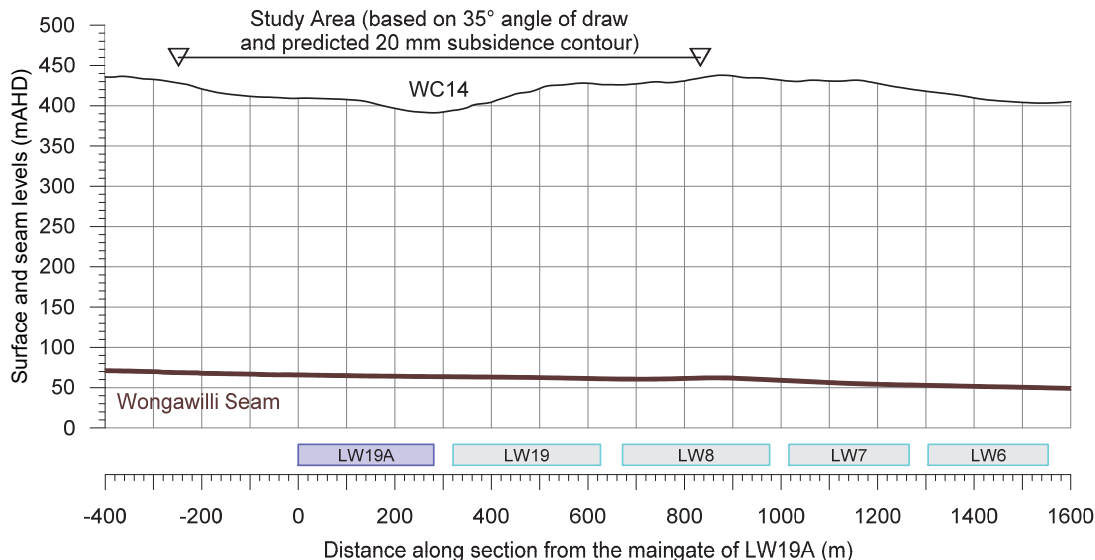
Fig. 1.2 Surface and seam levels along Section 1 (cross-section)
