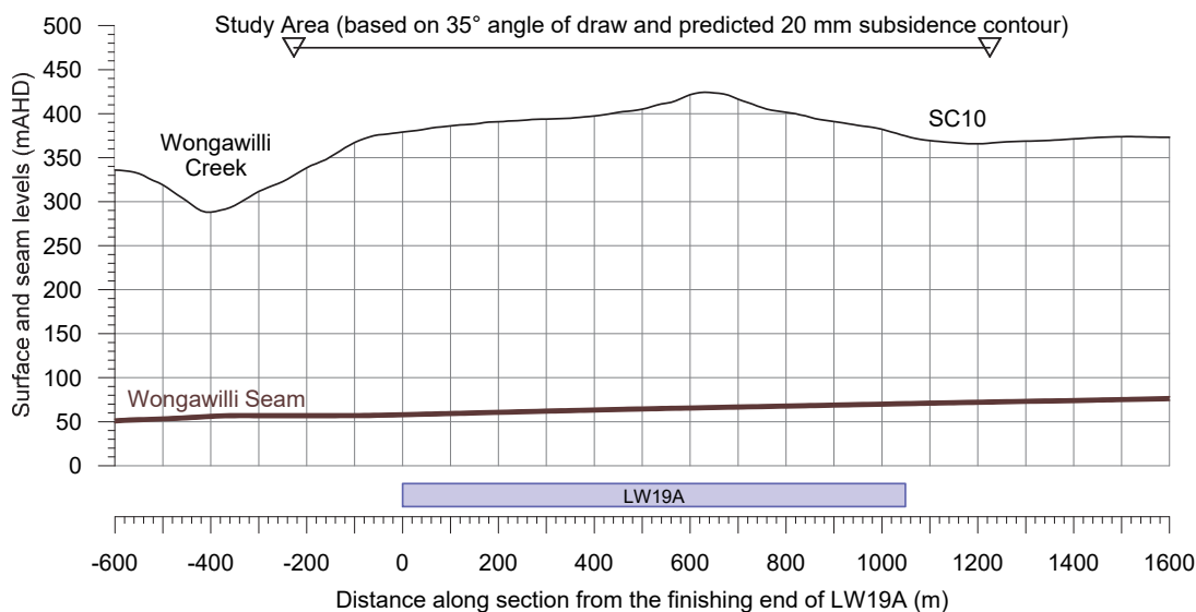
Fig. 1.3 Surface and seam levels along Section 2 (long-section)
