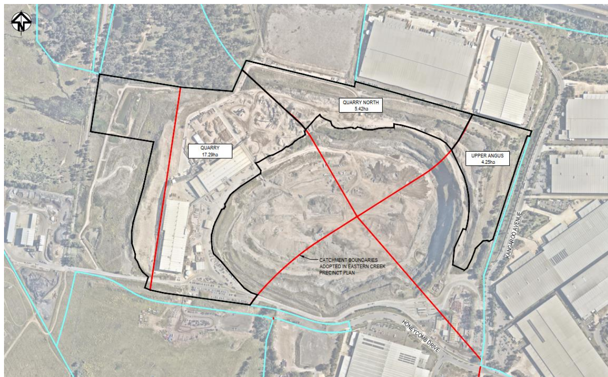
Figure 7: Stormwater catchment plan under pre-development conditions
