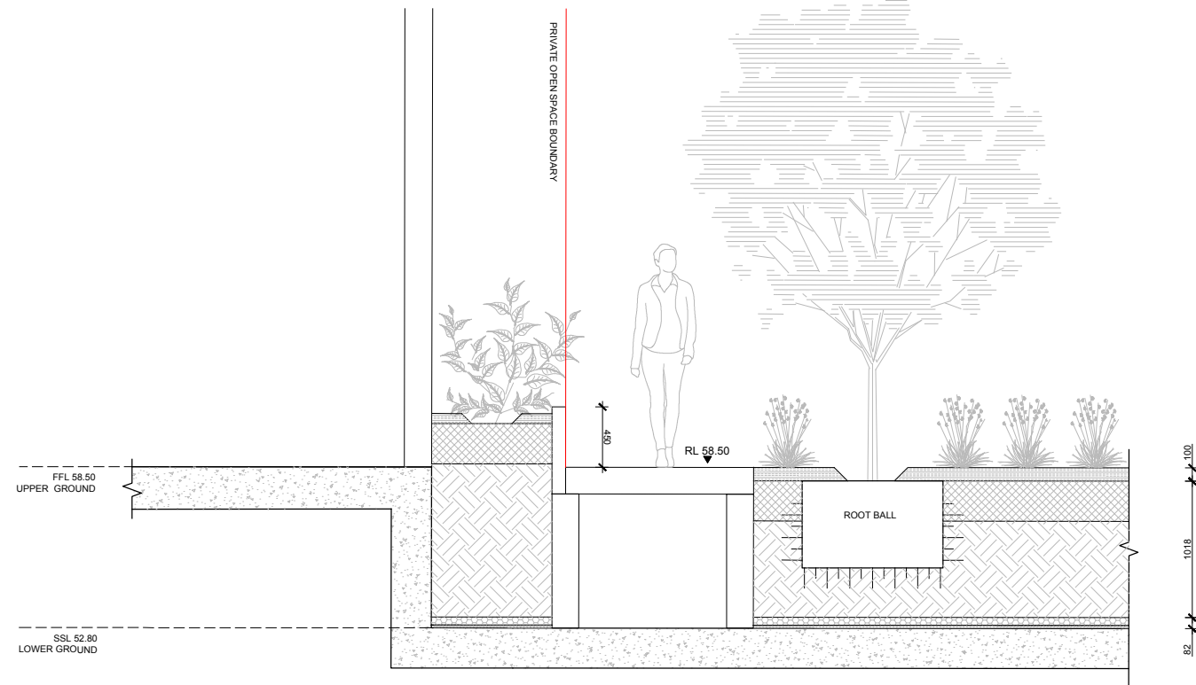
02 BUILDING E - EAST 1:50@A1
