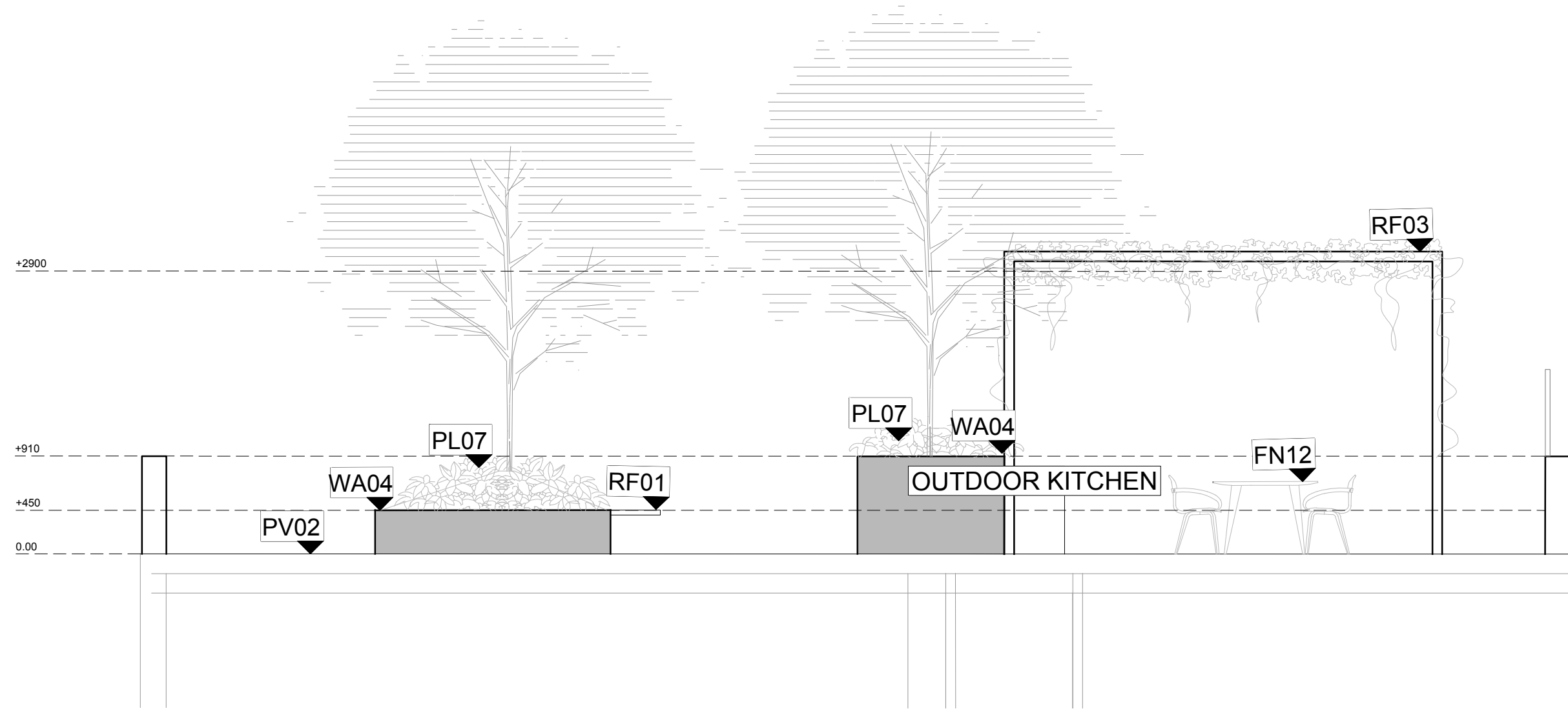
01 L_1801 COMMUNAL ROOF TERRACE - STAGE 1 1:50@A1
