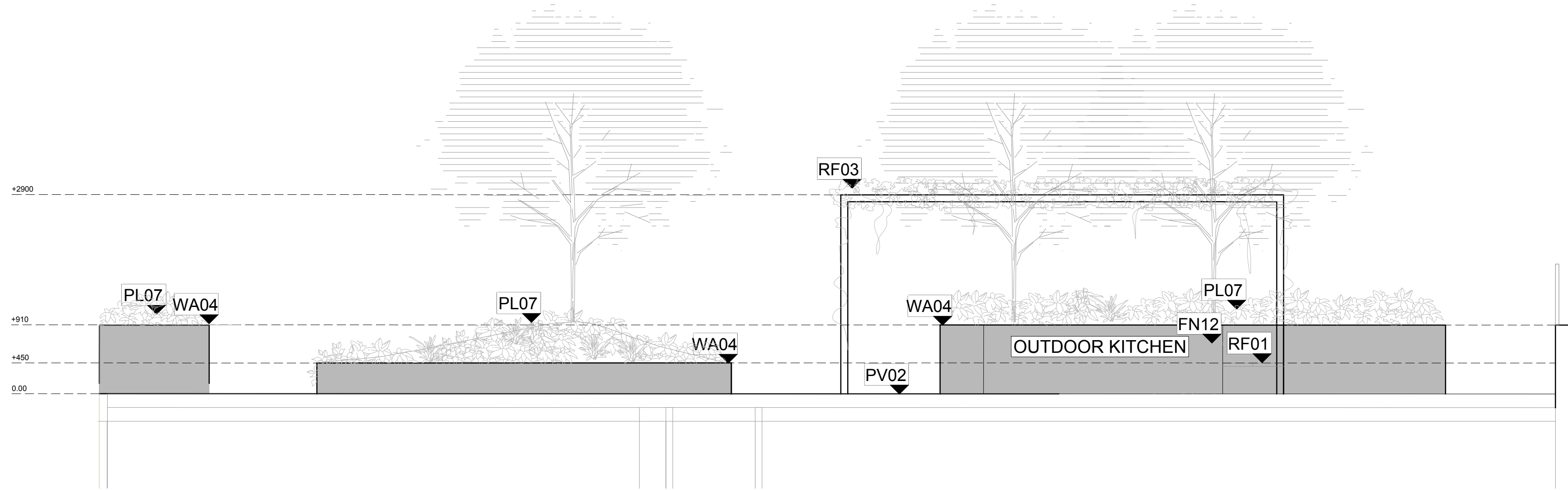
02 L_1801 COMMUNAL ROOF TERRACE - STAGE 1 1:50@A1
