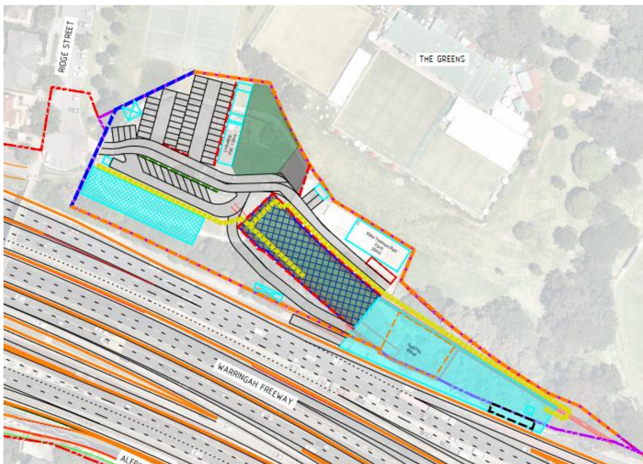
Figure 3 Ridge street north construction support site layout and parking
