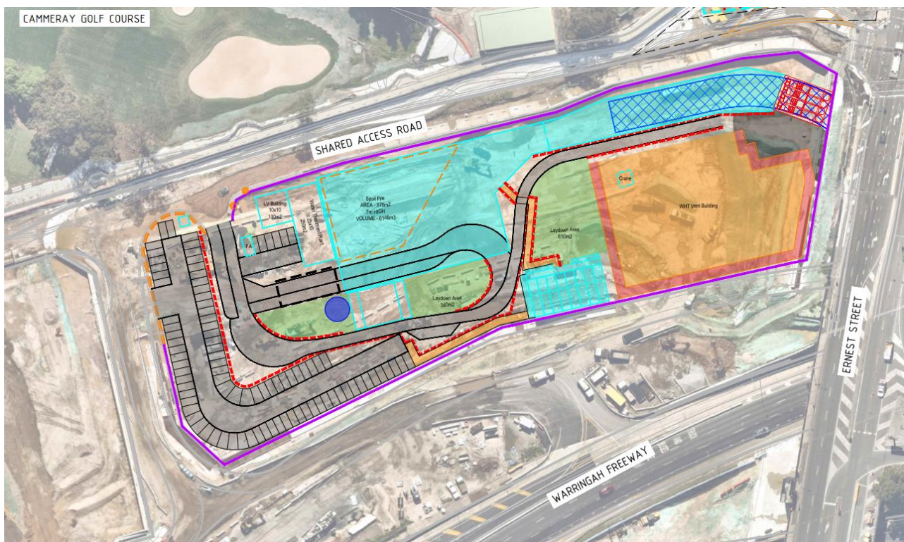
Figure 4 Cammeray construction site layout and parking
