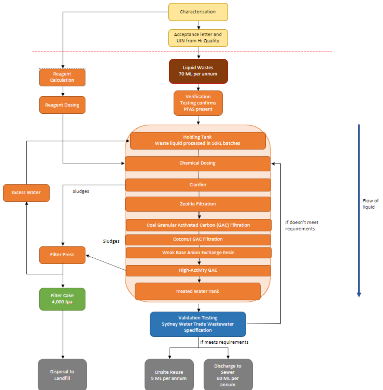
Figure 1-4 PFAS contaminated liquid waste process flow
