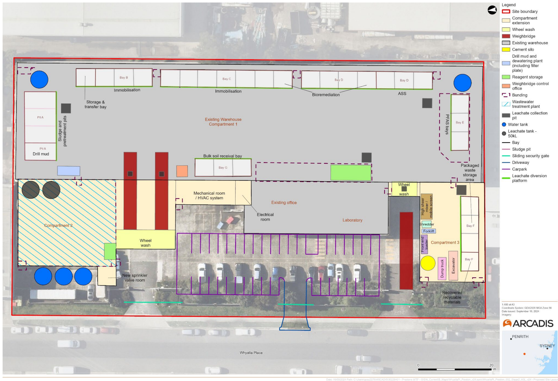
Figure 1-1 Facility layout
