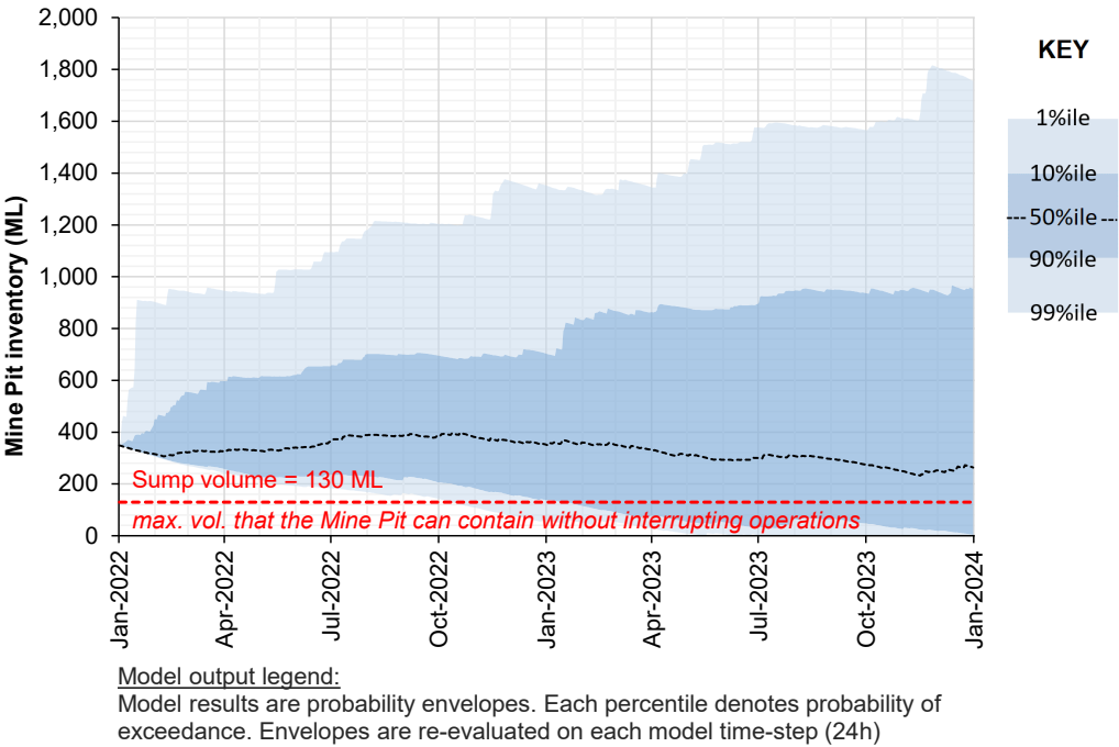
Figure 13 Predicted Annual Maximum Stored Water Volume in the Mine Pit
