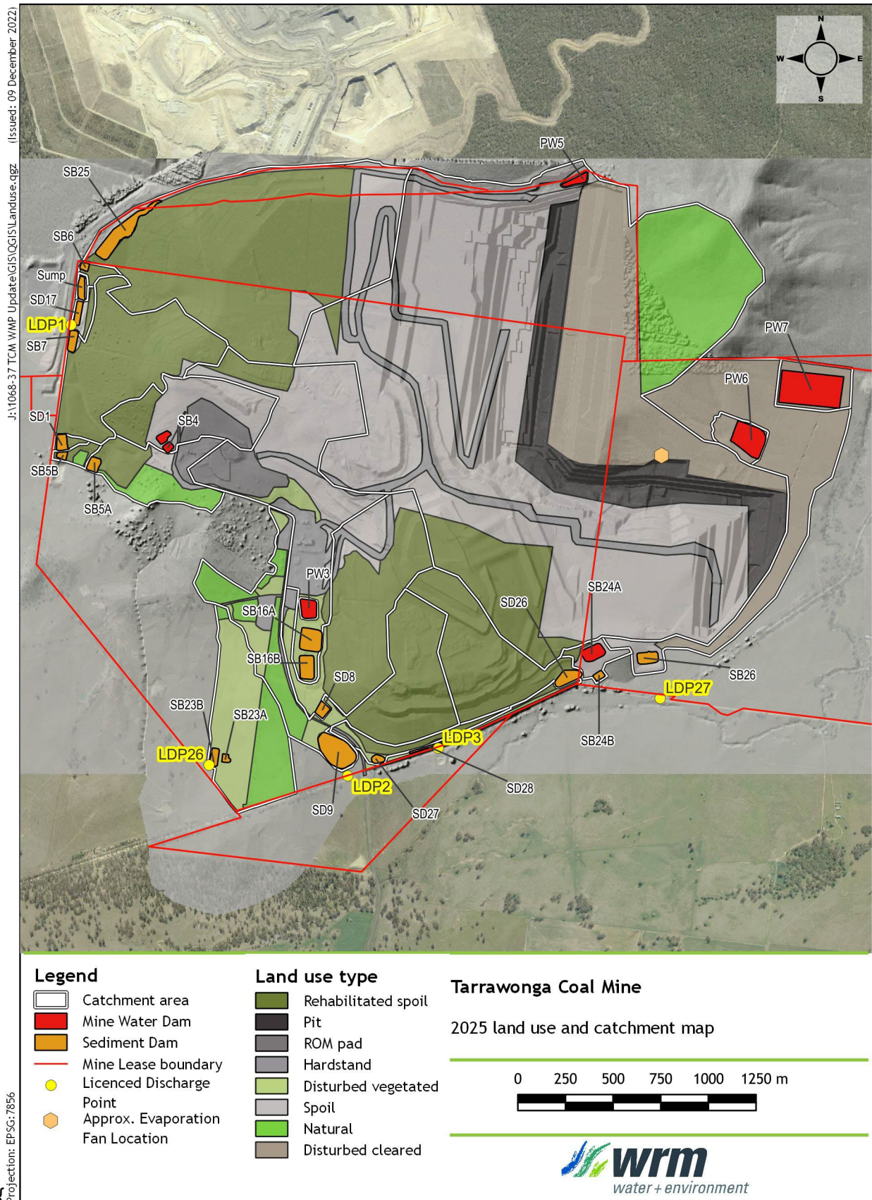
Figure 6 TCM Year 2025 Catchment Plan and Site Layout
