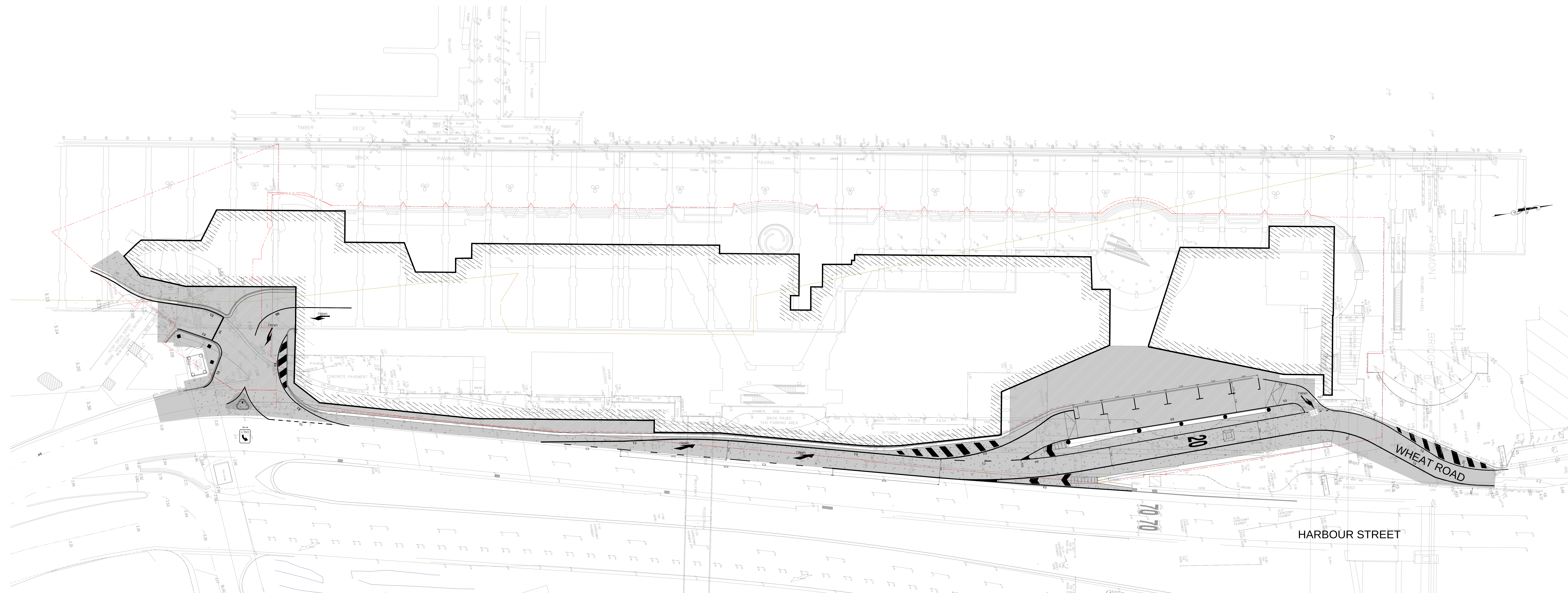
SITE WORKS - GROUND FLOOR - OVERALL PLAN
