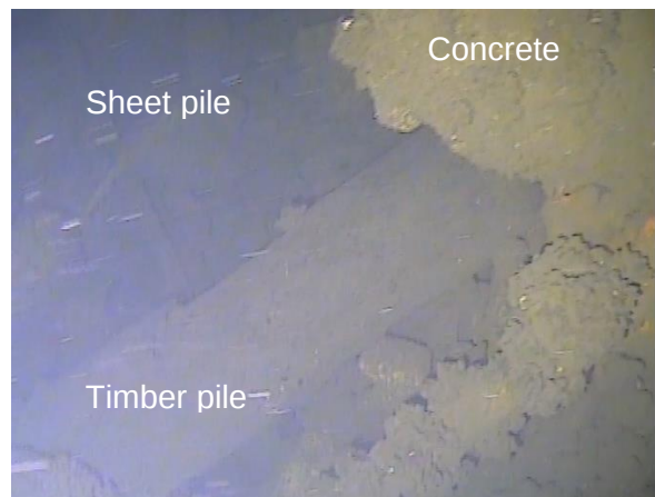
Figure 89: Horizontal timber pile on the northeast end of T7. (Image from T7 (b) Cockle Bay 210705; 03:38).
