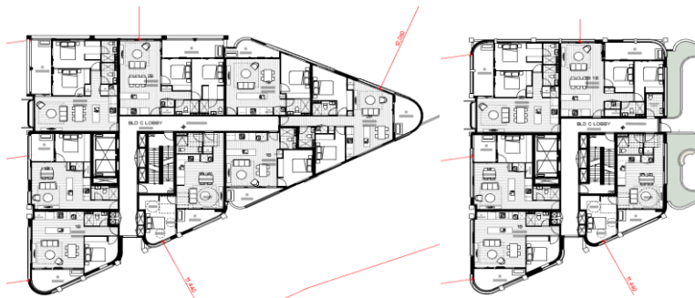
Fig.4.F2.1 Typical BLD C podium lobby with one opening (left), tower lobby with two openings (right)
