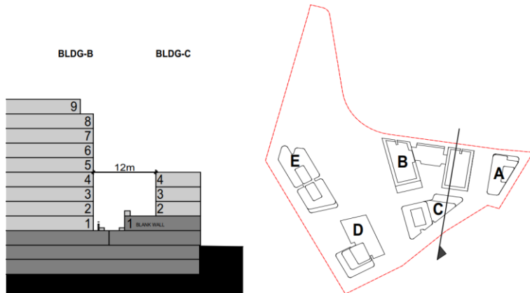
Fig. 3F1.2 Building B-C separation & Key Plan
