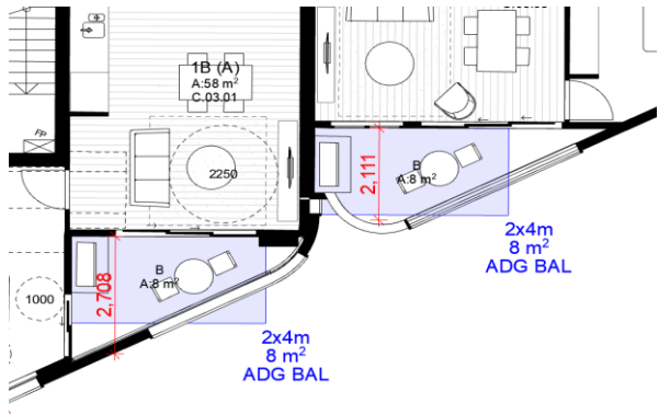
Fig.4E1.1 Irregular ear shaped balcony configuration
