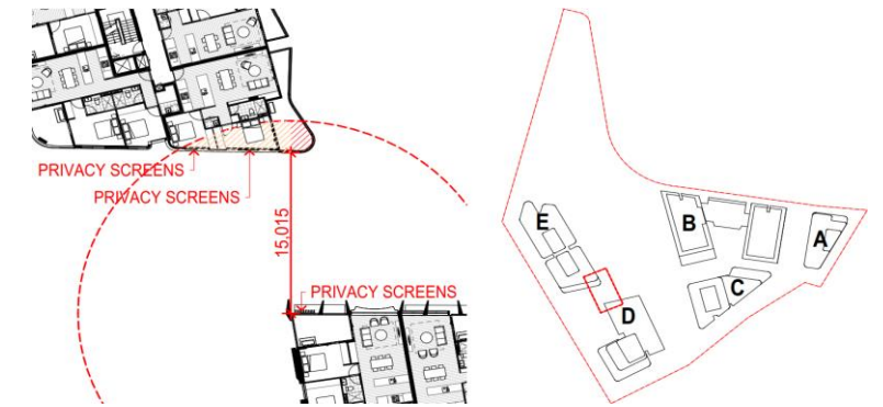
Fig. 3F1.2 Building D-E separation (storeys 3-9) & Key Plan (NTS)
