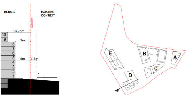
Fig. 3F1.6 Building D boundary condition & Key Plan
