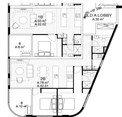
Fig.4E1.1 Typical 1Bed and 2bed balcony
