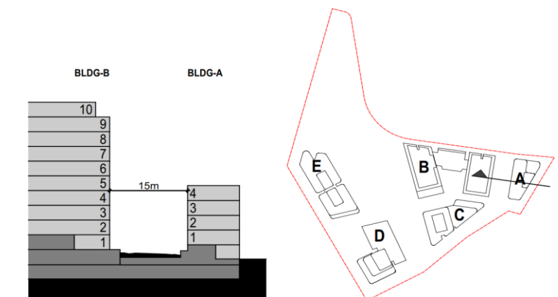
Fig. 3F1.1 Building A-B Section1 & Key Plan
