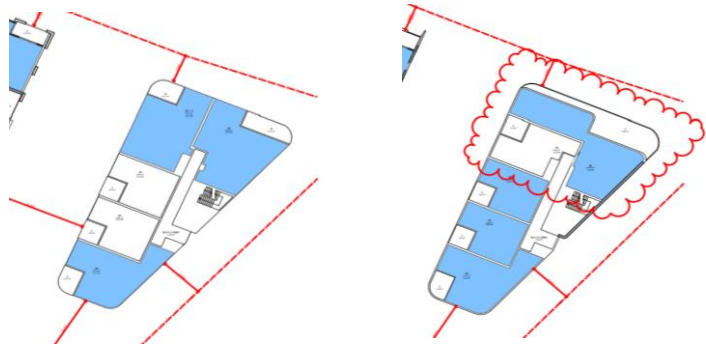
Fig.4A3.1 Cross Ventilation Diagram typical level (left) and top floor (right).
