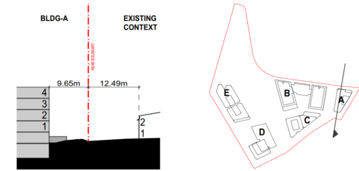
Fig. 3F1.5 Building A boundary condition & Key Plan The proposed BLD A seeks to maintain building separation for both privacy and acoustic purpose. In locations where ADG building separation could not be met, living room and private open space are located in such a way that direct lines of sight from other buildings on site are avoided.
