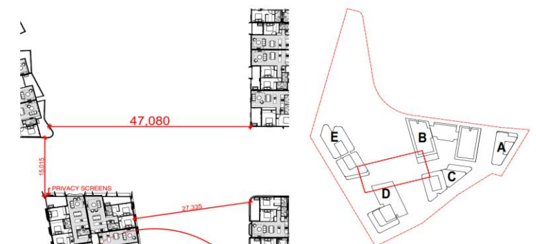
Fig. 3F1.7 Building B-E separation (storeys 1-9) & Key Plan
