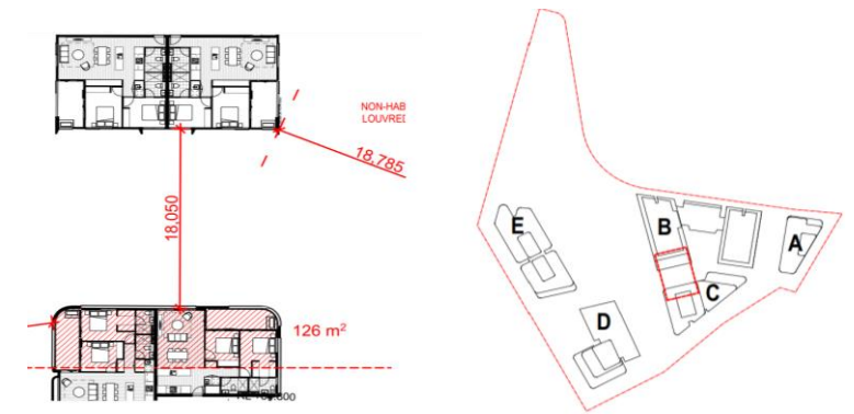
Fig. 3F1.3 Building C non-compliance (storey 9)
