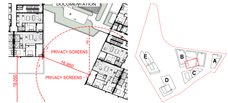
Fig. 3F1.5 Building B separation (storeys 5-8) & Key Plan
