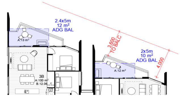
Fig.4E1.1 Typical triangular balcony where dimensions may not adhere exactly to ADG, objectives are still met.
