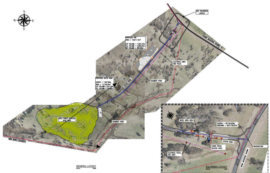
Figure 1: Proposed Rock Forest site location and layout
