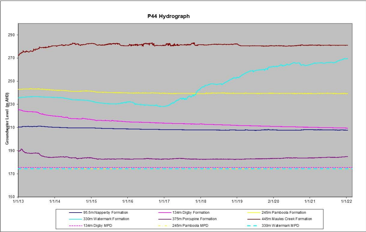
Figure C-22: Hydrograph for P44
