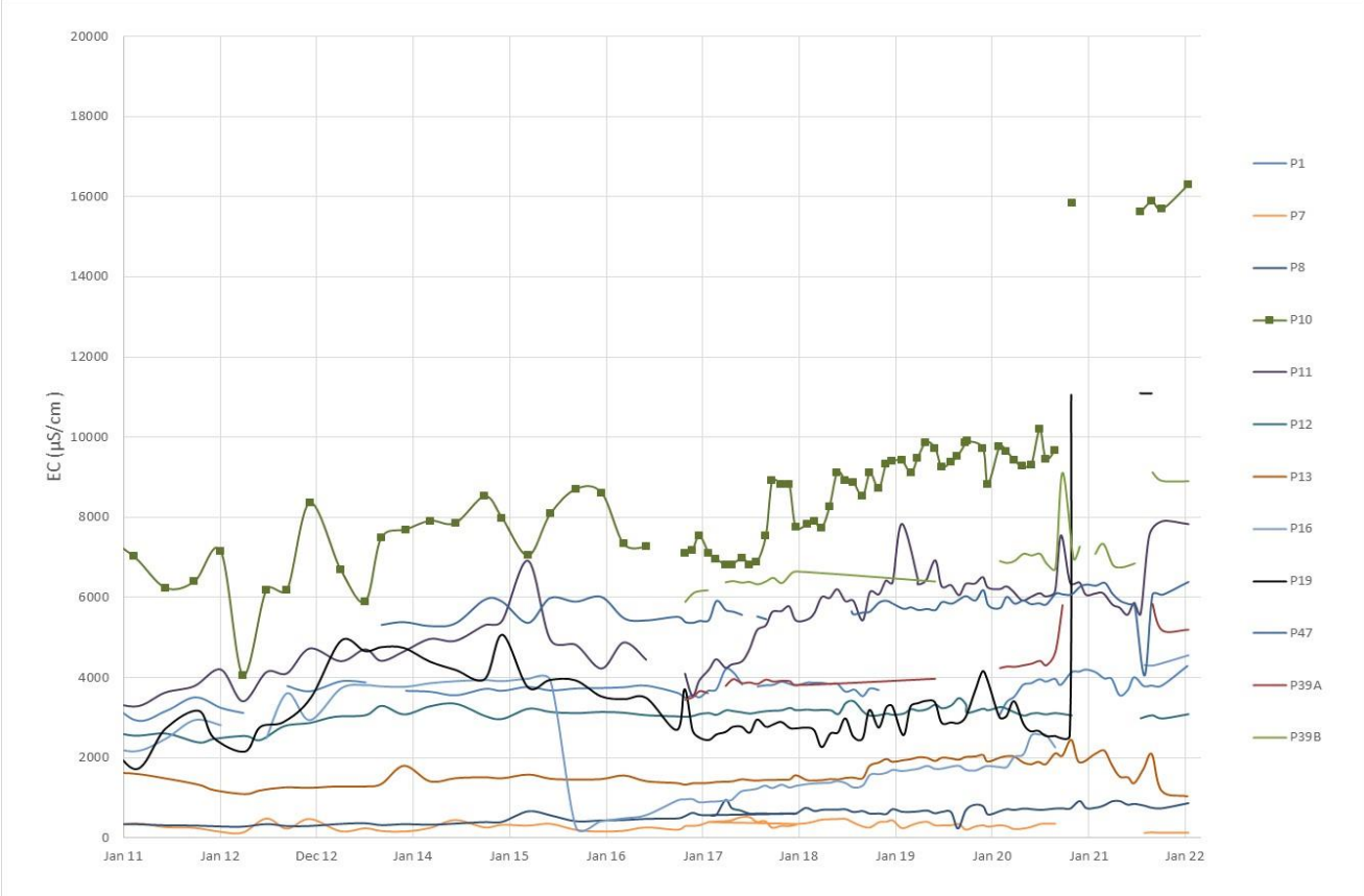
Figure C-36 Electrical Conductivity (EC) for Selected Deep Piezometers
