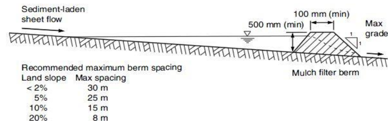
Figure 1 - Typical placement of mulch filter berm
