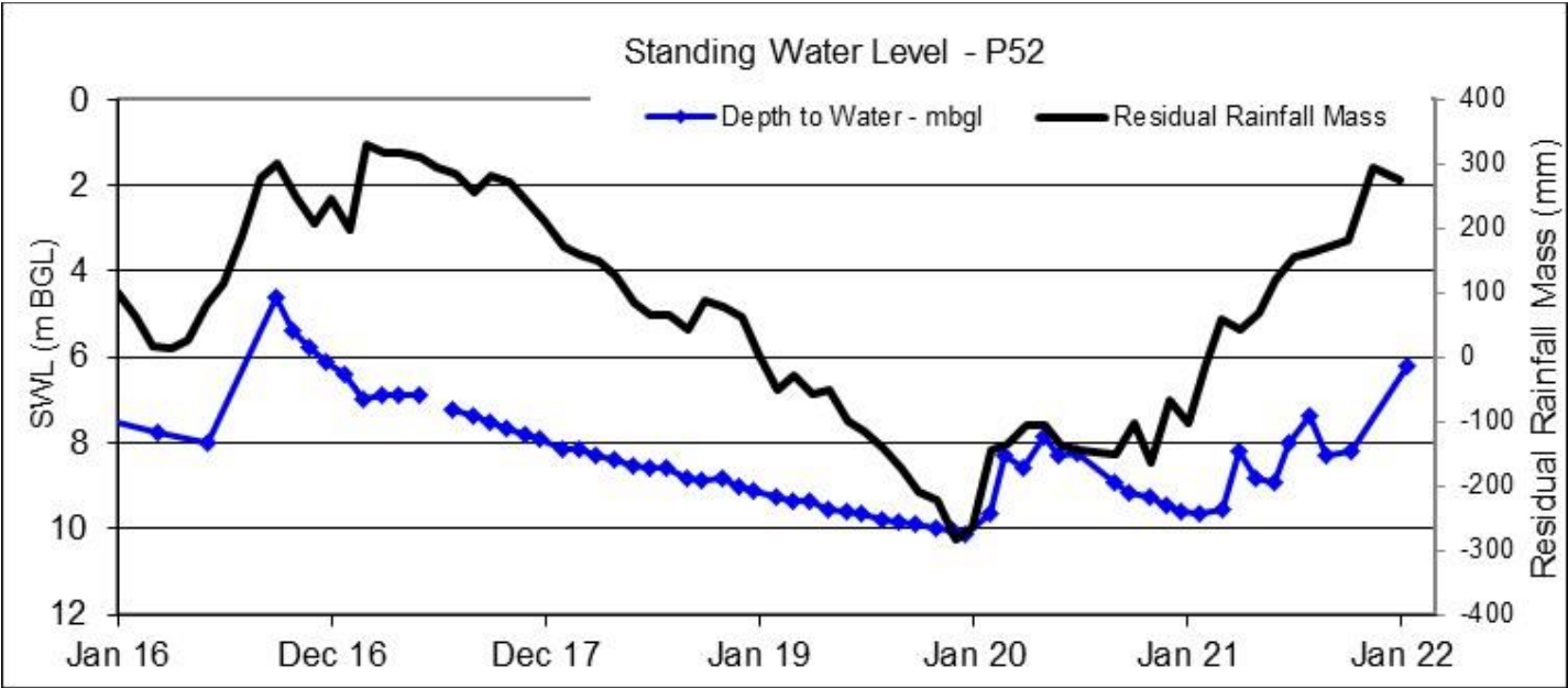
Figure C-33: Hydrograph for P52
