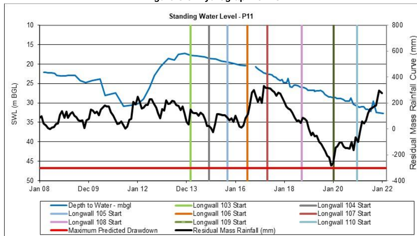
Figure C-7: Hydrograph for P11
