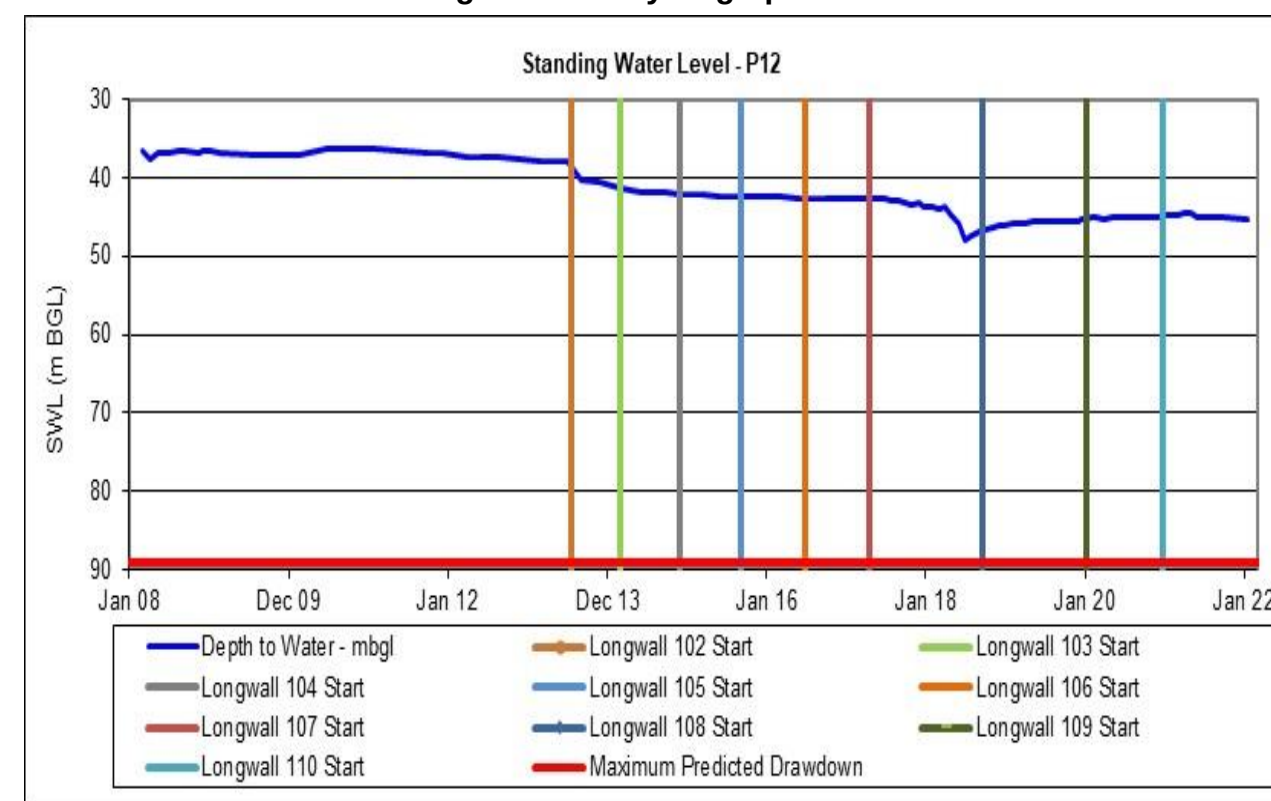
Figure C-16: Hydrograph for P12
