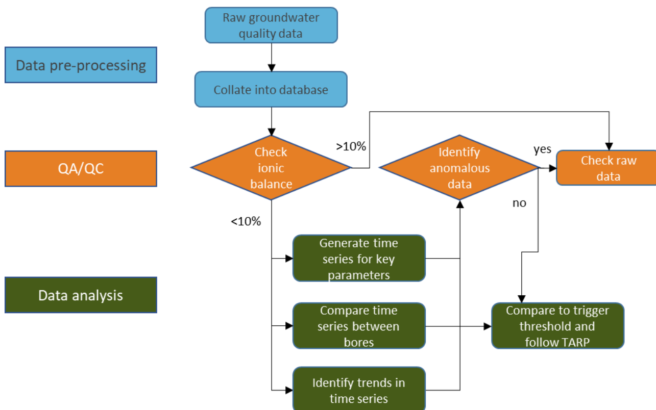
Figure 6-2 Groundwater quality data pre-processing and analysis procedures
