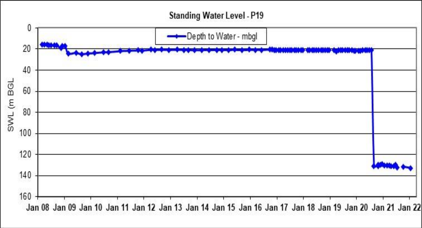
Figure C-18: Hydrograph for P19
