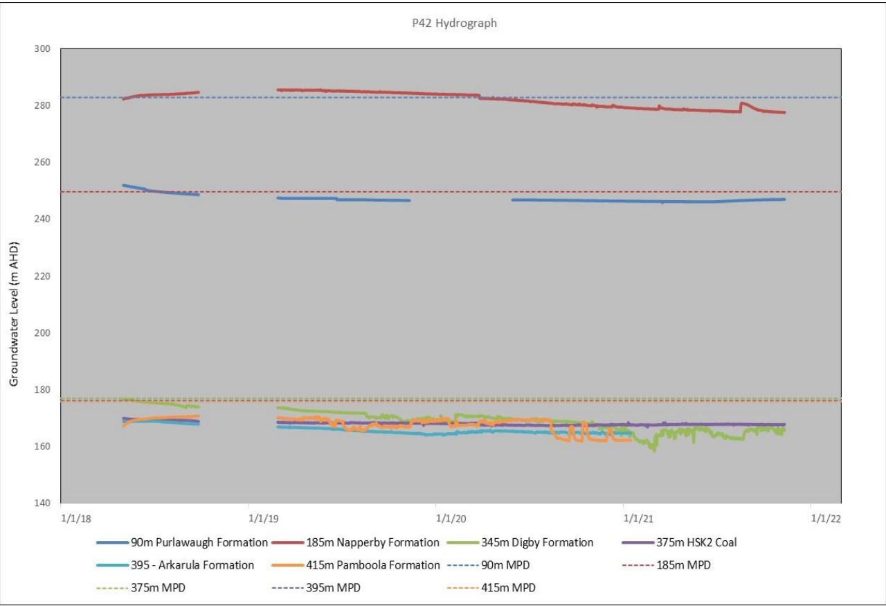
Figure C-20: Hydrograph for P42
