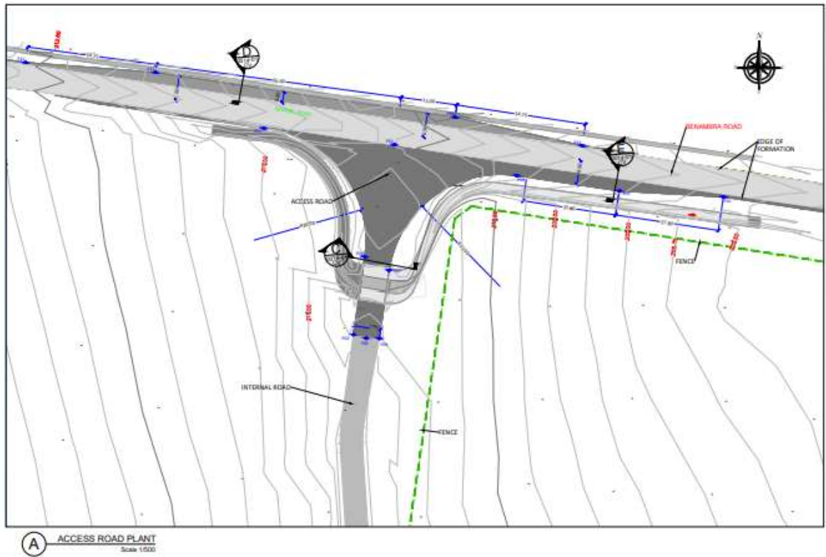
Substation Access off Benambra Rd
