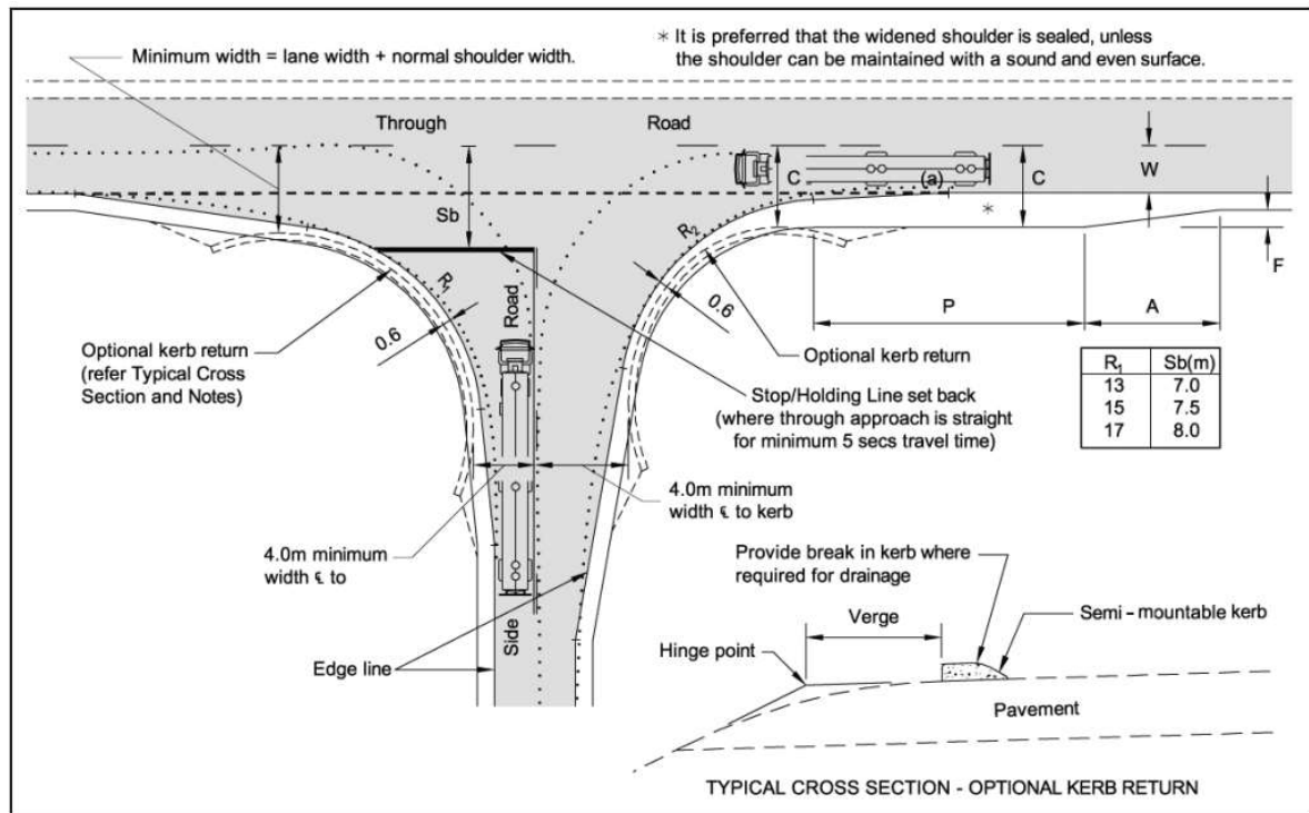
This is a typical Basic LH & RH turn drawing
