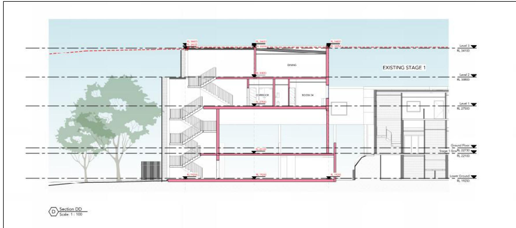
Figure 6 Section D-D (Team 2 Architects 2022)
