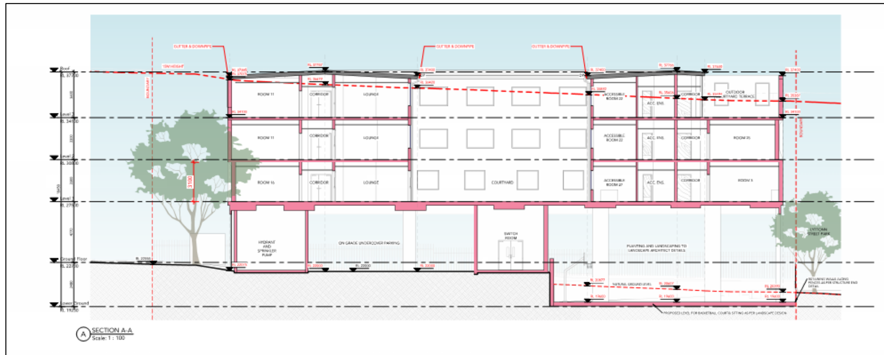
Figure 3 Section A-A (Team 2 Architects 2022)
