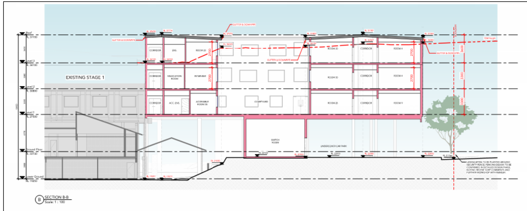
Figure 4 Section B-B (Team 2 Architects 2022)
