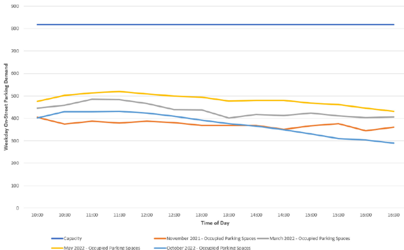
Figure 2: Saturday Surveved on street Parking Demand November 21-October 22
