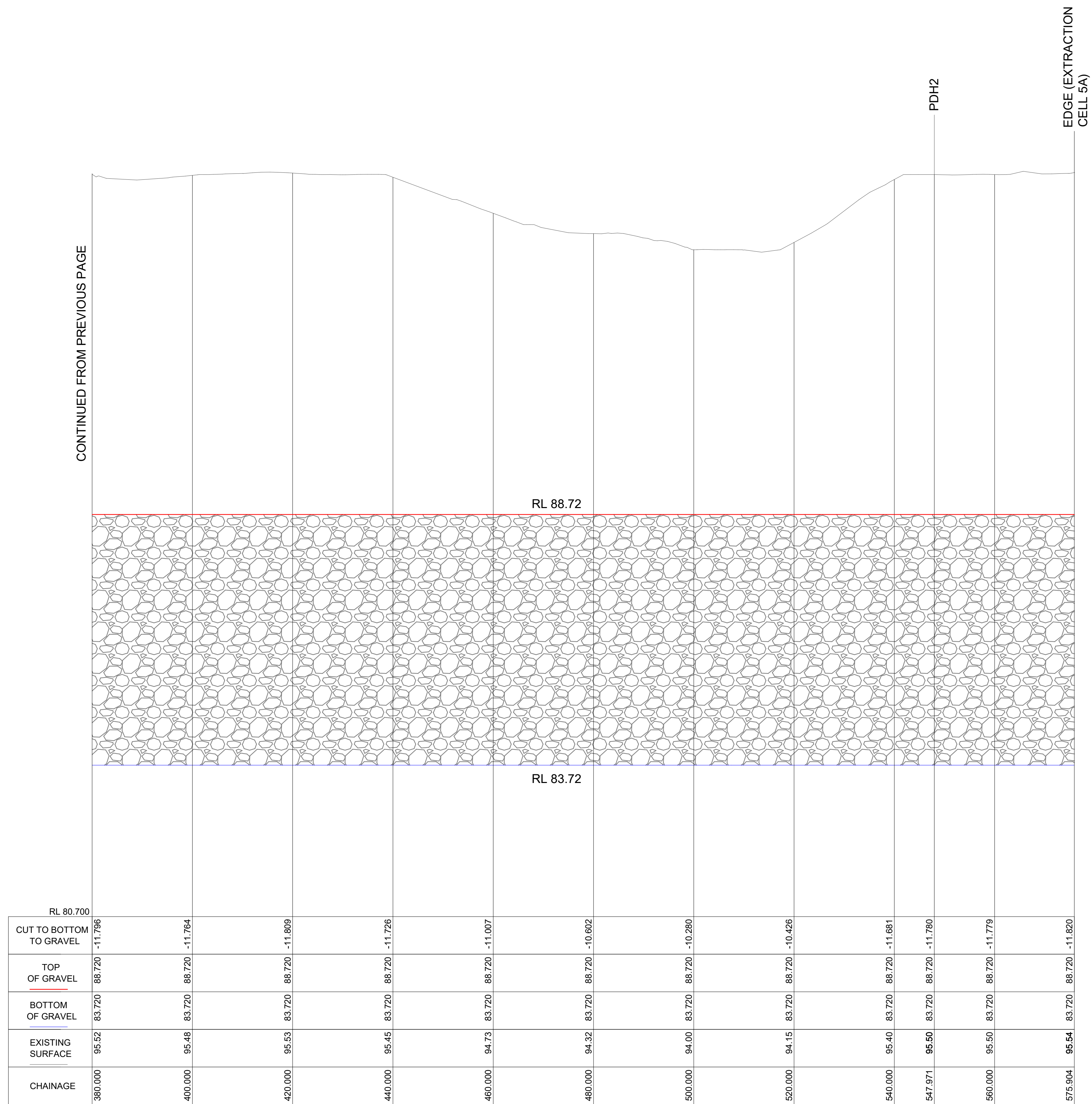
SECTION 02 SCALES: HORIZONTAL 1:500 VERTICAL 1:50
