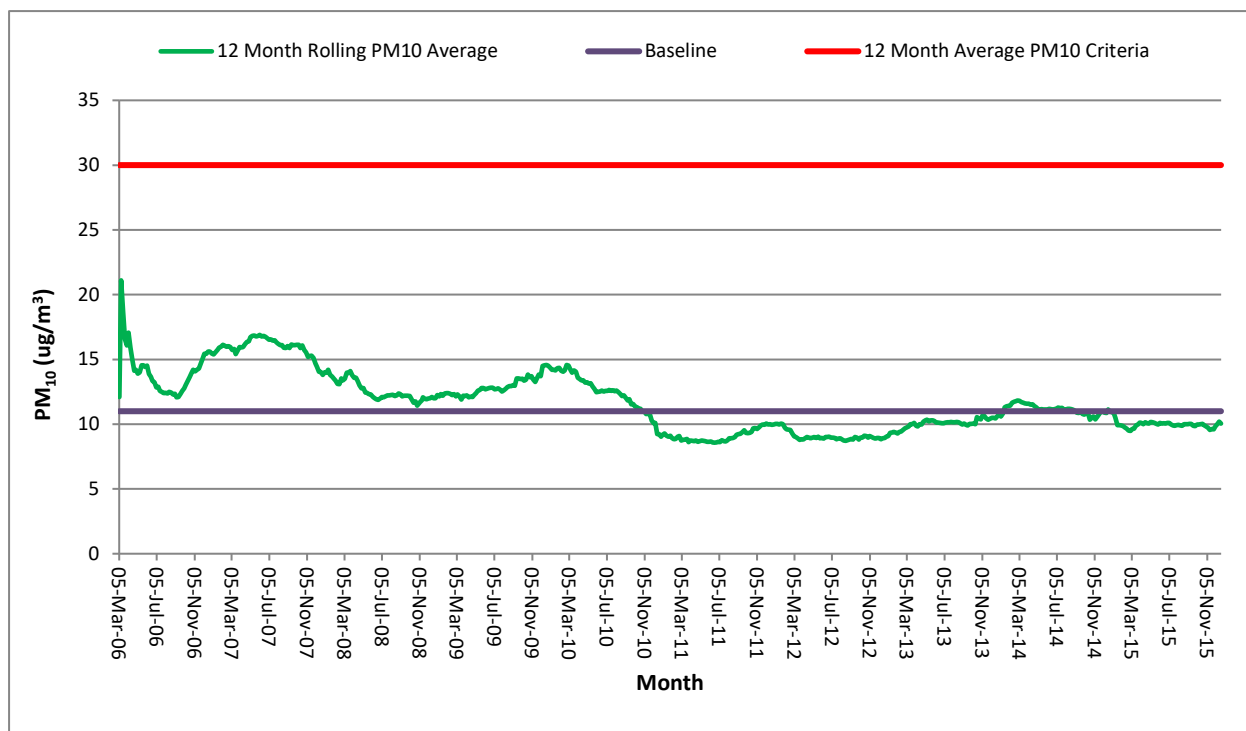
Figure 3: Actual versus Average Baseline PM10 (HV1)
