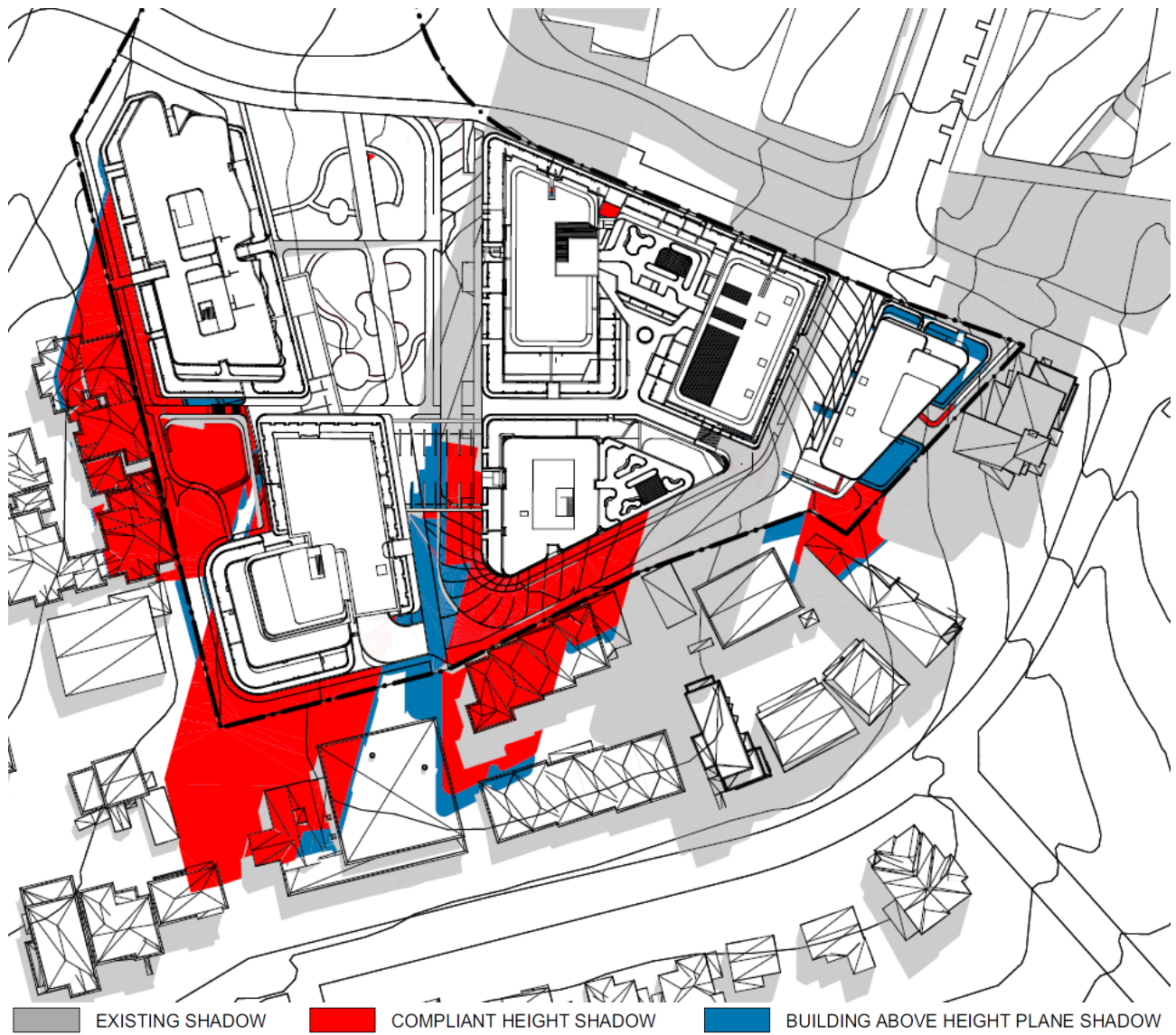
Figure 20 Shadow diagram for Stage 1A on 21 st June at 11am
