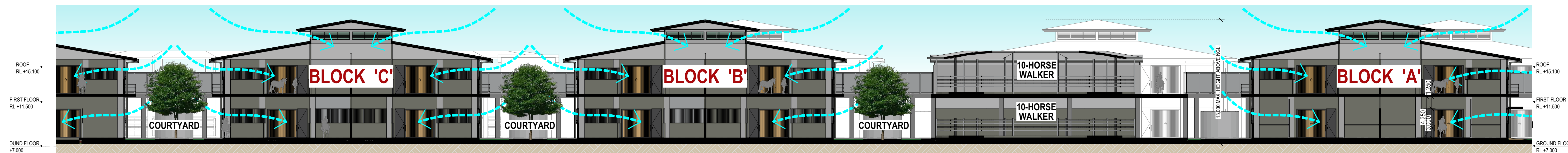
03 1:200 @ A1 TYPICAL STABLES SECTION 03
