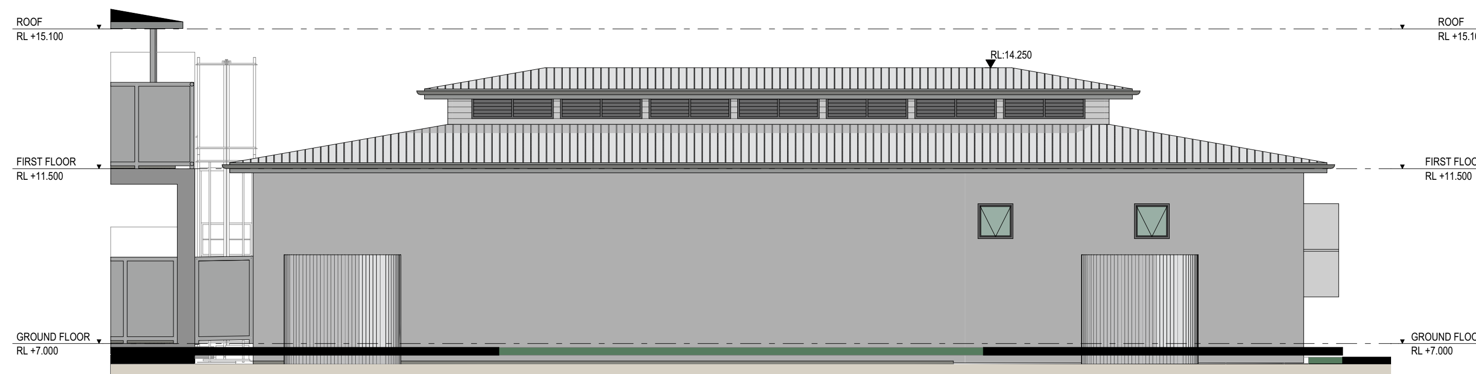
OFFICE NORTH ELEVATION 04 1:100
