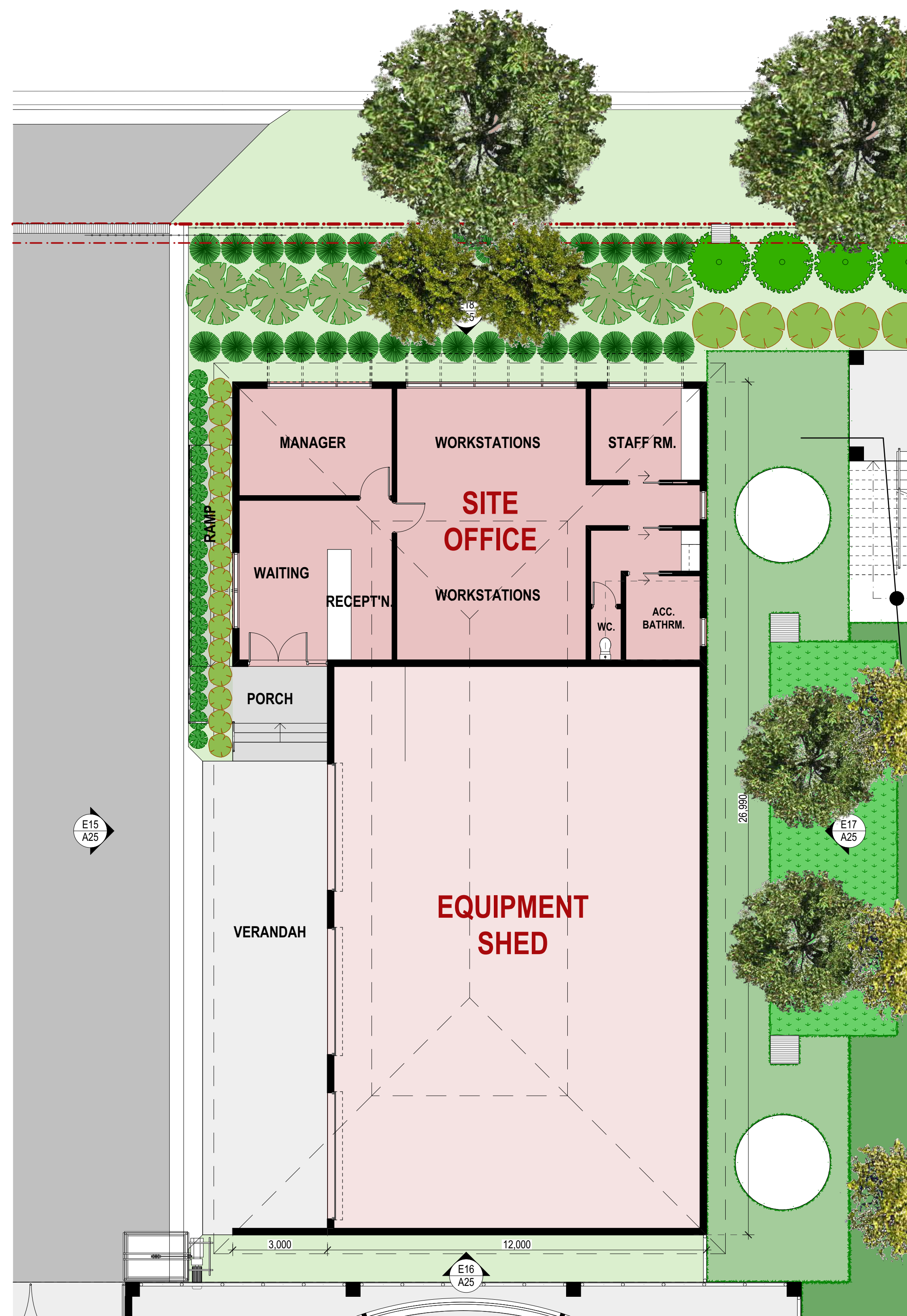
OFFICE & EQUIPMENT SHED PLAN 01 1:100 @ A1
