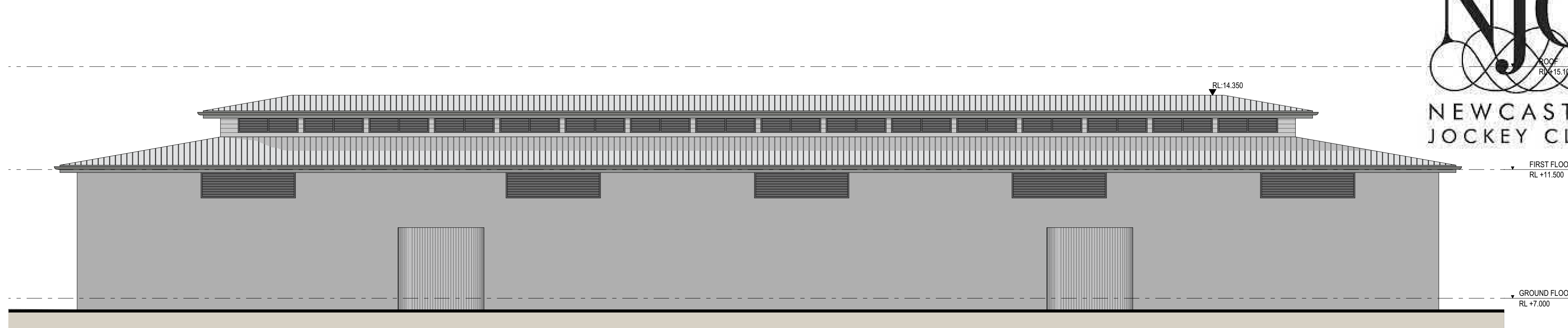
05 GOODS STORAGE SHED WEST ELEVATION 1:100
