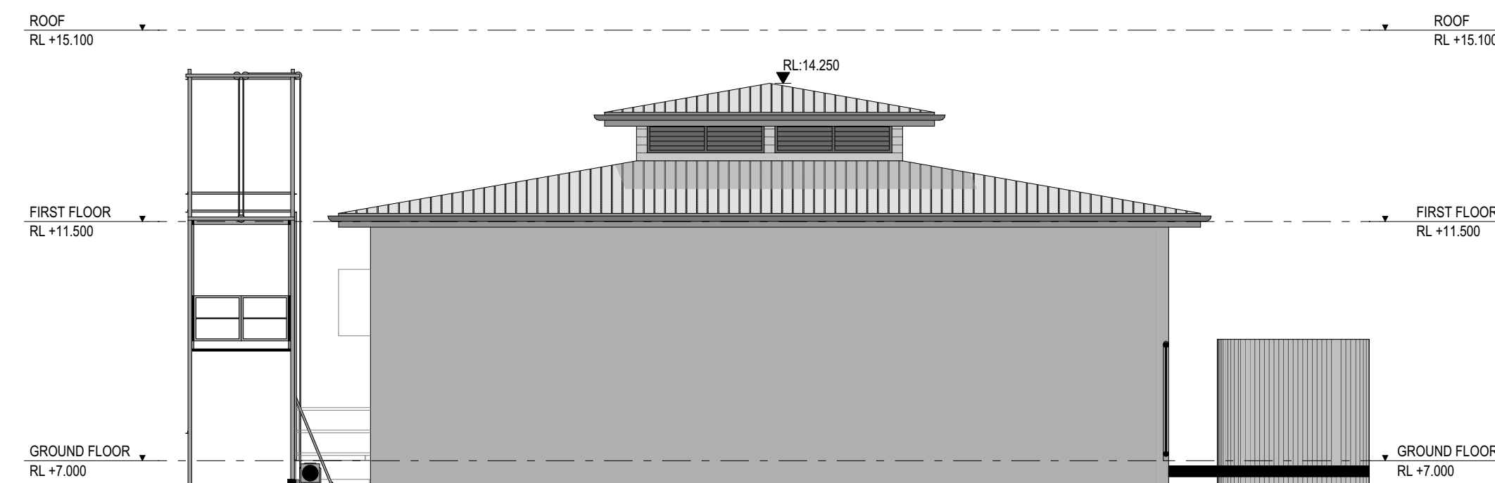
OFFICE EAST ELEVATION 03 1:100
