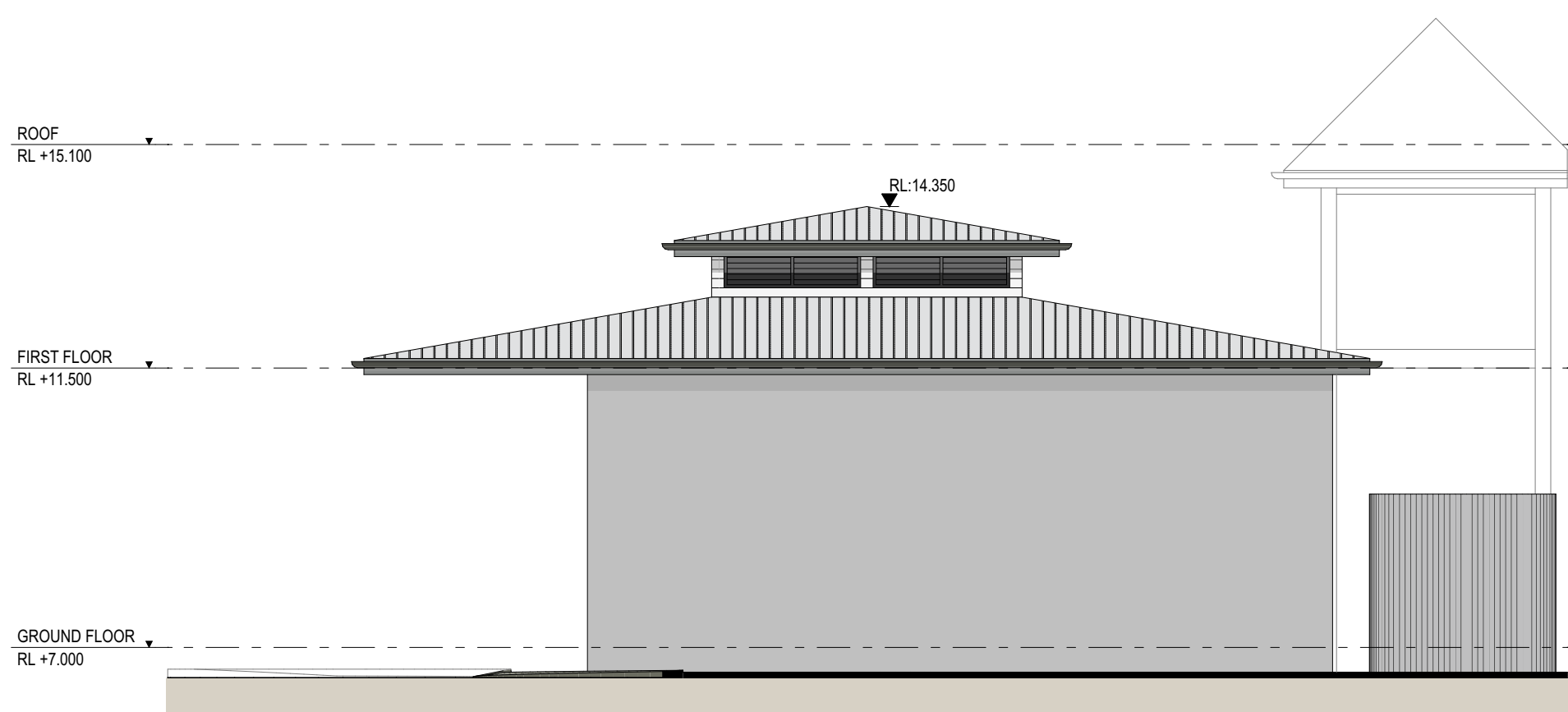
04 GOODS STORAGE SHED NORTH ELEVATION 1:100
