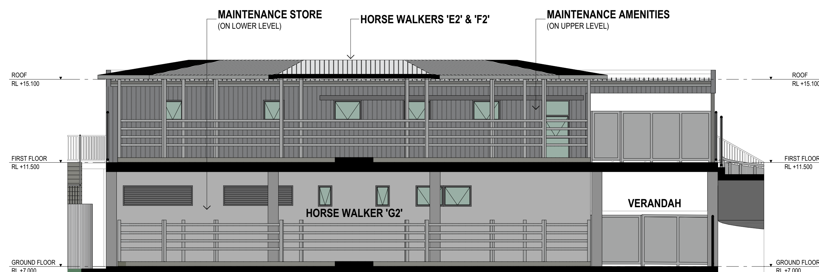
02 1:100 MAINTENANCE FACILITY EAST ELEVATION
