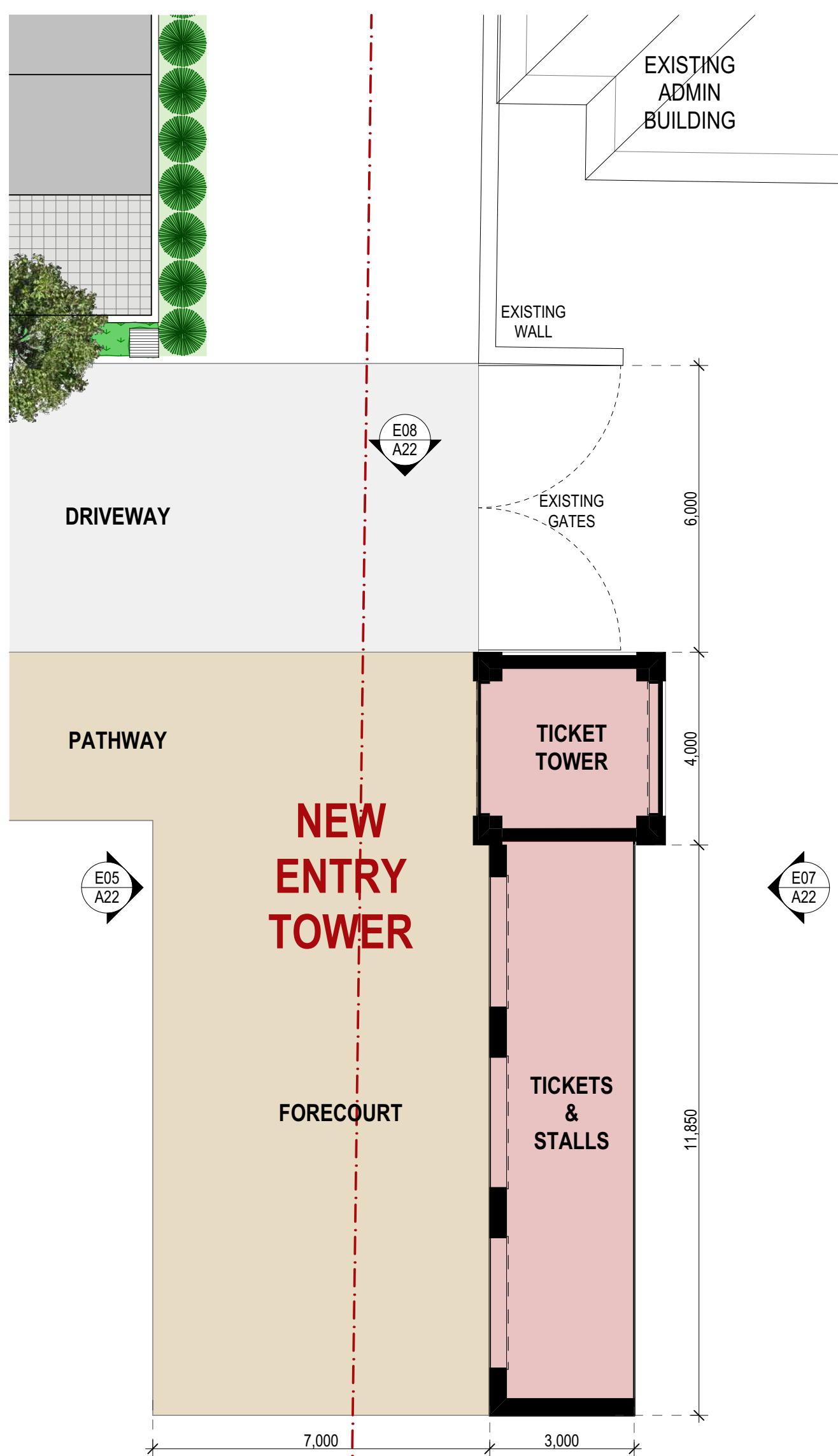
01 1:100 @ A1 NEW ENTRY TOWER PLAN
