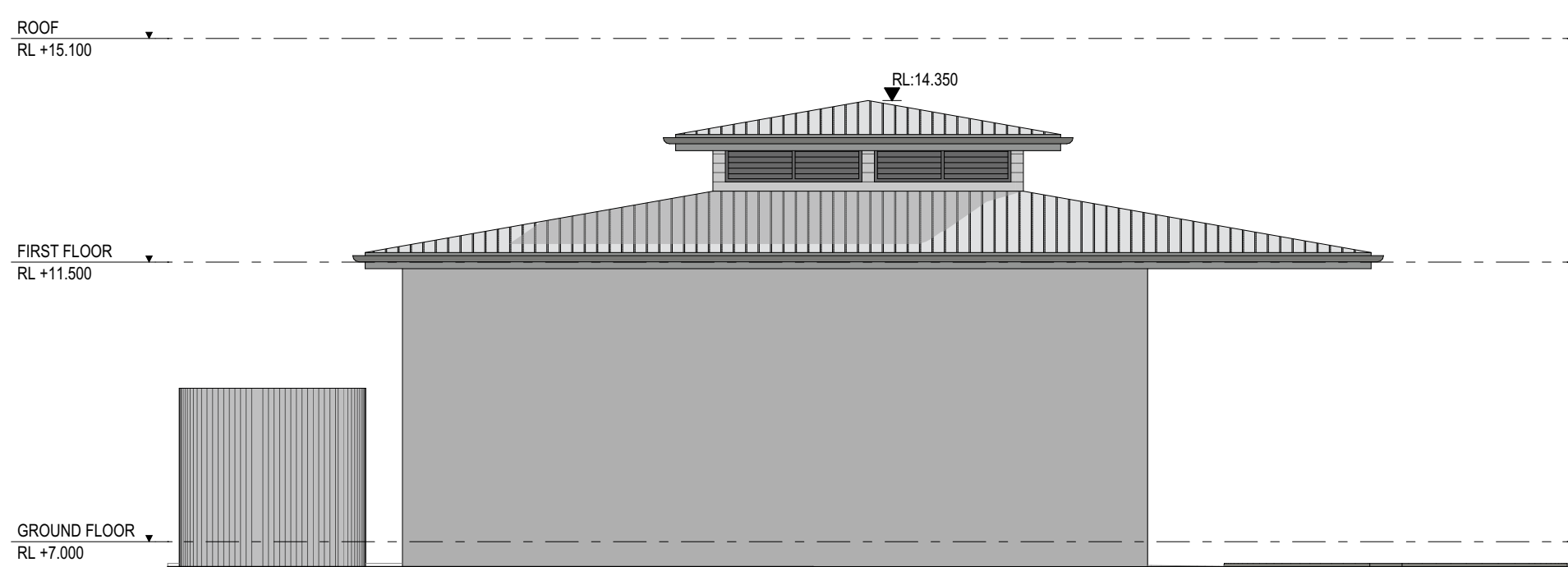
02 GOODS STORAGE SHED SOUTH ELEVATION 1:100 @ A1
