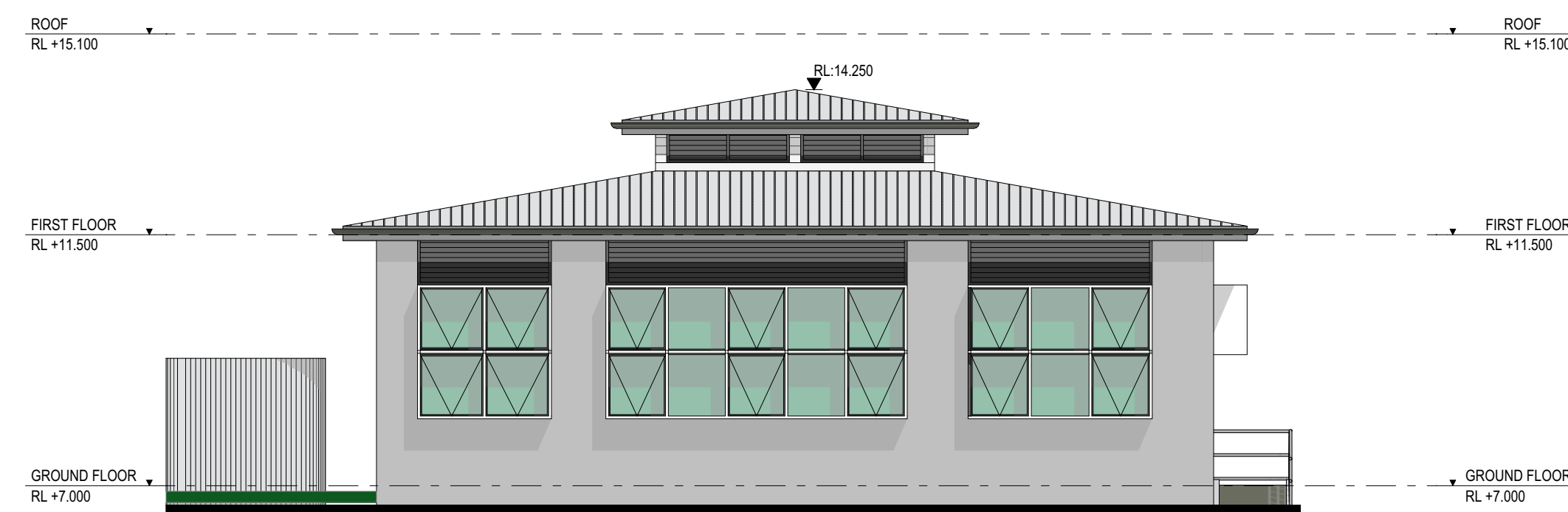
OFFICE WEST ELEVATION 05 1:100
