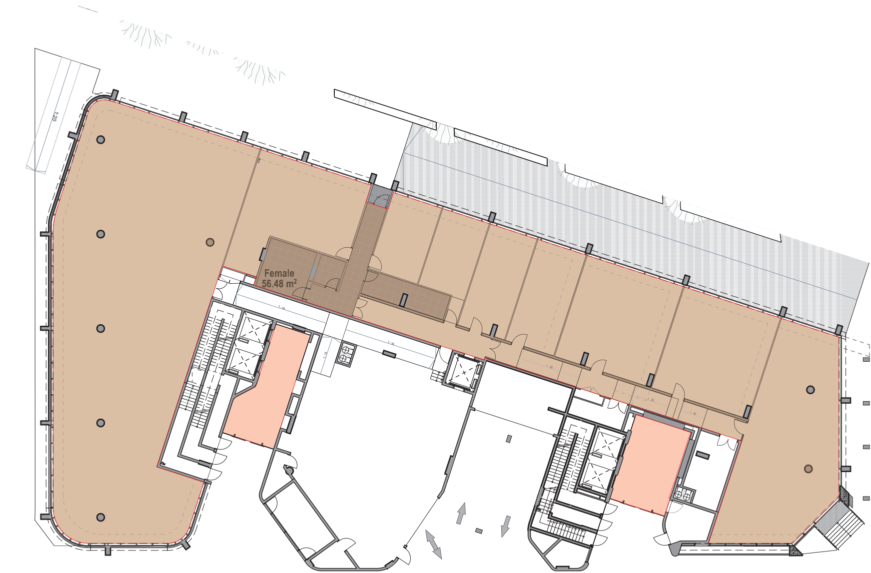
0. Ground Floor 1:300
