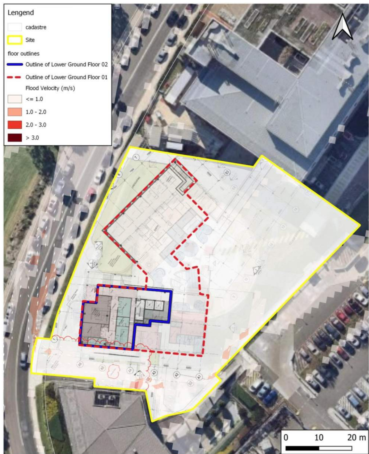
Figure 17 - Flood Velocities (1% AEP) – Proposed Conditions (Ground Floor)
