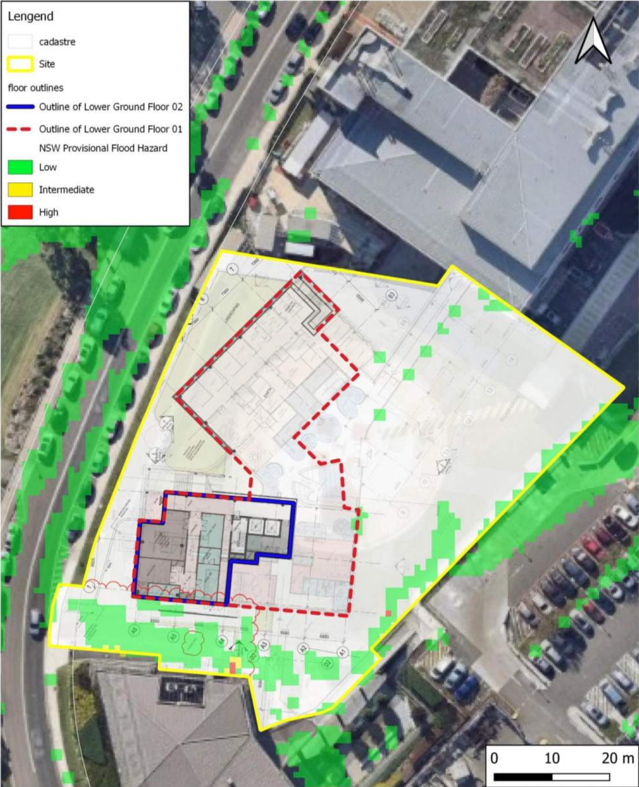
Figure 18 - Provisional Flood Hazards (1% AEP) – Proposed Conditions (Ground Floor)
