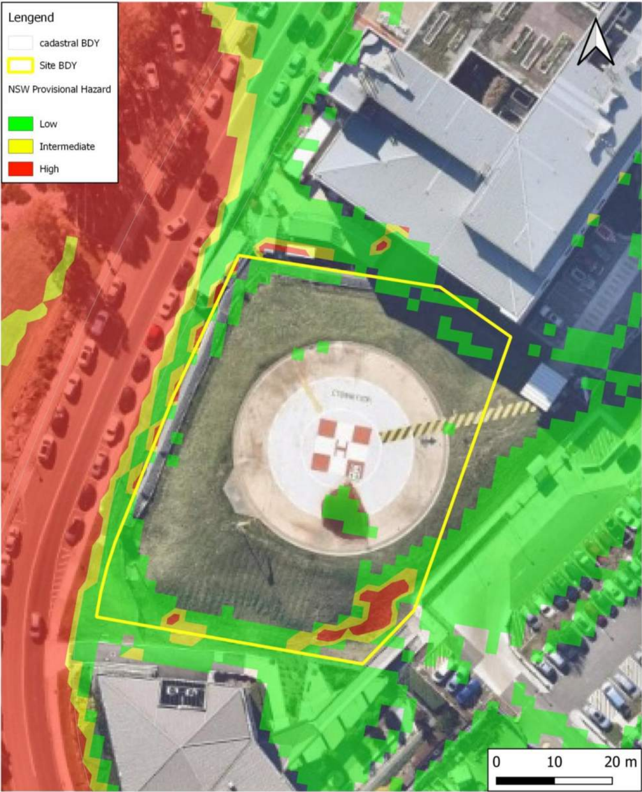
Figure 13 - Provisional Flood Hazards (PMF) – Existing Conditions
