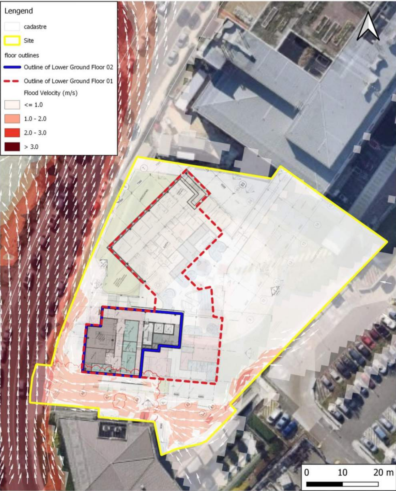
Figure 20 - Flood Velocities (PMF) – Proposed Conditions (Ground Floor)
