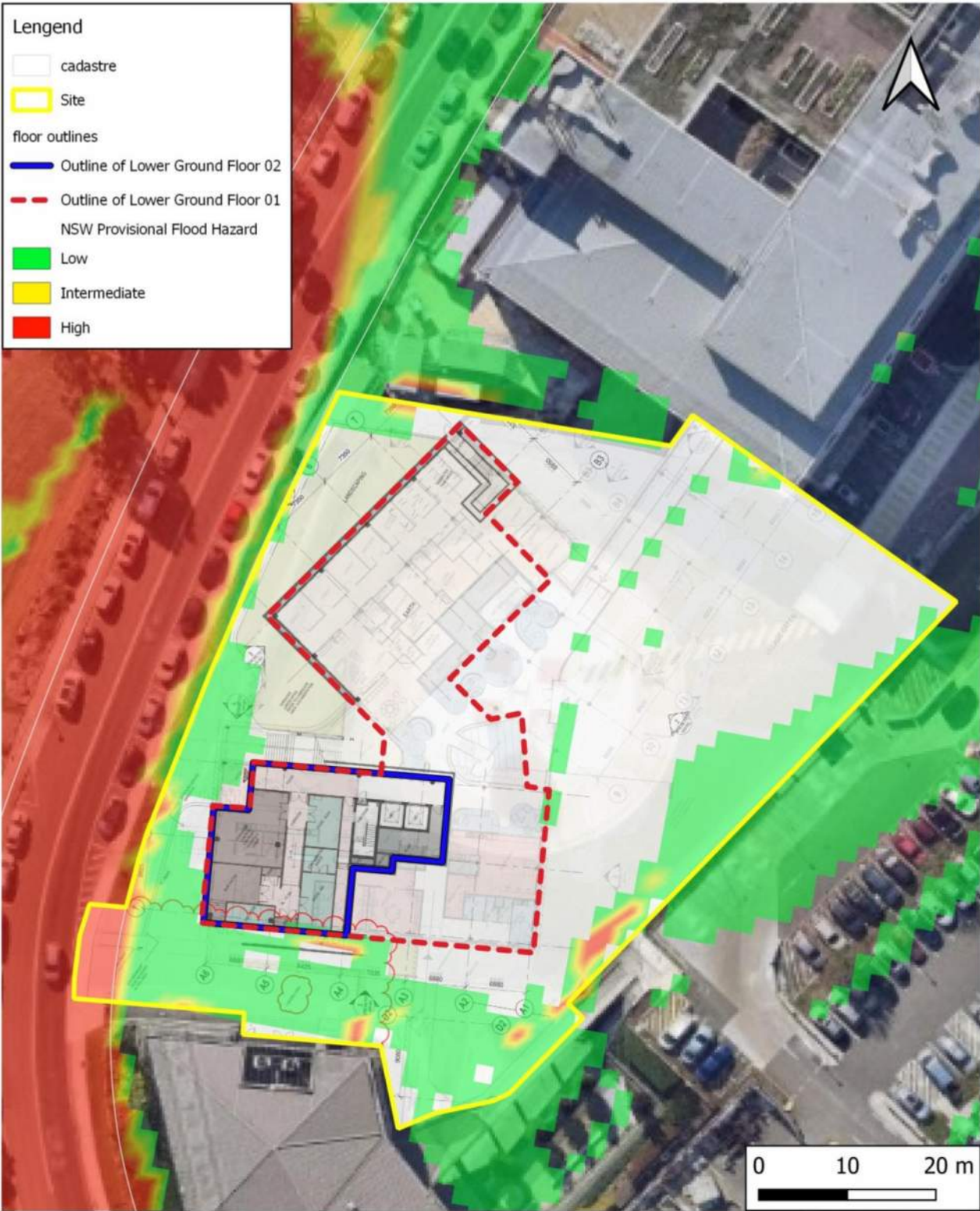
Figure 21 - Provisional Flood Hazards (PMF) – Proposed Conditions (Ground Floor)
