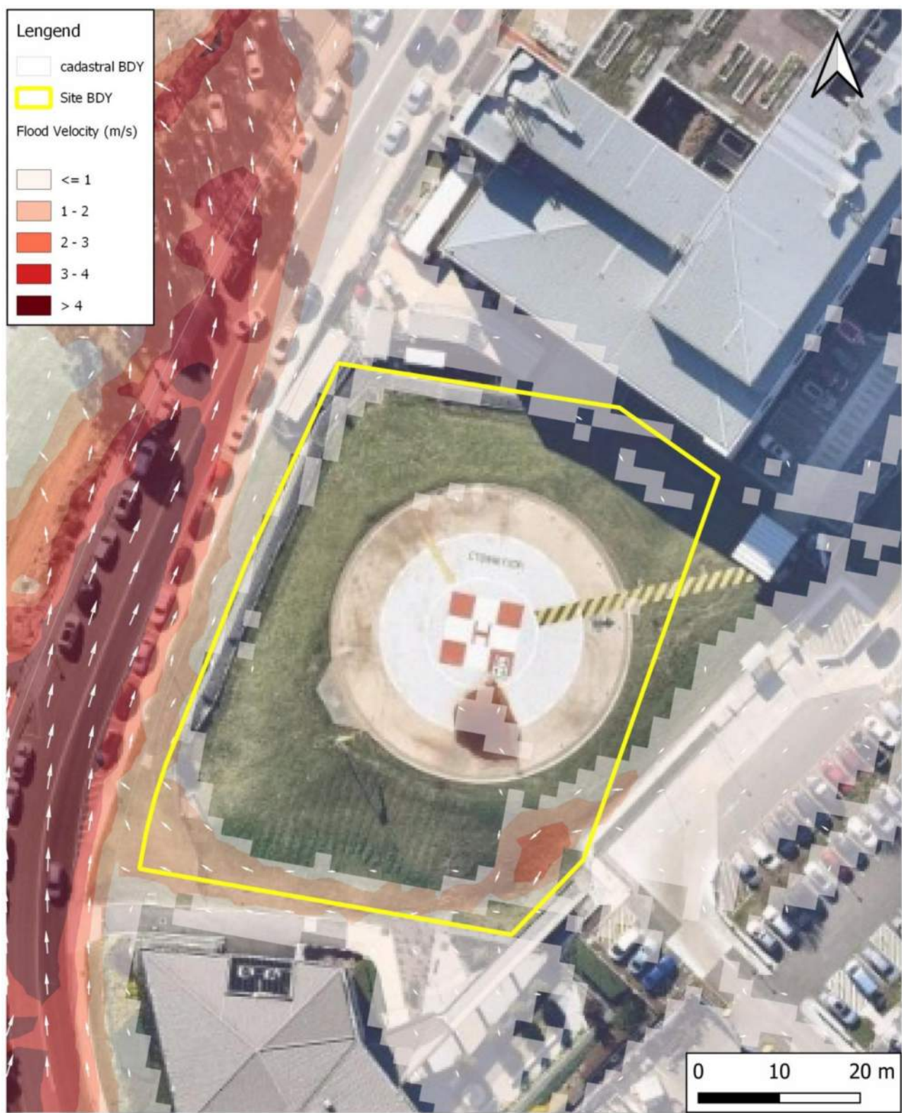
Figure 12 - Flood Velocities (PMF) – Existing Conditions
