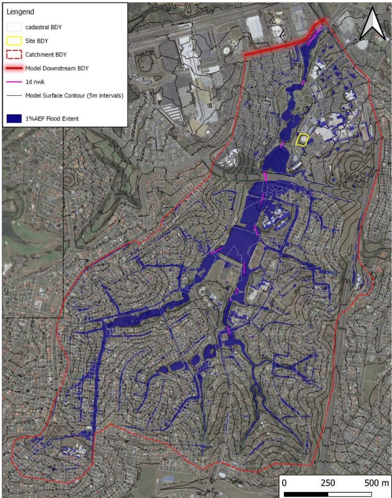
Figure 7 – TUFLOW Model 1D & 2D Domains - 1% AEP Flood Extent
