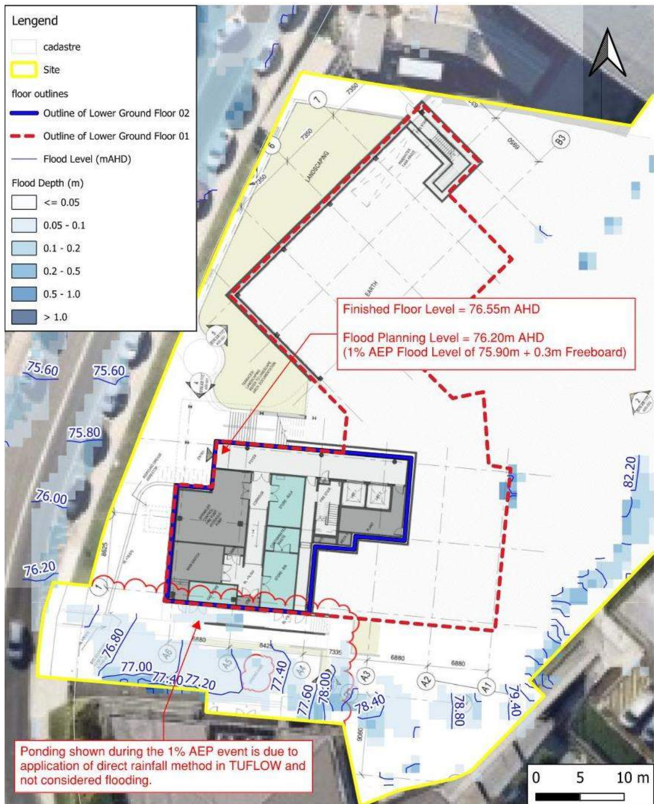
Figure 22 – Flood Panning levels (FPLs) Vs. Proposed Finished Floor Levels (FFLs) – Lower Ground 02
