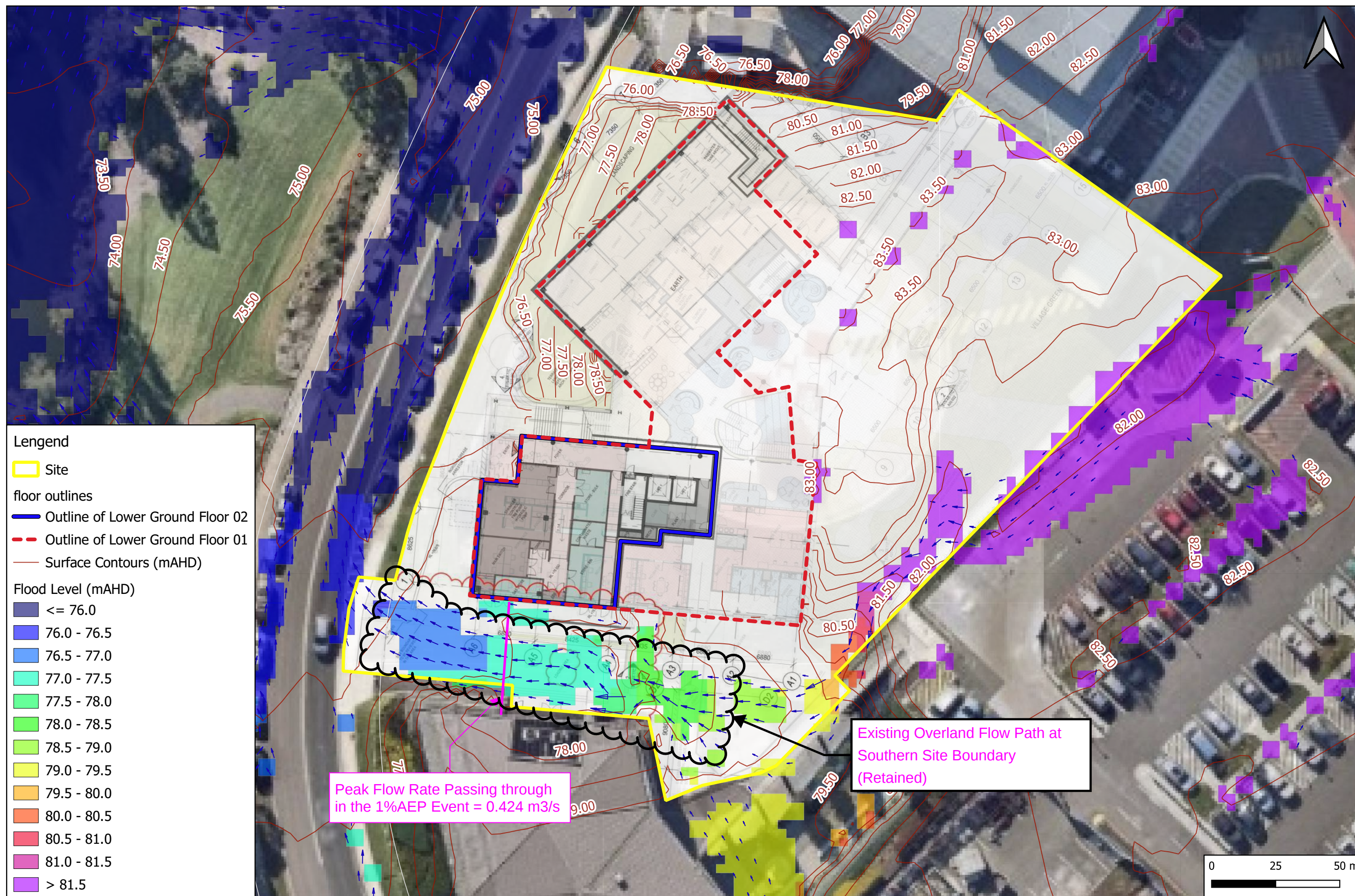
Figure A2 - Existing Overland Flow Path Retained in Post Development Conditions
