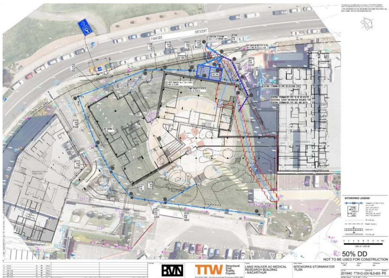
Figure 27 - Proposed Site Stormwater drainage network
