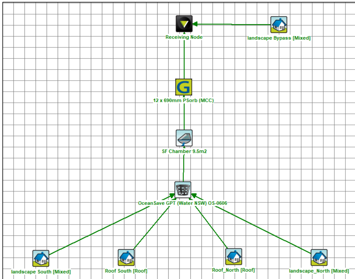
Figure 28 Proposed Treatment Train Layout
