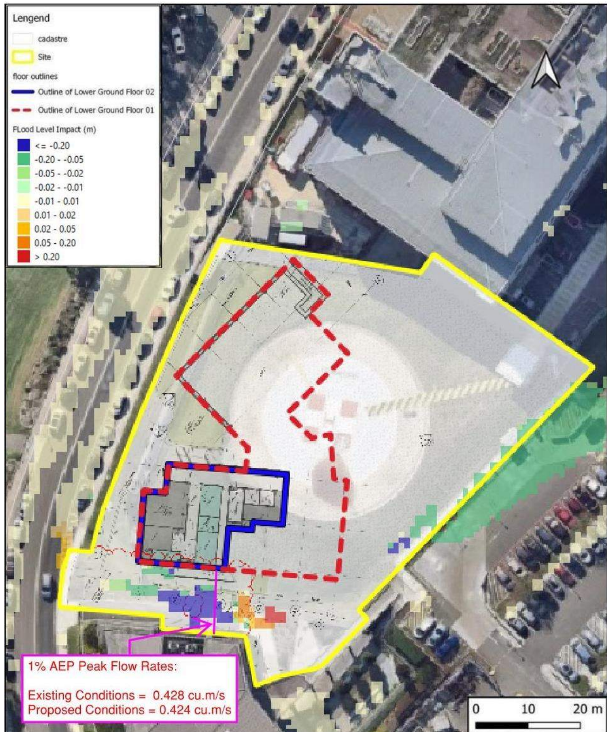
Figure 25 – Flood Impact Assessment Map (1% AEP Flood event)
