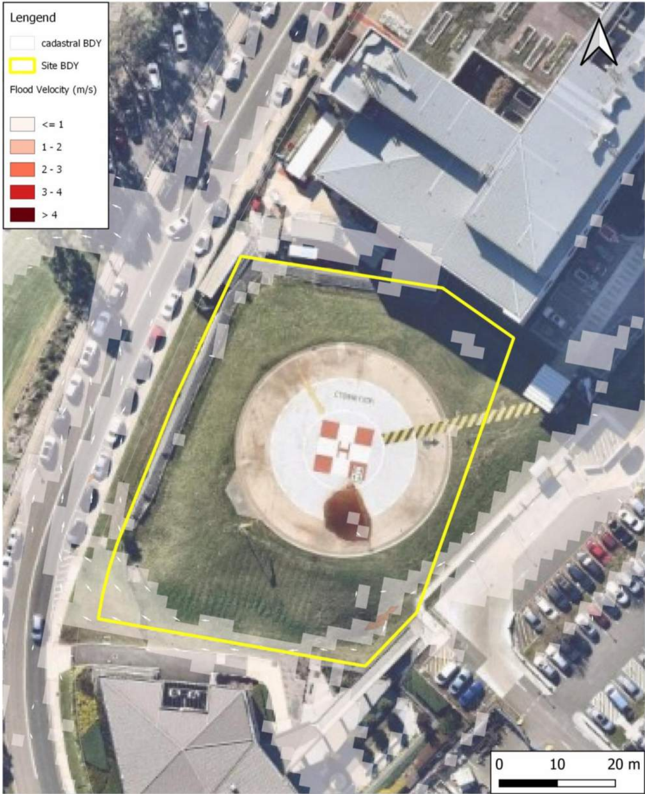
Figure 9 - Flood Velocities (1% AEP) – Existing Conditions
