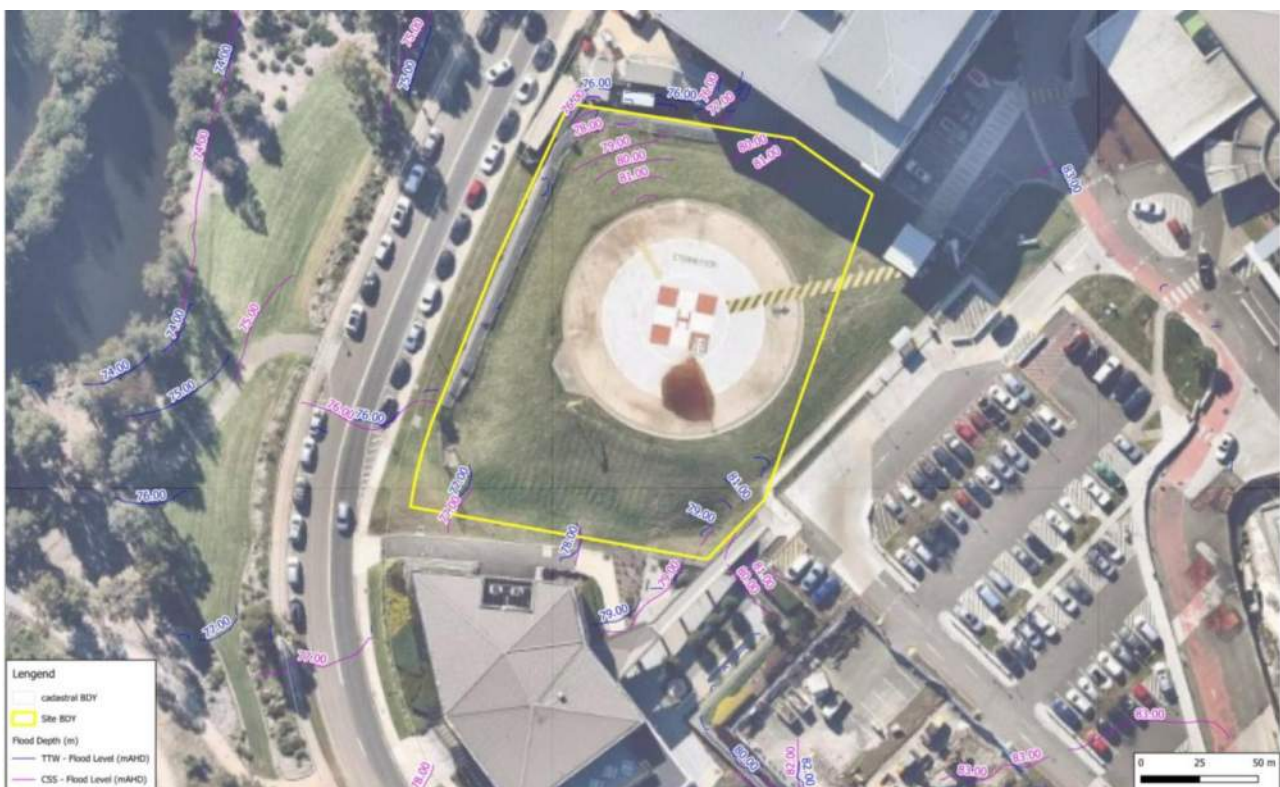
Figure 14 - Flood Level Comparison (CSS vs TTW Model Results) - 1% AEP
