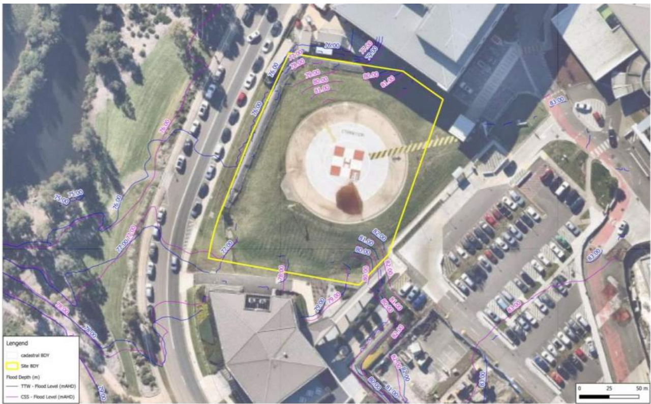
Figure 15 - Flood Level Comparison (CSS vs TTW Model Results) – PMF
