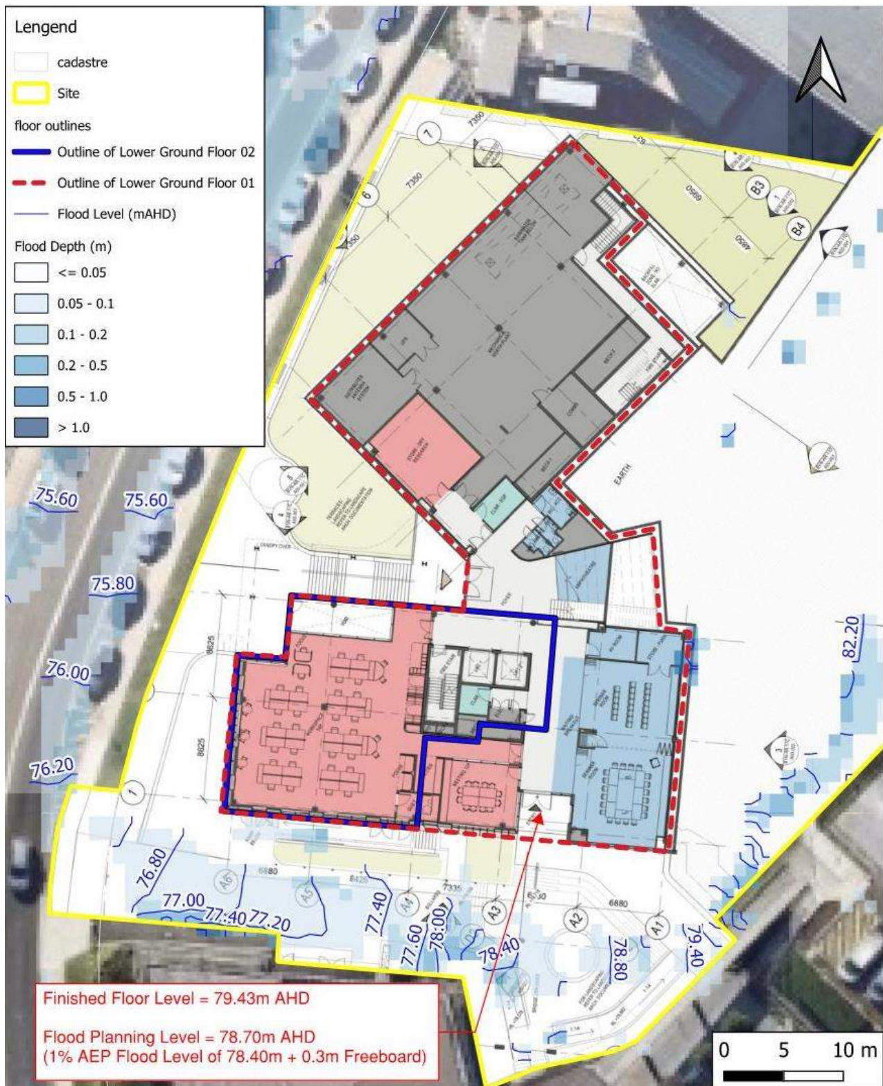
Figure 23 – Flood Panning levels (FPLs) Vs. Proposed Finished Floor Levels (FFLs) – Lower Ground 01
