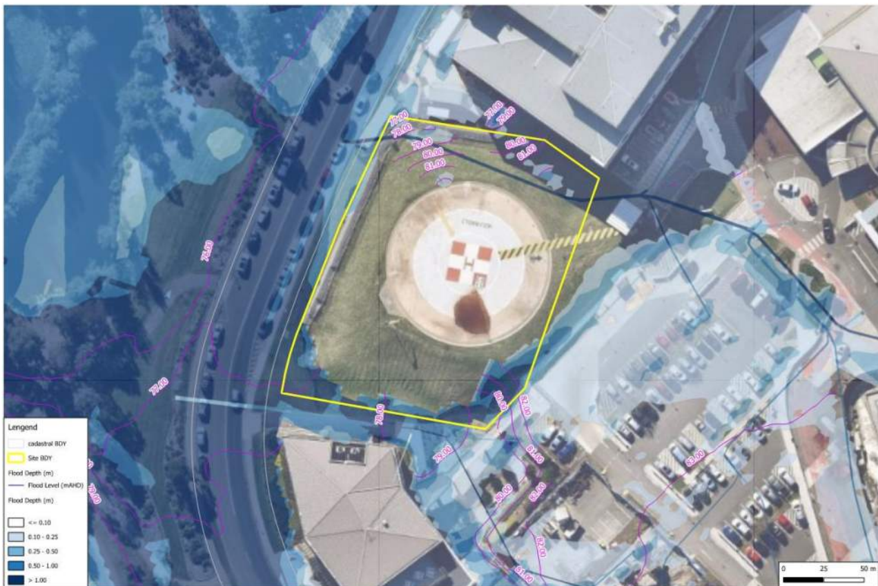
Figure 6 - Received flood Results (CSS) - PMF Flood Event
