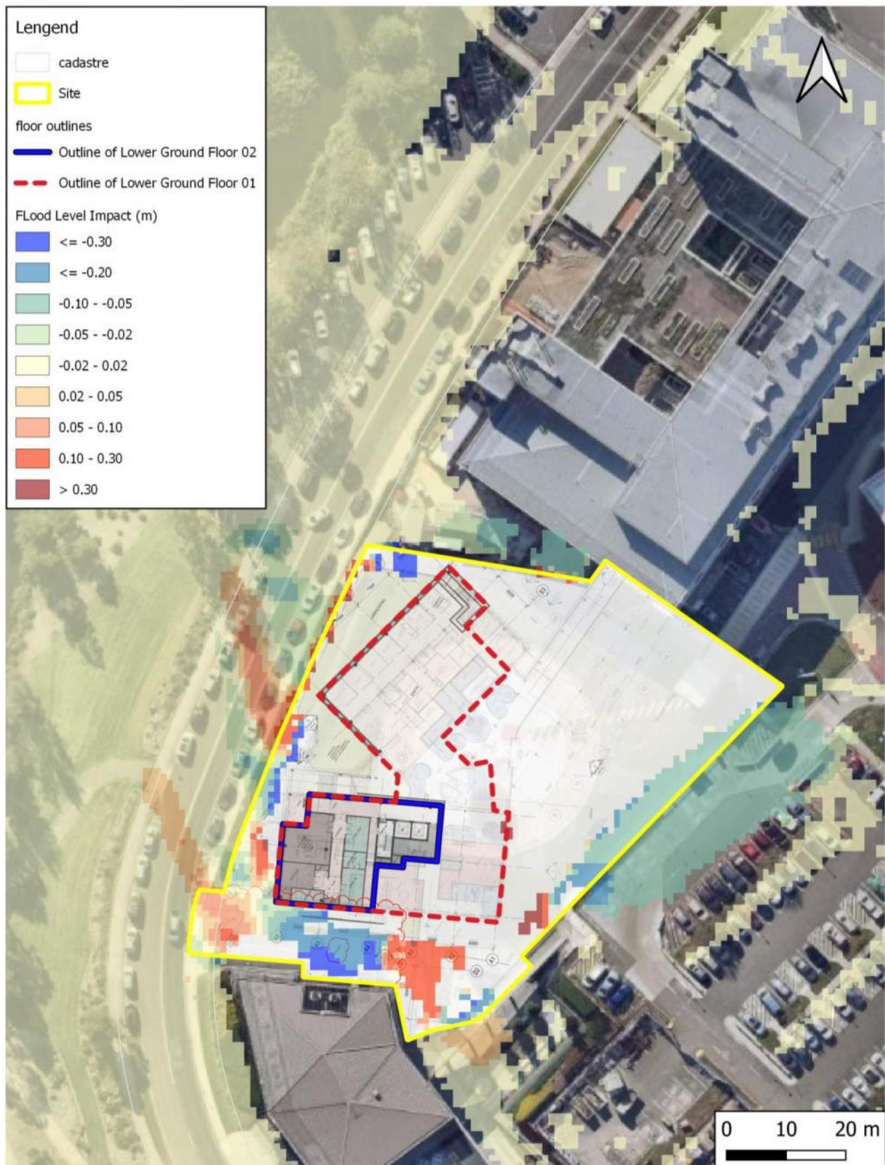
Figure 26 – Flood Impact Assessment Map (PMF event)
