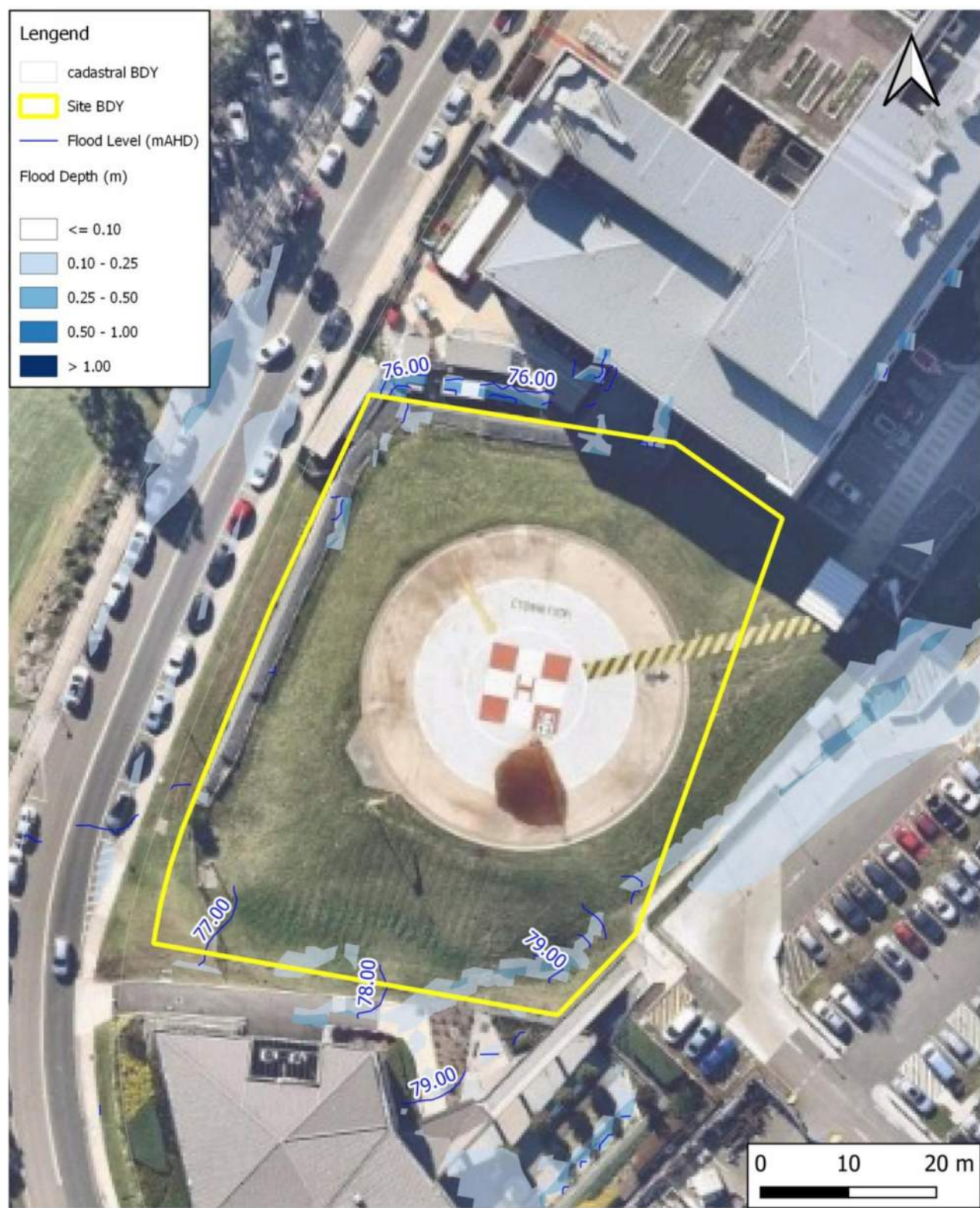
Figure 8 - Flood Levels & Depths (1% AEP) – Existing Conditions
