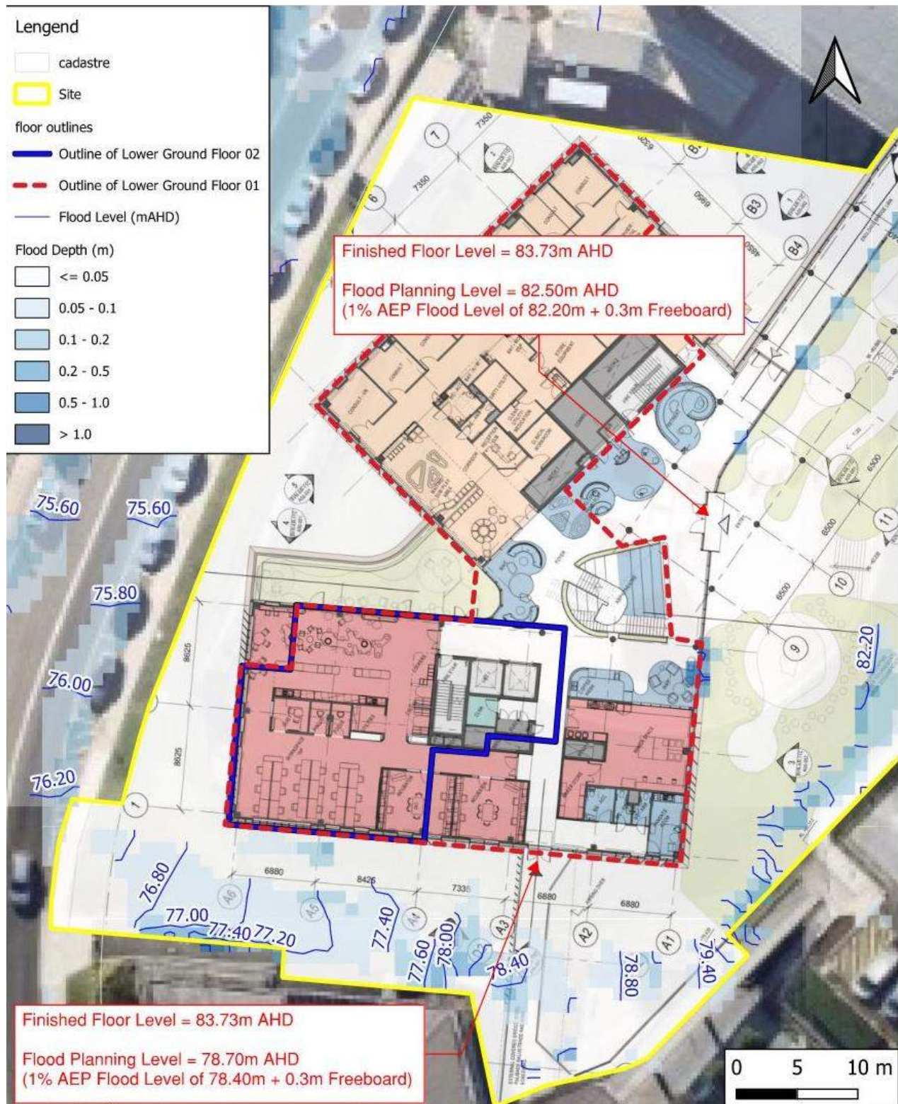
Figure 24 – Flood Panning levels (FPLs) Vs. Proposed Finished Floor Levels (FFLs) – Ground Floor
