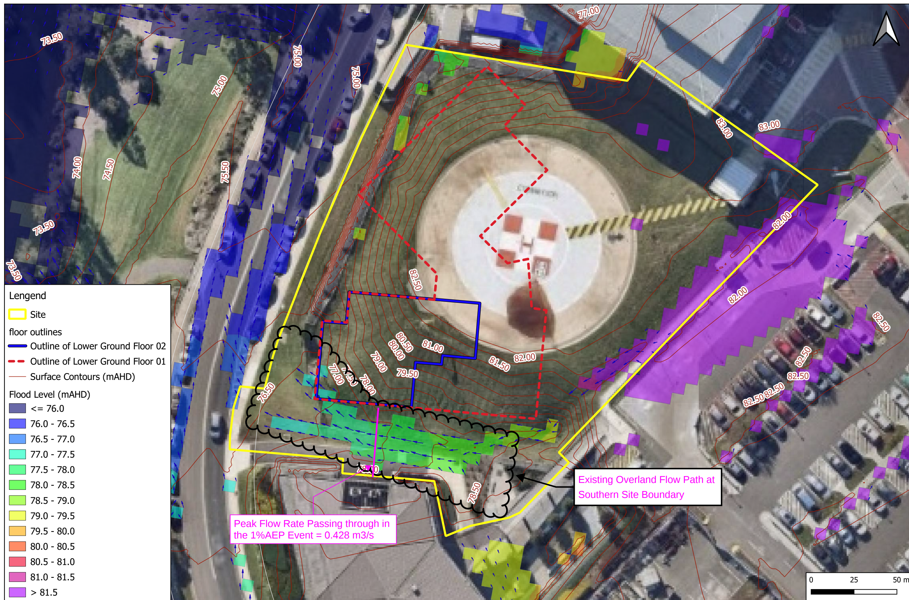
Figure A1 - Existing Overland Flow Path at Southern Site Boundary
