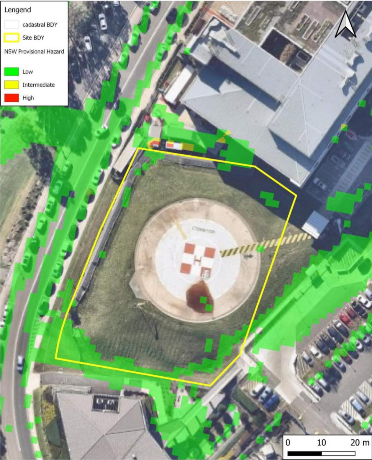
Figure 10 - Provisional Flood Hazards (1% AEP) – Existing Conditions
