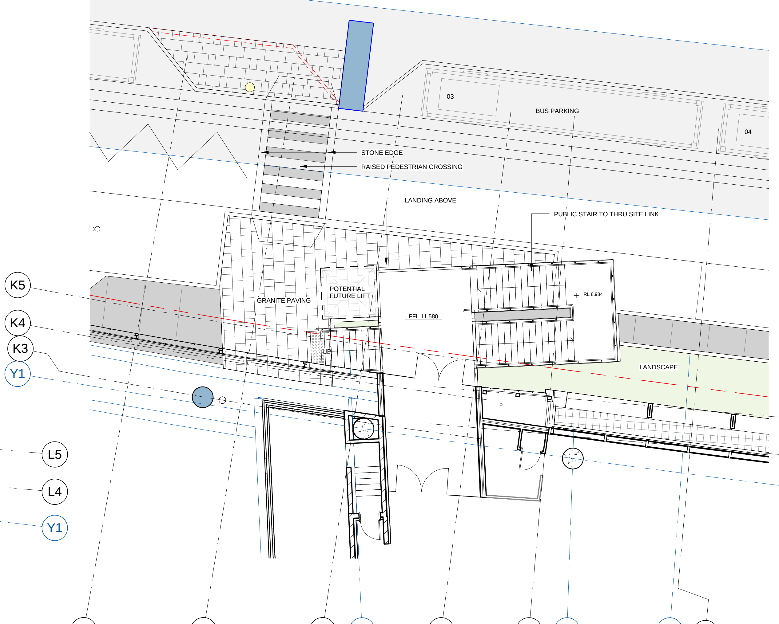
3 PUBLIC DOMAIN - GROUND (Wheat Road) SCALE 1: 100
