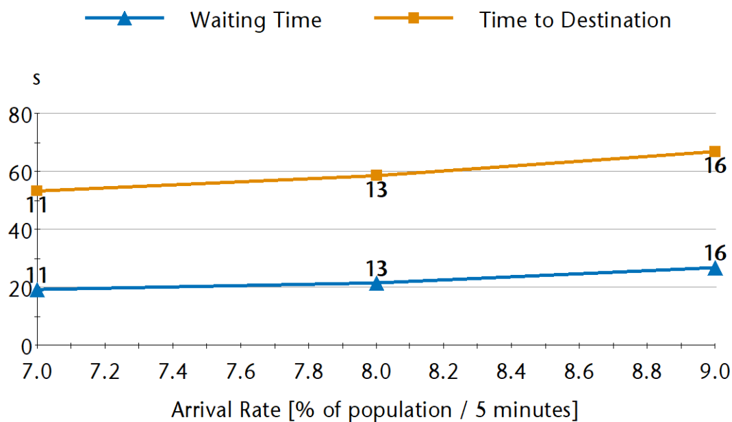
Figure 3. Two way (50%, 50%, 0%) Results for 1600kg @ 2.0mps (3 Lifts).
