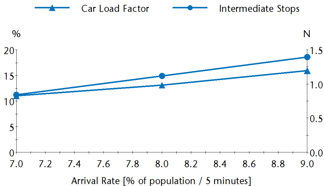
Figure 4. Two way (50%, 50%, 0%) Results for 1600kg @ 2.0mps (3 Lifts).
