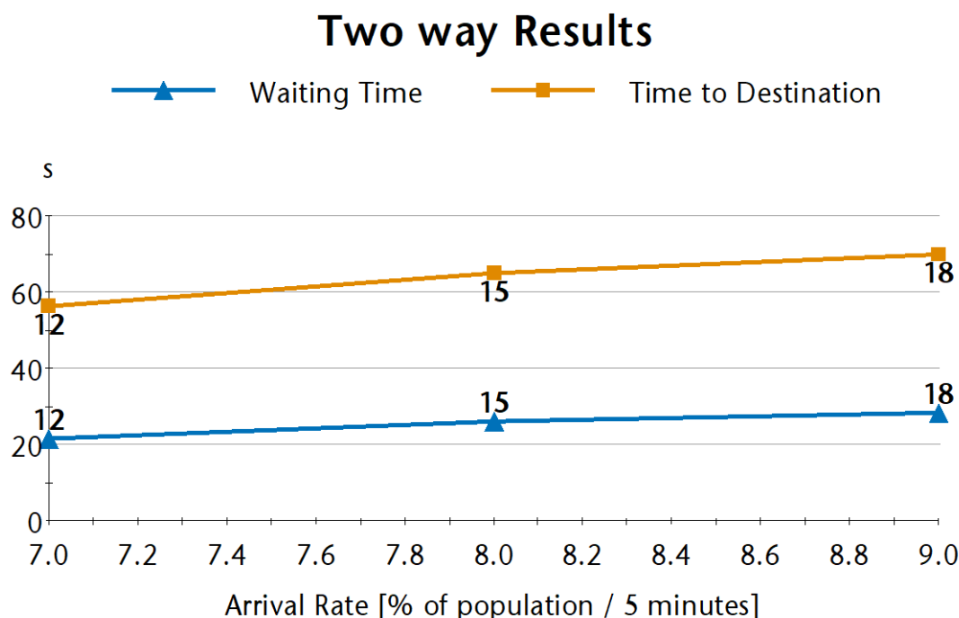
Figure 1. Two way (15%, 85%, 0%) Results for 1600kg @ 2.0mps (3 Lifts).
