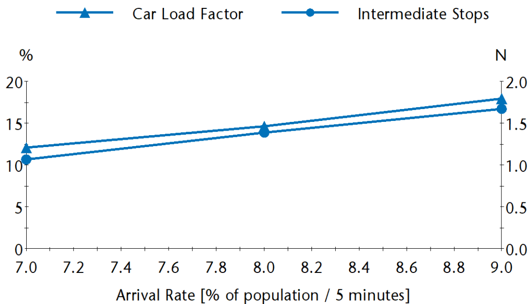
Figure 2. Two way (15%, 85%, 0%) Results for 1600kg @ 2.0mps (3 Lifts).
