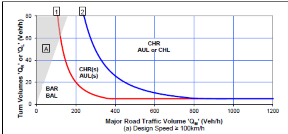
Figure 4.2: Austroads Warrants for Turn Treatments
