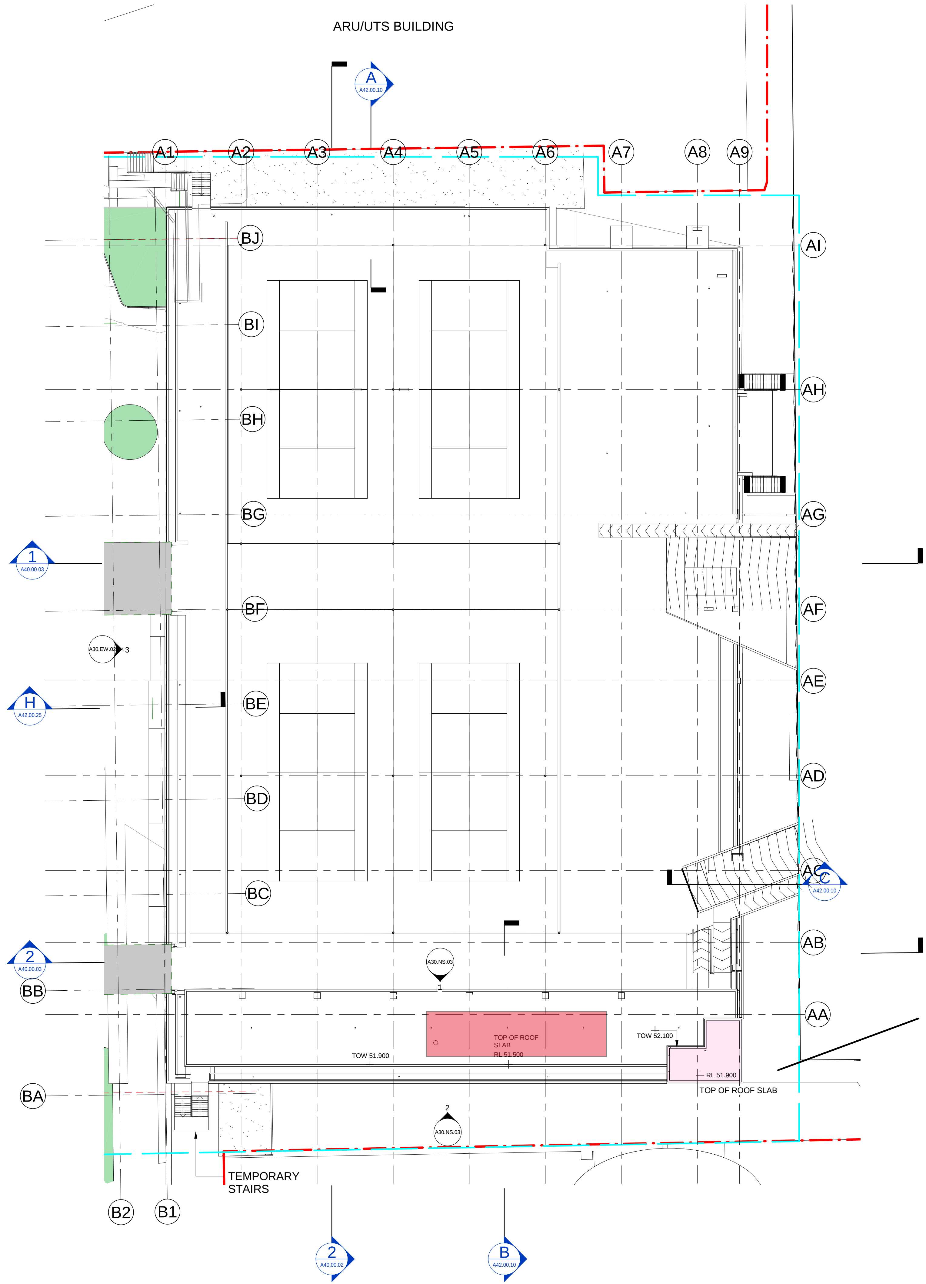
1 SSDA ROOF LEVEL EAST SCALE 1 : 250
