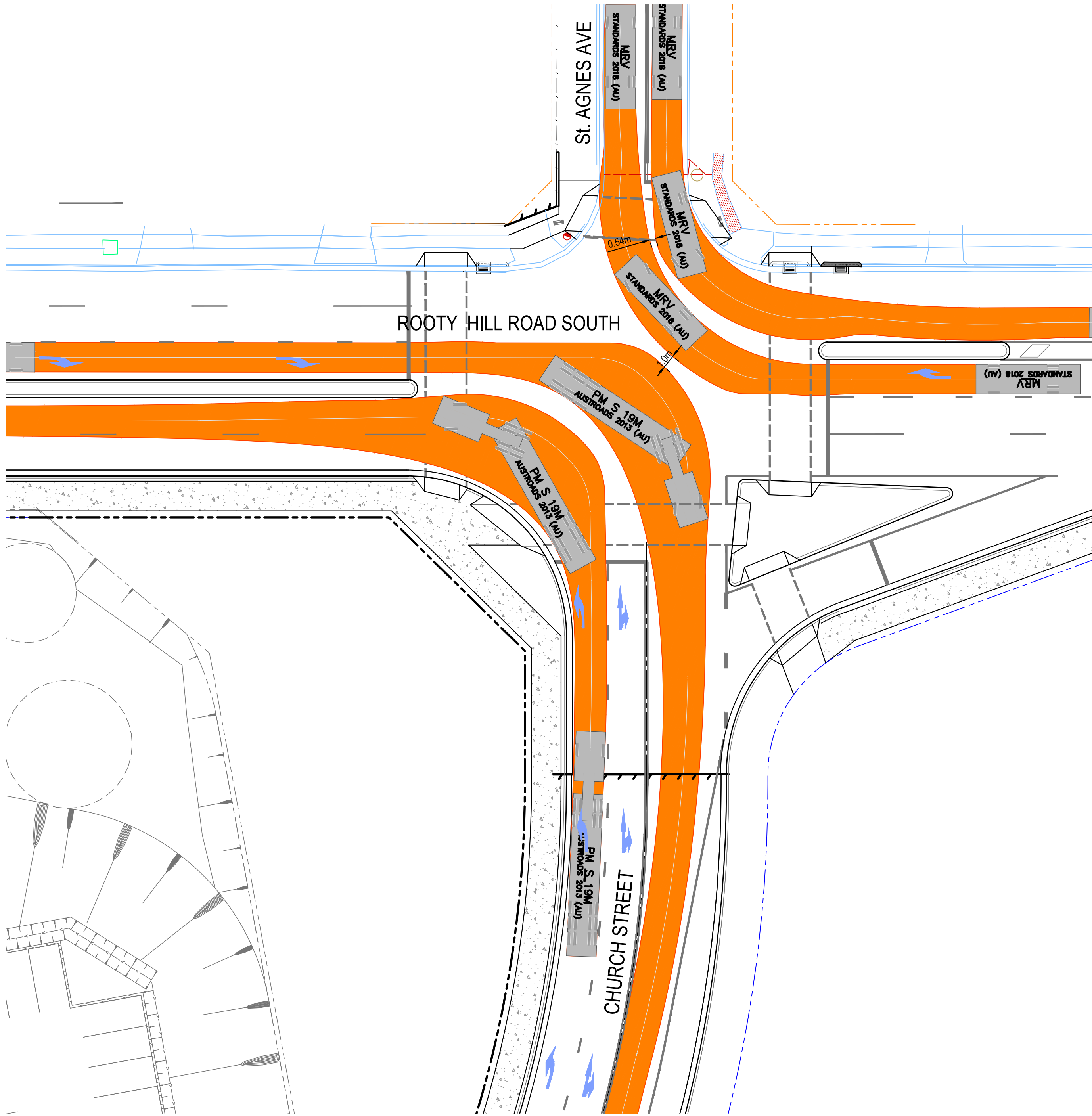
INTERSECTION LAYOUT - TURNING PATHS
