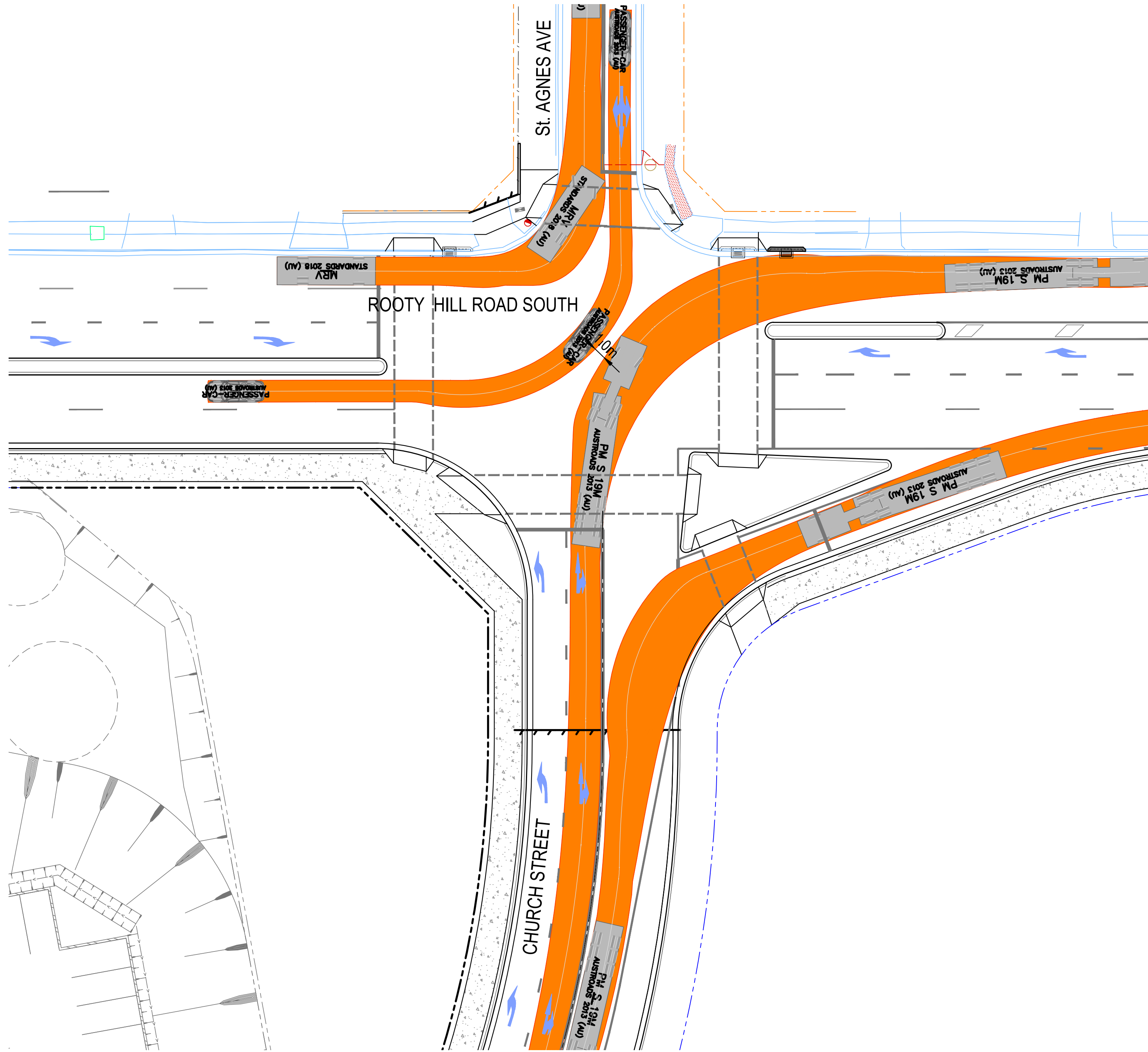
INTERSECTION LAYOUT - TURNING PATHS
