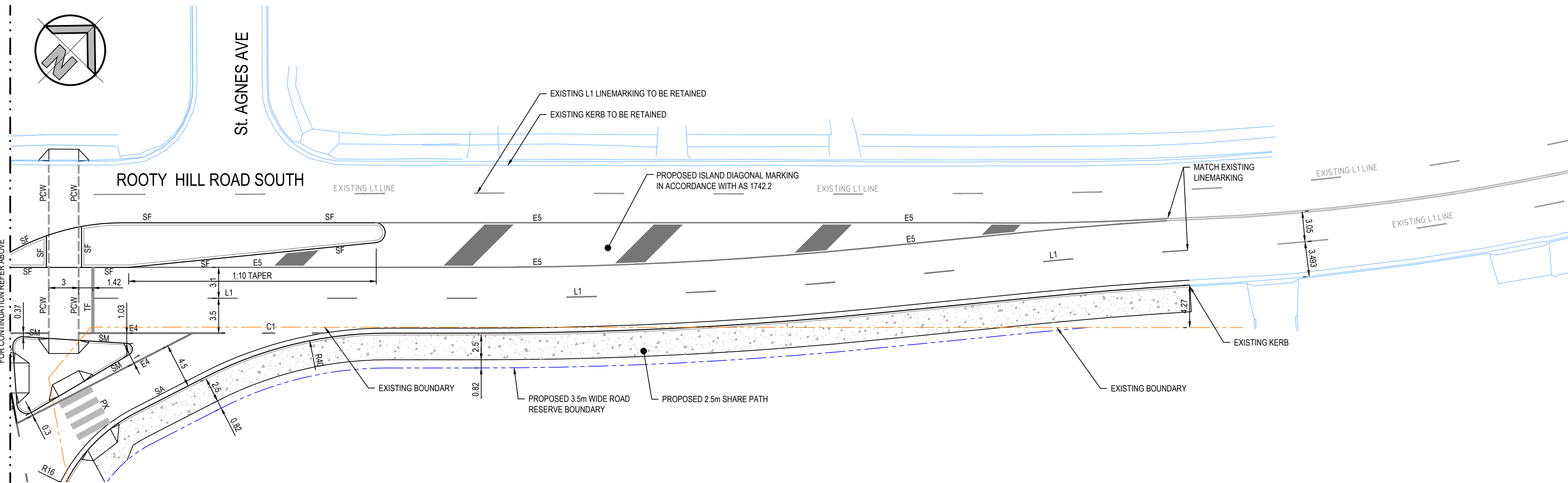
INTERSECTION LAYOUT - CONCEPT LINEMARKING PLAN SCALE: 1:250 @A1
