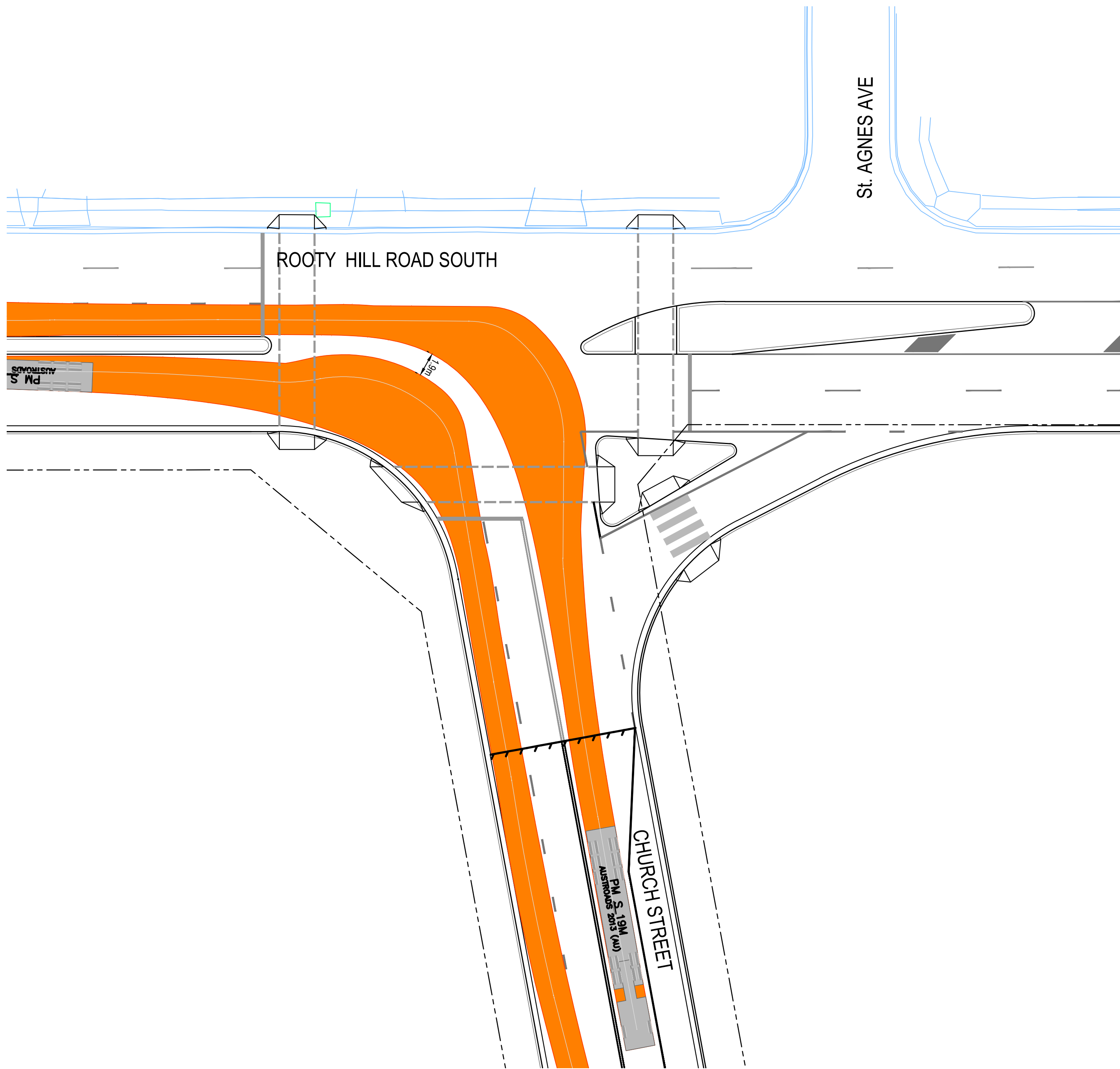
INTERSECTION LAYOUT - TURNING PATHS SCALE: 1:250@A1
