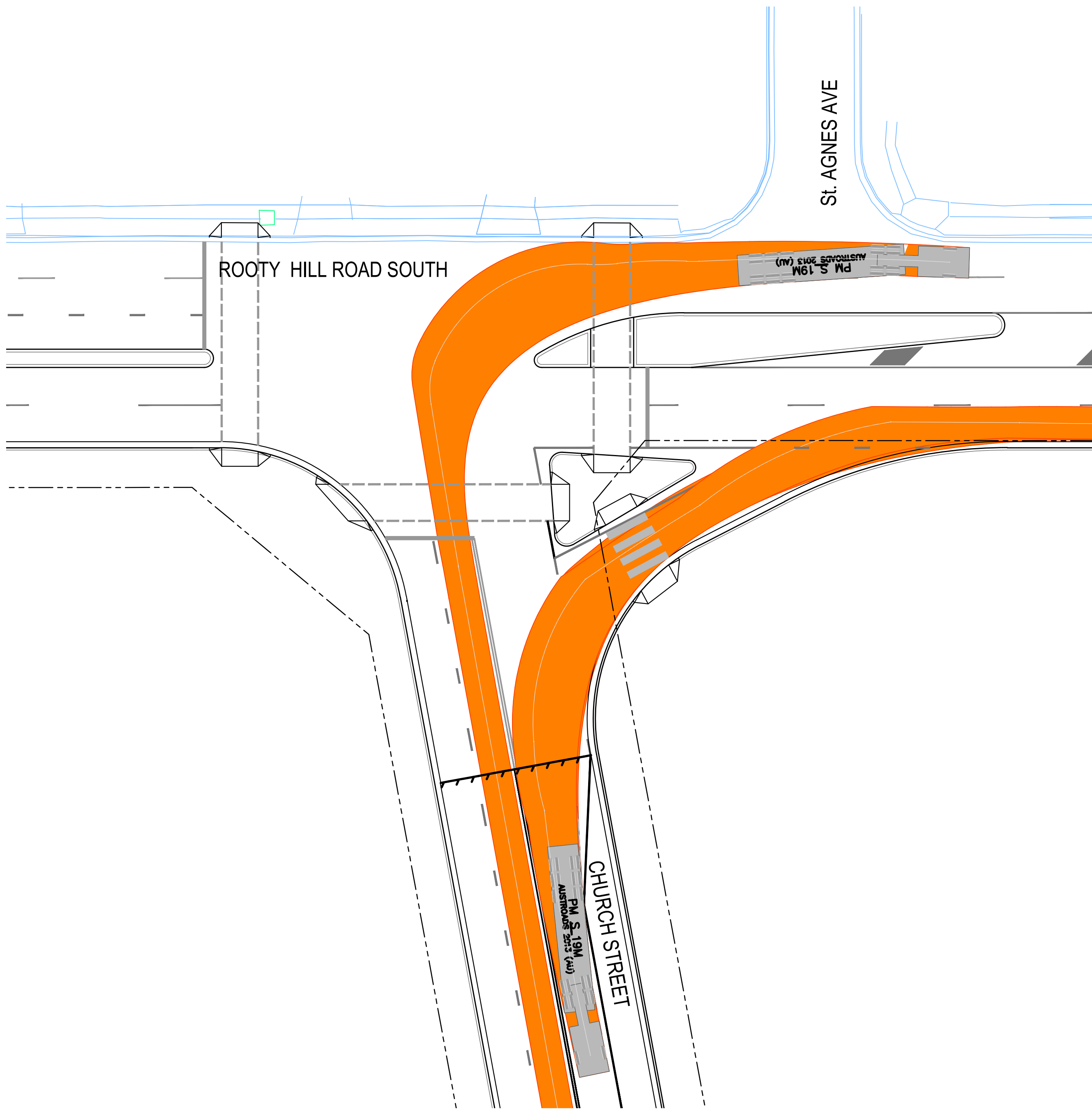
INTERSECTION LAYOUT - TURNING PATHS SCALE: 1:250@A1
